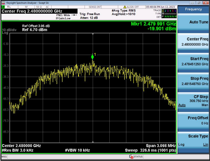
Power Spectral Density_NVNT_ANT1_2Mbps_2480
