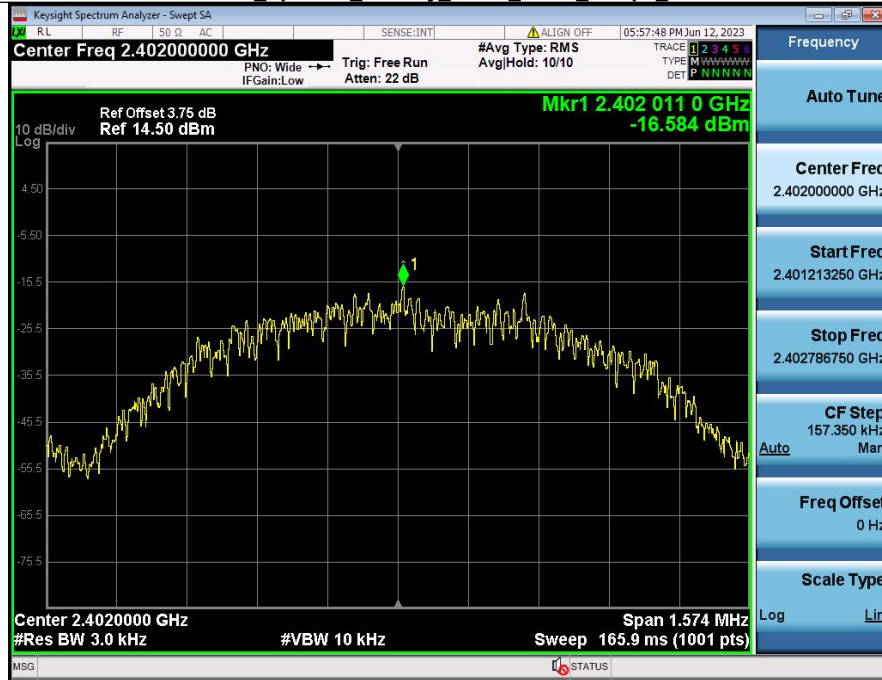
Power_Spectral_Density_NVNT_ANT1_1Mbps_2402
