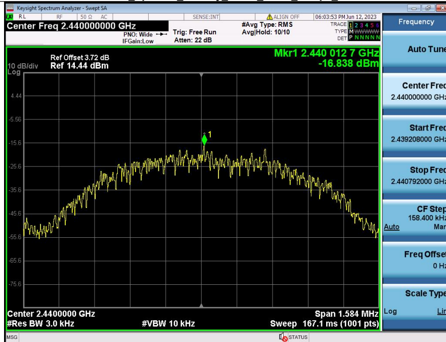
Power_Spectral_Density_NVNT_ANT1_1Mbps_2440
