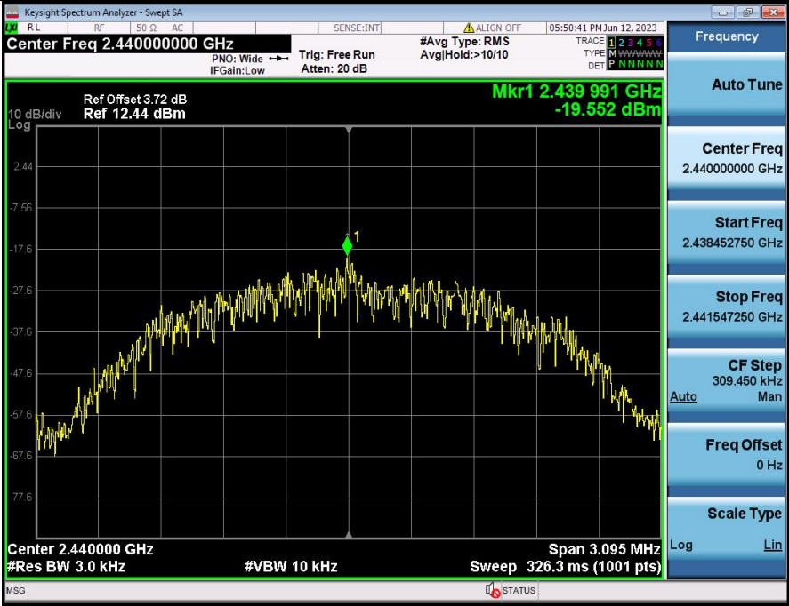
Power Spectral Density_NVNT_ANT1_2Mbps_2440
