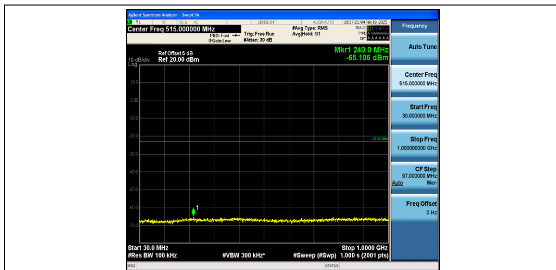
Band2_15MHz_16QAM_18675_1RB#0_30~1000_30~1000
