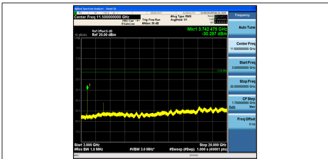
Band2_20MHz_16QAM_18900_1RB#0_3000~20000_3000~20000
