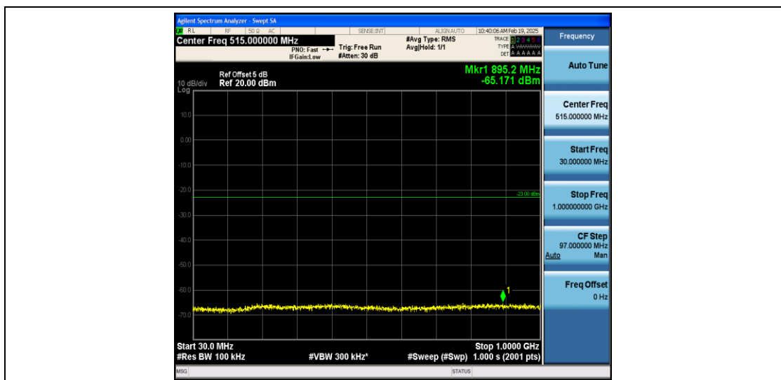
Band2_15MHz_QPSK_19125_1RB#0_30~1000_30~1000
