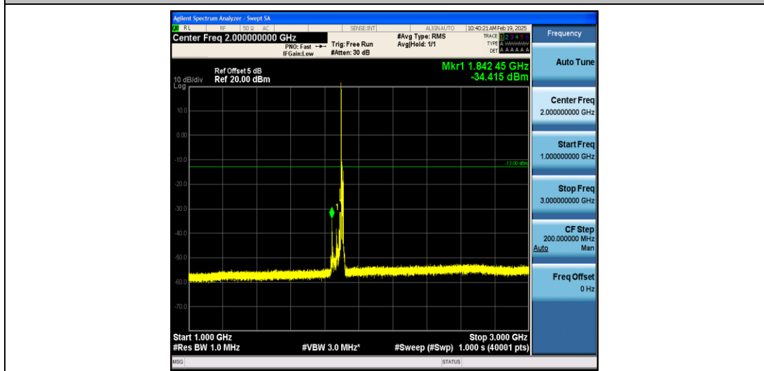
Band2_15MHz_QPSK_19125_1RB#0_1000~3000_1000~3000
