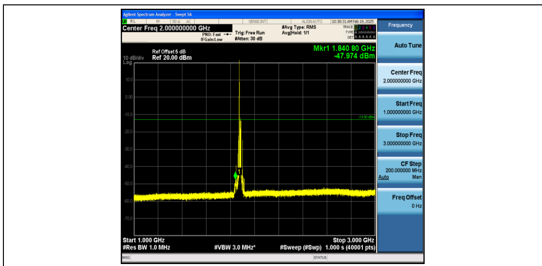
Band2_15MHz_QPSK_18900_1RB#0_1000~3000_1000~3000
