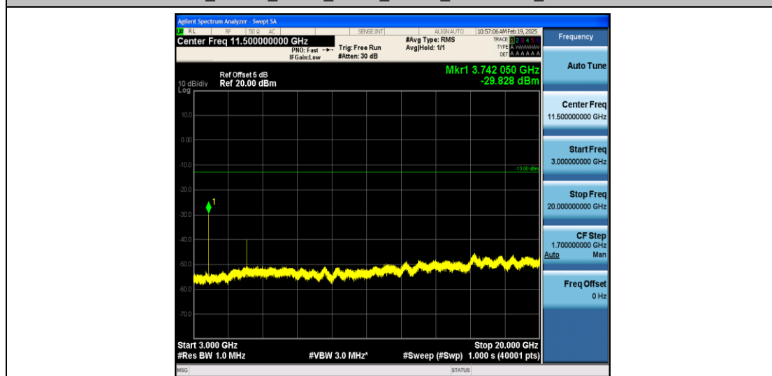
Band2_20MHz_QPSK_18900_1RB#0_3000~20000_3000~20000
