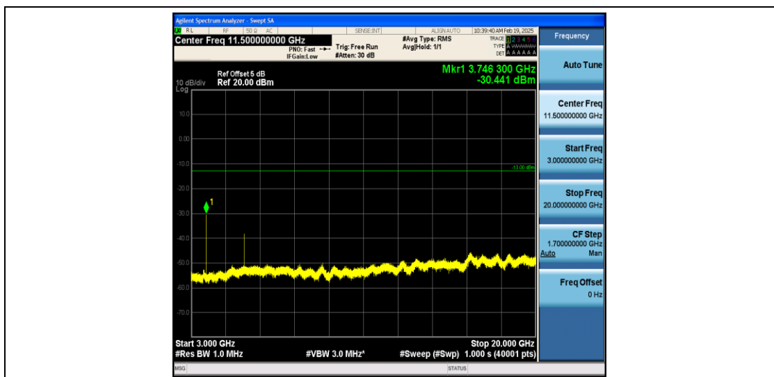
Band2_15MHz_16QAM_18900_1RB#0_3000~20000_3000~20000
