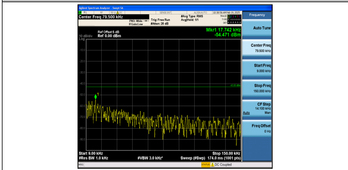
Band2_15MHz_16QAM_18900_1RB#0_0.009~0.15_0.009~0.15
