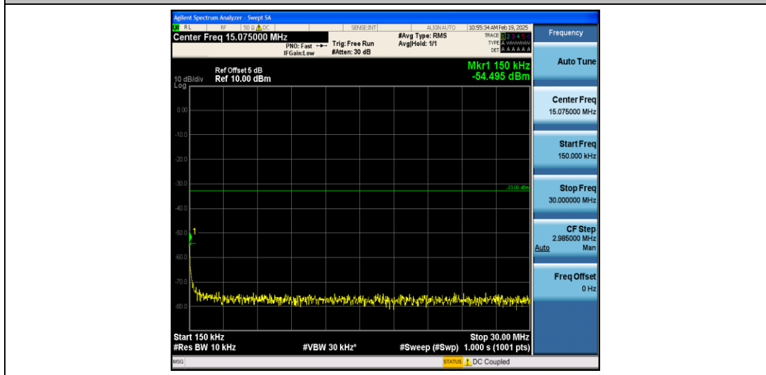
Band2_20MHz_16QAM_18700_1RB#0_0.15~30_0.15~30
