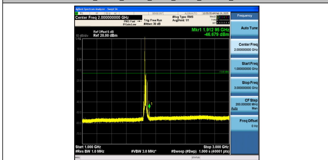
Band2_20MHz_16QAM_18700_1RB#0_1000~3000_1000~3000
