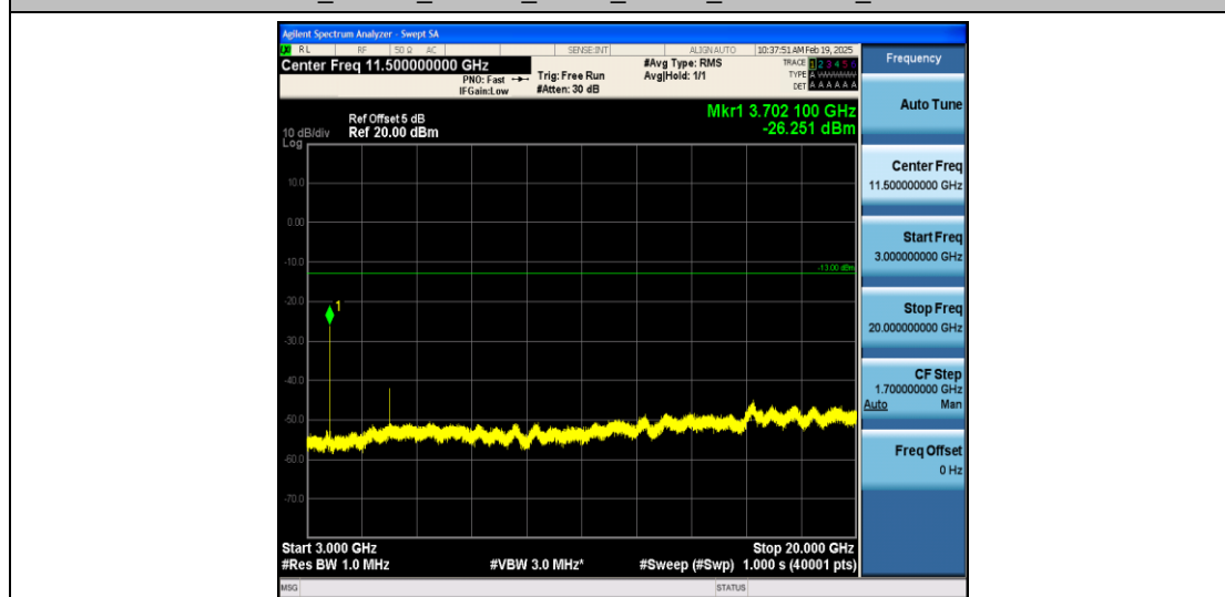
Band2_15MHz_16QAM_18675_1RB#0_3000~20000_3000~20000
