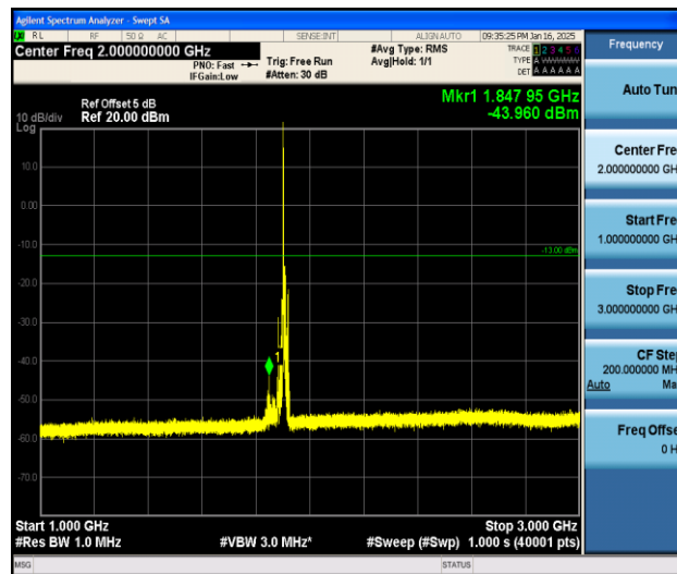
Band2_10MHz_16QAM_19150_1RB#0_1000~3000_1000~3000
