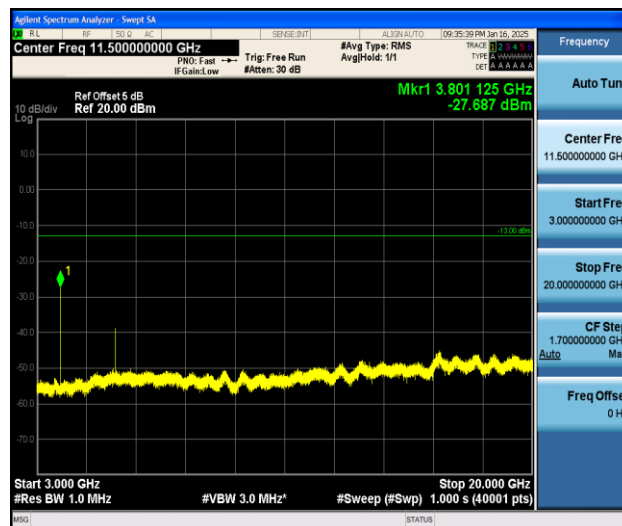
Band2_10MHz_16QAM_19150_1RB#0_3000~20000_3000~20000
