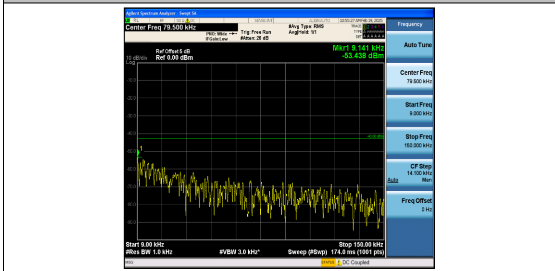
Band2_20MHz_16QAM_18700_1RB#0_0.009~0.15_0.009~0.15
