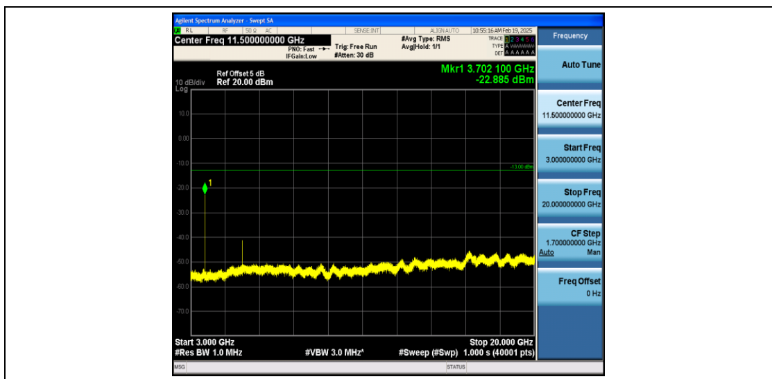
Band2_20MHz_QPSK_18700_1RB#0_3000~20000_3000~20000
