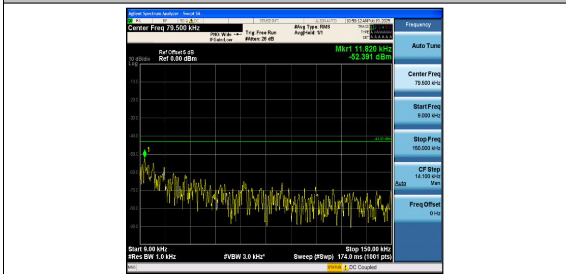
Band2_20MHz_QPSK_19100_1RB#0_0.009~0.15_0.009~0.15
