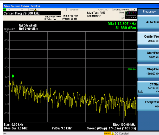
Band2_15MHz_QPSK_18675_1RB#0_0.009~0.15_0.009~0.15
