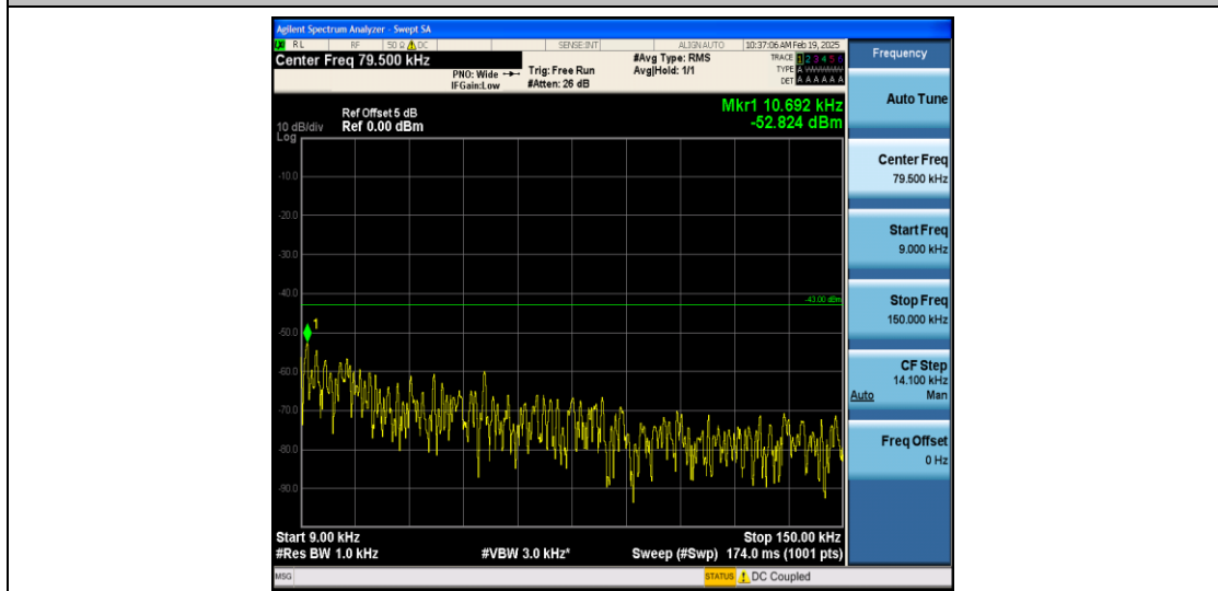
Band2_15MHz_16QAM_18675_1RB#0_0.009~0.15_0.009~0.15
