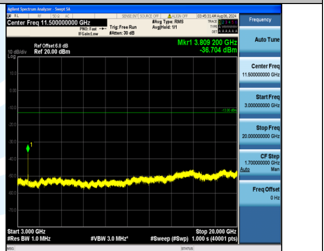
Band2_10MHz_16QAM_19150_50RB#0_3000~20000_3000~20000
