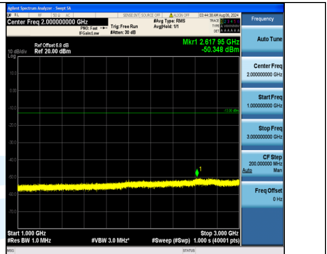
Band2_10MHz_16QAM_19150_1RB#49_1000~3000_1000~3000
