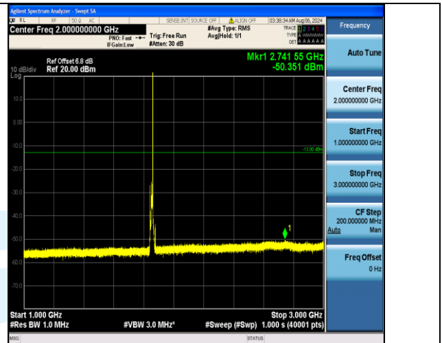
Band2_10MHz_16QAM_18650_1RB#49_1000~3000_1000~3000
