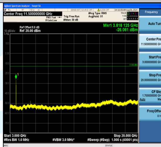
Band2_15MHz_QPSK_19125_1RB#74_3000~20000_3000~20000
