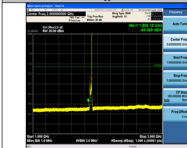
Band2_15MHz_QPSK_19125_1RB#74_1000~3000_1000~3000
