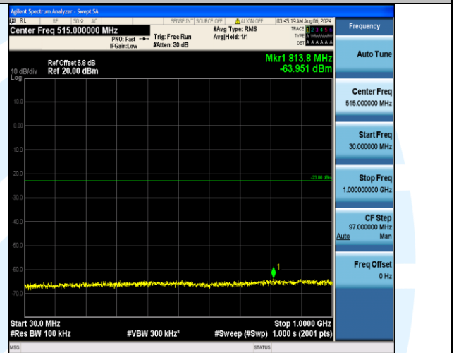
Band2_10MHz_16QAM_19150_50RB#0_30~1000_30~1000
