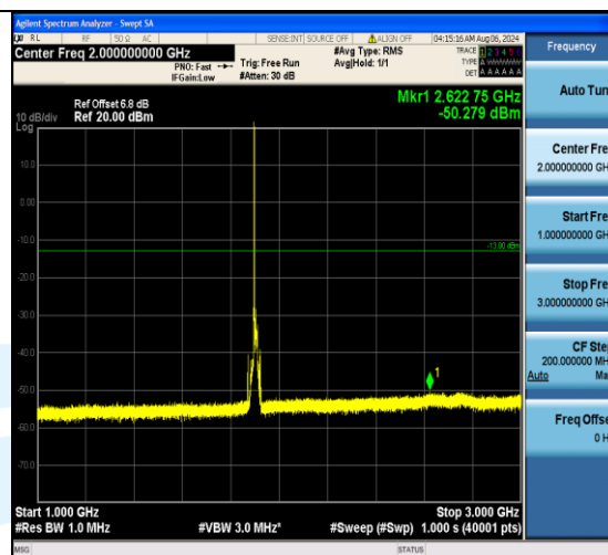
Band2_15MHz_QPSK_19125_1RB#0_1000~3000_1000~3000
