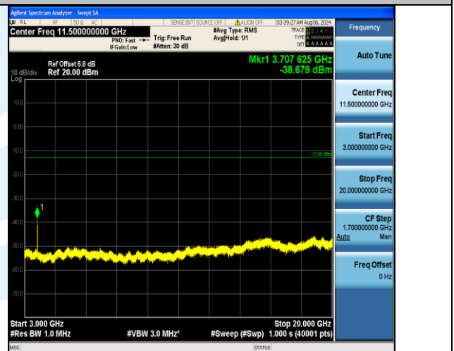
Band2_10MHz_16QAM_18650_50RB#0_3000~20000_3000~20000
