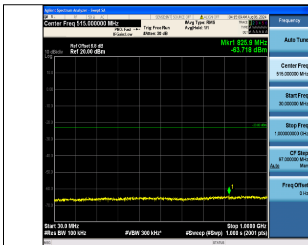
Band2_15MHz_QPSK_19125_1RB#0_30~1000_30~1000
