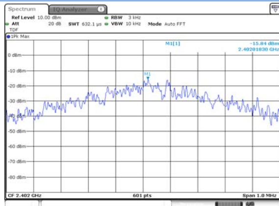
GFSK (BLE) LOW CHANNEL
