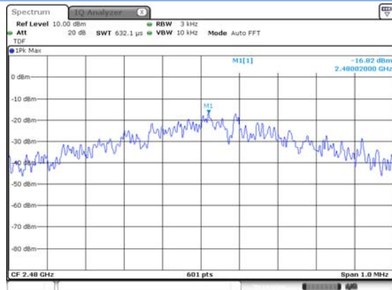
GFSK (BLE) HIGH CHANNEL
