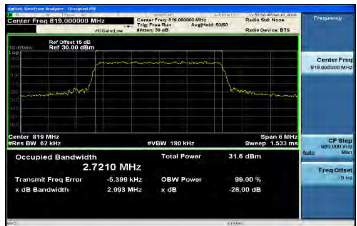
Part 90_Band26_3MHz_QPSK_15_0_HighCH26775
