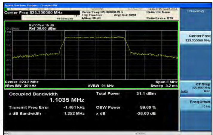
Part 90_Band26_1_4MHz_16QAM_6_0_HighCH26783
