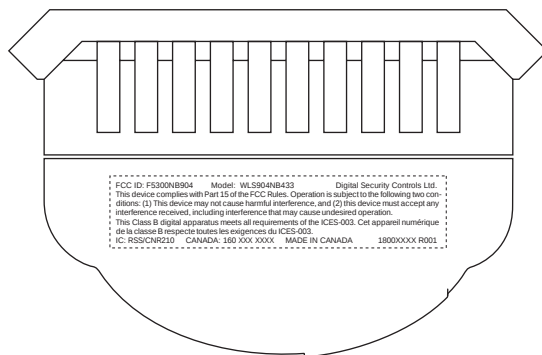
TOP OF THE UNIT SHOWING PLACEMENT OF LABEL (ACTUAL SIZE) (THE UNIT SHOWN ATTACHED TO MOUNTING BRACKET)
