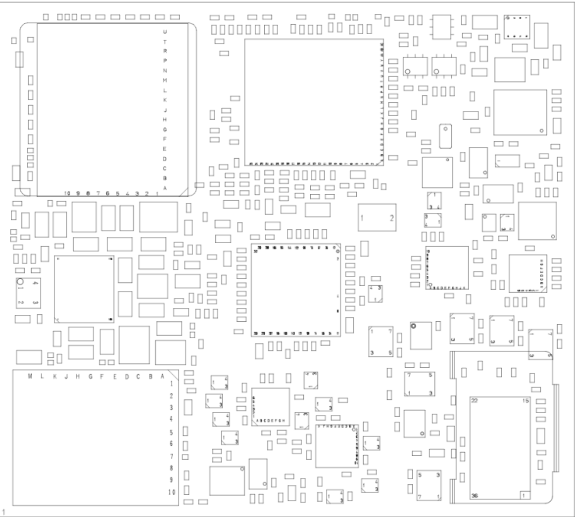
Figure 1: Floorplan ALAS5-AM
