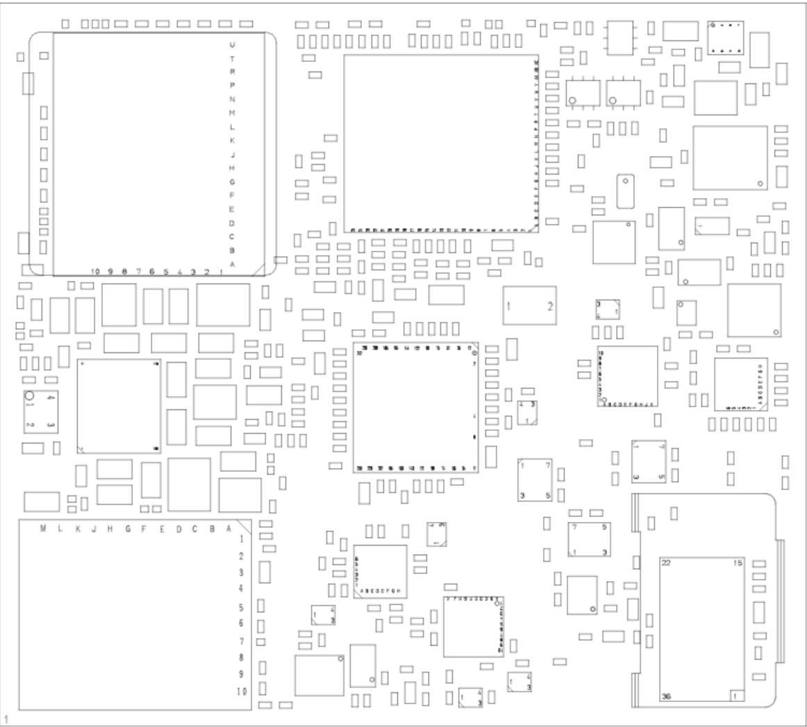
Figure 2: Floorplan ALAS5V-US
