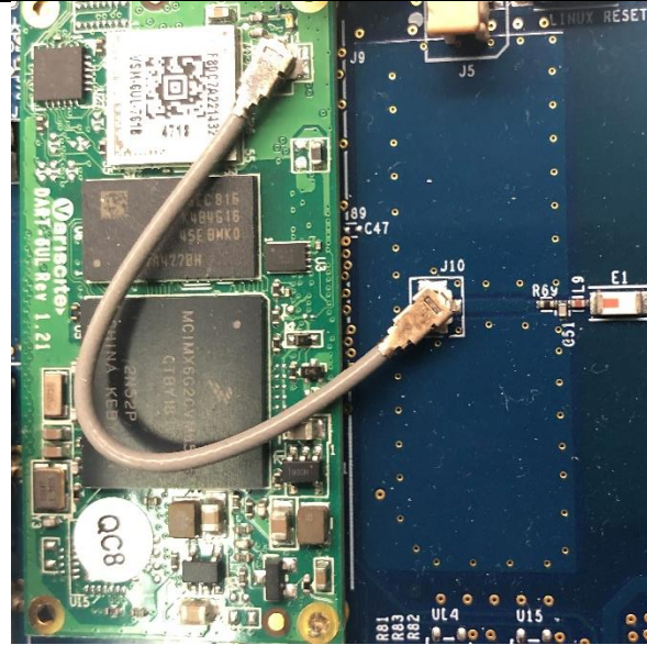
On-board Antenna print component side
