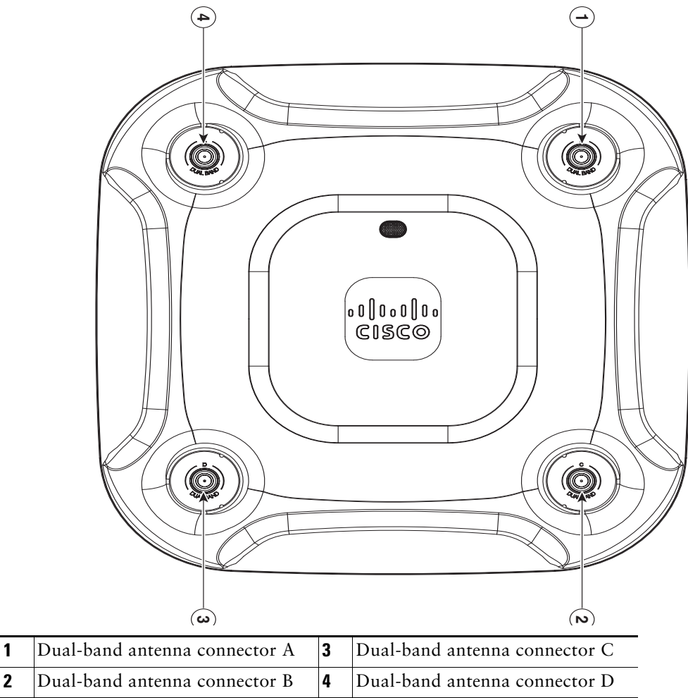
Figure 1 Access Point Ports and Connections (top)—3702E Model
