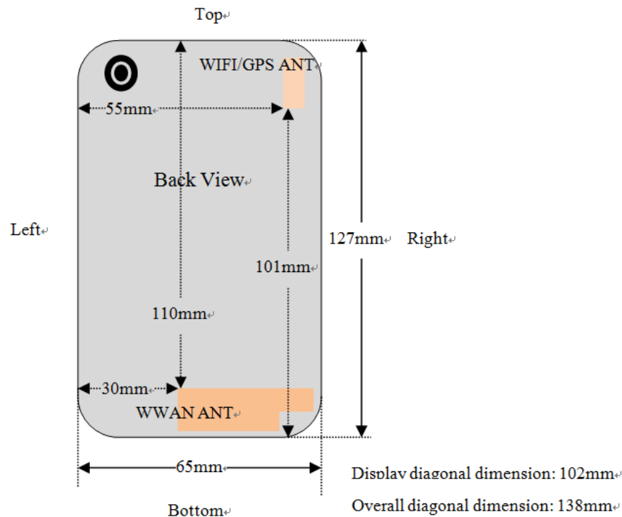
Fig.14.1 EUT Antenna Locations
