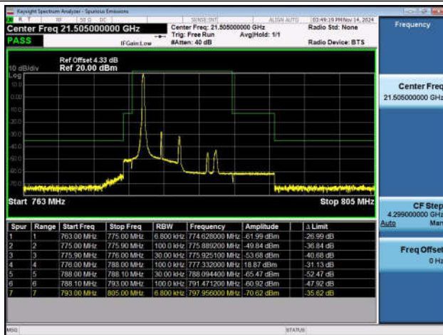
Band13_5MHz_QPSK_23255_1RB#24
