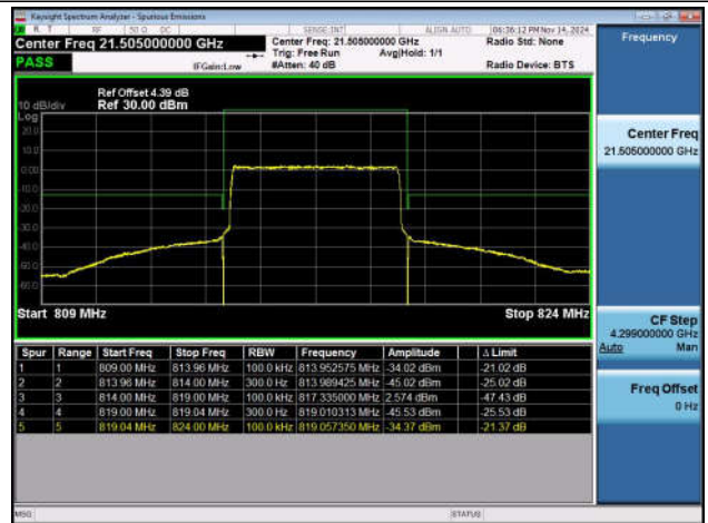
Band26_5MHz_QPSK_26715_25RB#0
