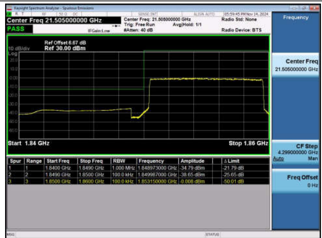
Band25_10MHz_QPSK_26640_50RB#0
