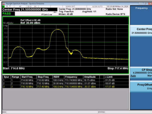
Band12_1.4MHz_QPSK_23173_1RB#5
