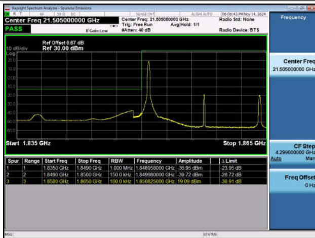
Band25_15MHz_QPSK_26615_1RB#74
