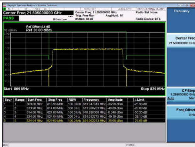
Band26_10MHz_QPSK_26740_50RB#0
