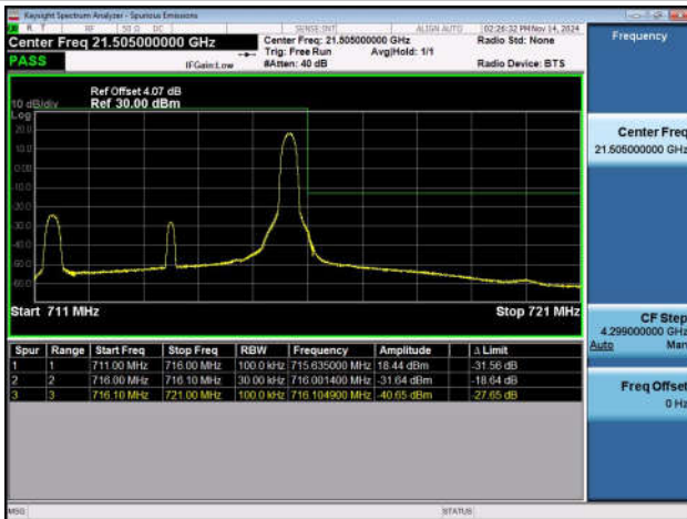
Band12_10MHz_QPSK_23060_1RB#0
