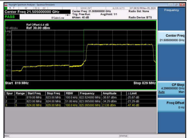
Band5_5MHz_QPSK_20625_25RB#0
