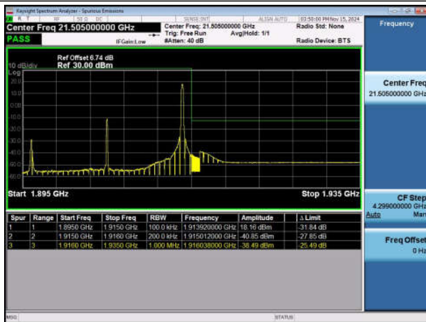
Band26_1.4MHz_QPSK_26697_1RB#0
