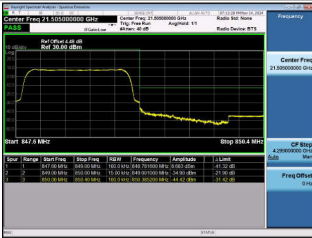
Band26_3MHz_QPSK_26805_15RB#0
