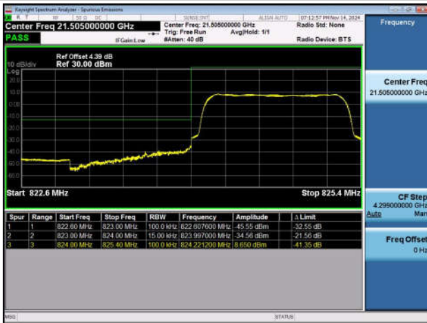
Band26_1.4MHz_QPSK_27033_6RB#0
