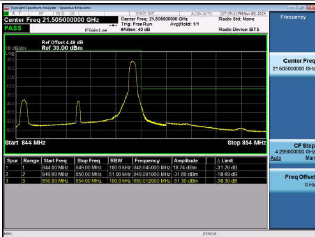
Band5_5MHz_QPSK_20625_1RB#24
