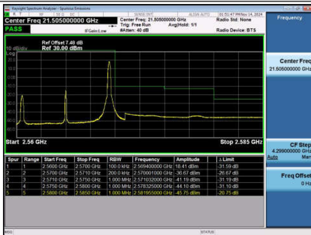
Band7_10MHz_QPSK_21400_1RB#49
