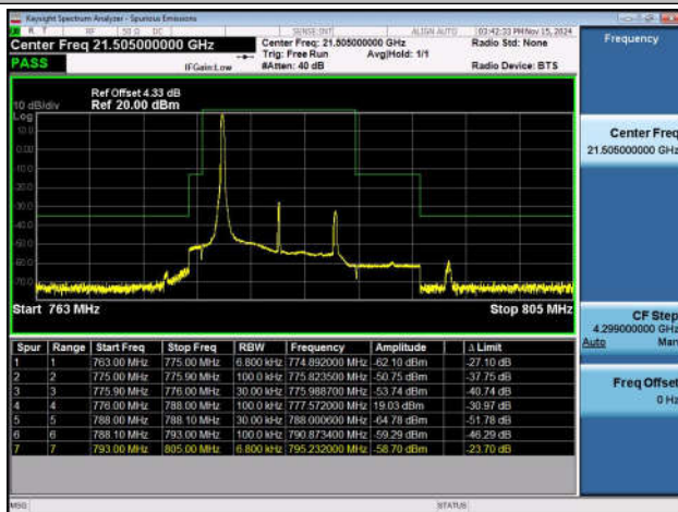
Band13_10MHz_QPSK_23230_1RB#0
