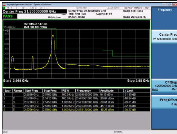
Band7_10MHz_QPSK_20800_1RB#0
