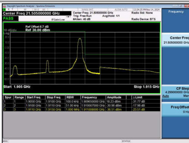
Band2_5MHz_QPSK_19175_1RB#24
