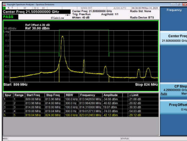
Band26_5MHz_QPSK_26715_1RB#0
