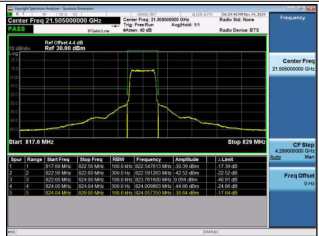
Band26_1.4MHz_QPSK_26783_6RB#0
