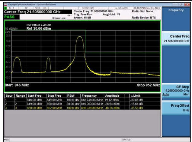
Band26_3MHz_QPSK_27025_1RB#14
