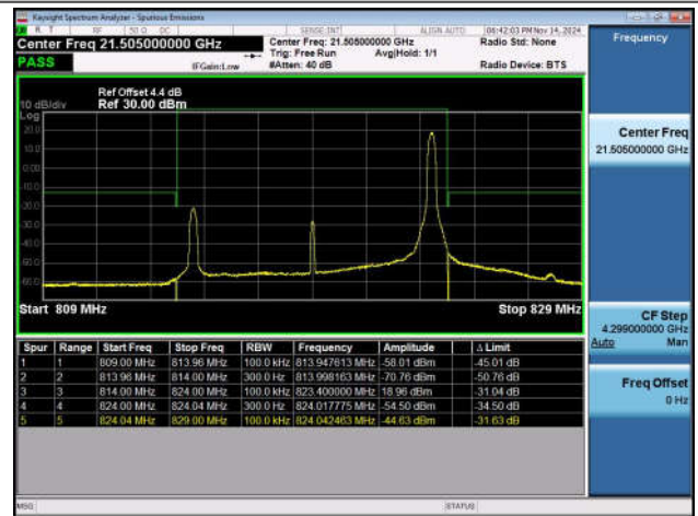
Band26_1.4MHz_QPSK_26797_1RB#0
