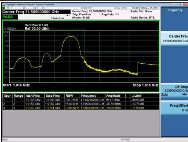
Band25_1.4MHz_QPSK_26683_1RB#5
