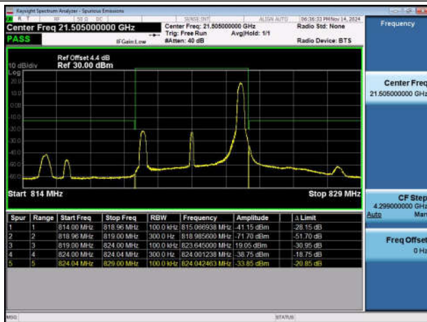
Band26_10MHz_QPSK_26740_1RB#0
