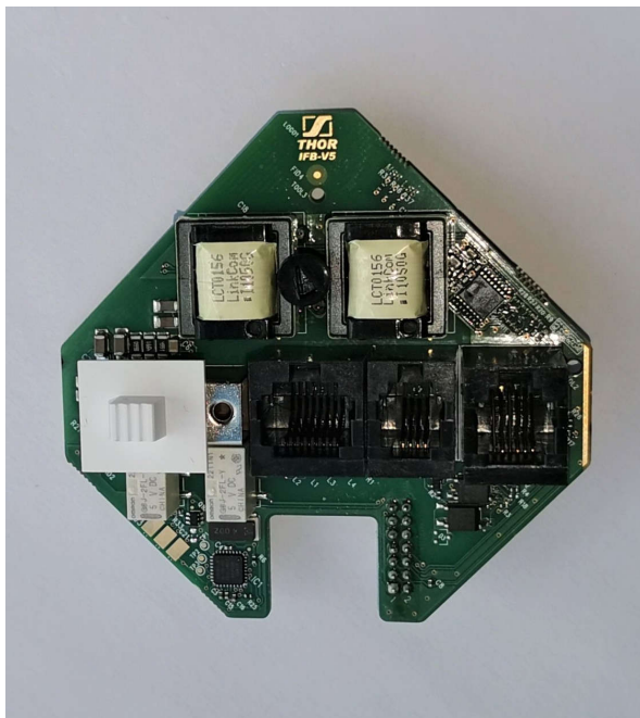
SCDB9 Interface Board
