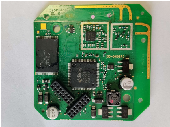
Main PCB without shielding
