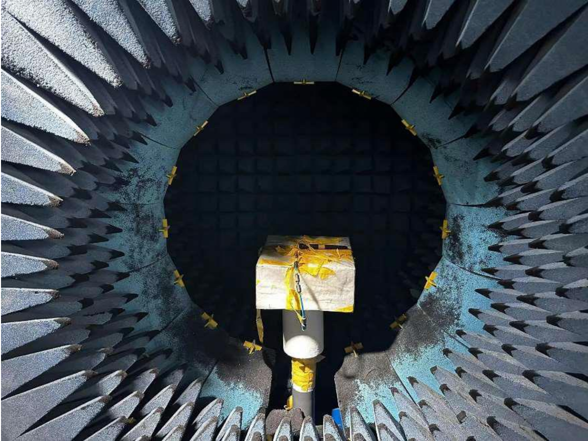
Antenna setup photo
