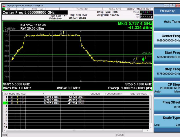
11AX80MIMO-Ant0-5610-PASS
