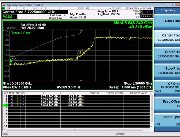
11AC80MIMO-Ant0-5775-PASS
