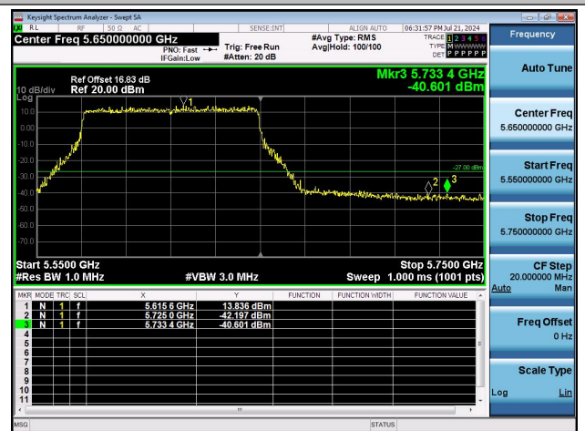
11AX80MIMO-Ant1-5610-PASS
