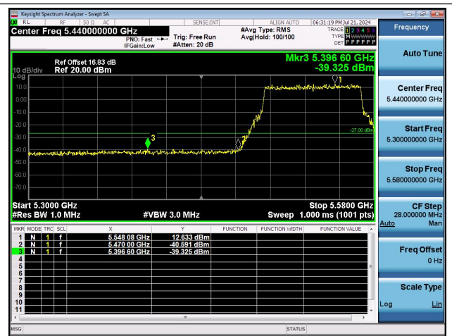
11AX80MIMO-Ant1-5530-PASS
