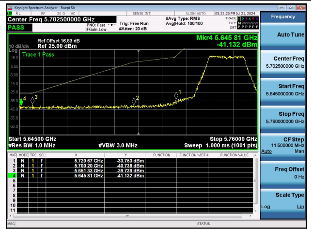
11N20MIMO-Ant1-5745-PASS
