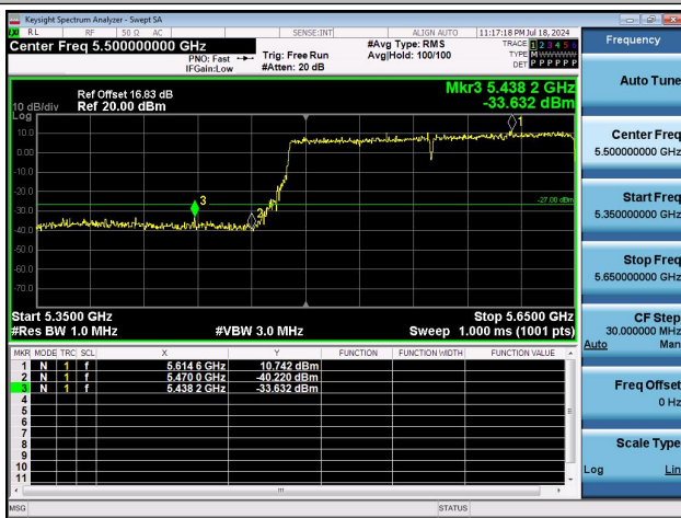
11AX160MIMO-Ant0-5570-PASS
