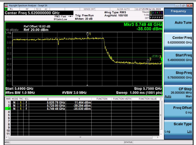
11AX160MIMO-Ant0-5570-PASS
