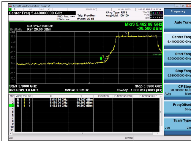
11AX80MIMO-Ant0-5530-PASS
