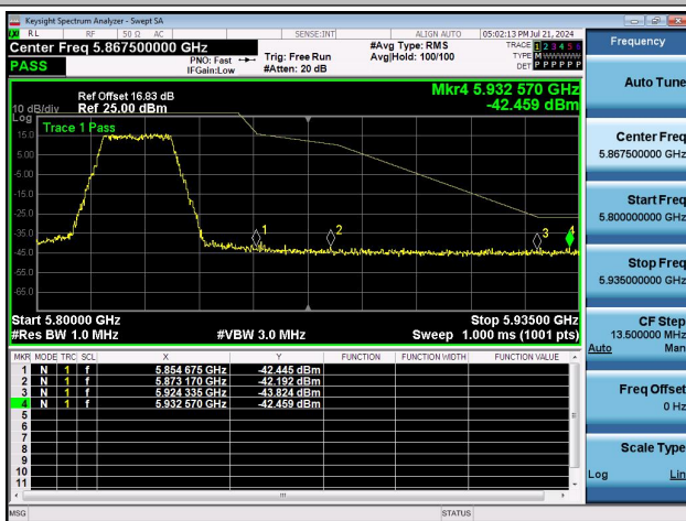
11AC20MIMO-Ant0-5825-PASS
