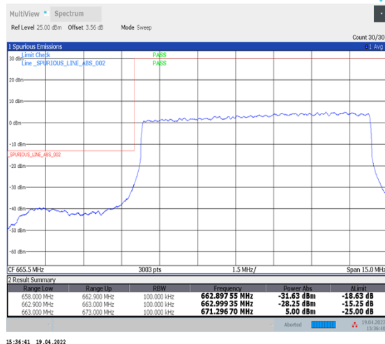
1-N71--15-10-L-3-DFT-PI2BPSK-Outer_Full-50@0-Ant1-PASS-see graph
