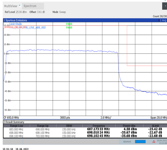
1-N71--15-15-H-3-DFT-PI2BPSK-Outer_Full-75@0-Ant1-PASS-see graph
