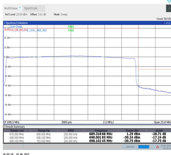
1-N71--15-20-H-6-CP-QPSK-Outer_Full-106@0-Ant1-PASS-see graph
