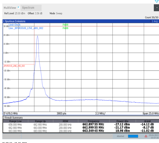
1-N71--15-20-L-4-CP-QPSK-Edge_1RB_Left-1@0-Ant1-PASS-see graph
