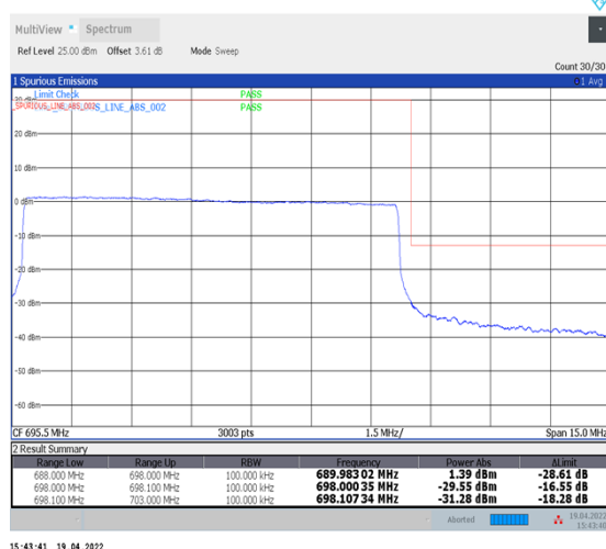
1-N71--15-10-H-6-CP-QPSK-Outer_Full-52@0-Ant1-PASS-see graph
