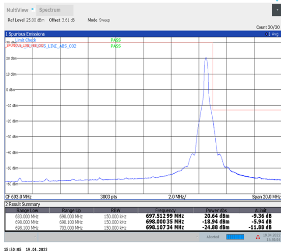
1-N71--15-15-H-2-DFT-PI2BPSK-Edge_1RB_Right-1@78-Ant1-PASS-see graph
