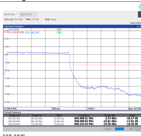
1-N71--15-5-H-3-DFT-PI2BPSK-Outer_Full-25@0-Ant1-PASS-see graph
