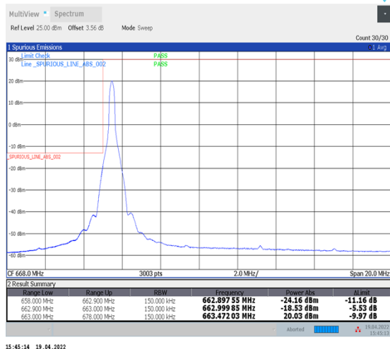
1-N71--15-15-L-1-DFT-PI2BPSK-Edge_1RB_Left-1@0-Ant1-PASS-see graph
