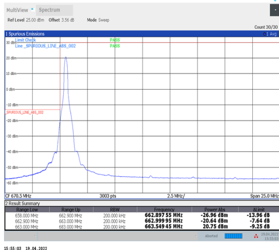
1-N71--15-20-L-1-DFT-PI2BPSK-Edge_1RB_Left-1@0-Ant1-PASS-see graph
