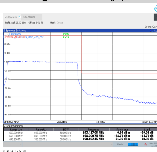
1-N71--15-5-H-6-CP-QPSK-Outer_Full-25@0-Ant1-PASS-see graph
