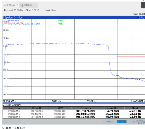
1-N71--15-20-H-3-DFT-PI2BPSK-Outer_Full-100@0-Ant1-PASS-see graph
