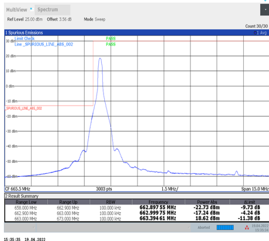
1-N71--15-10-L-1-DFT-PI2BPSK-Edge_1RB_Left-1@0-Ant1-PASS-see graph
