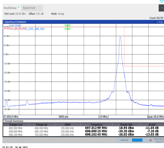
1-N71--15-15-H-5-CP-QPSK-Edge_1RB_Right-1@78-Ant1-PASS-see graph
