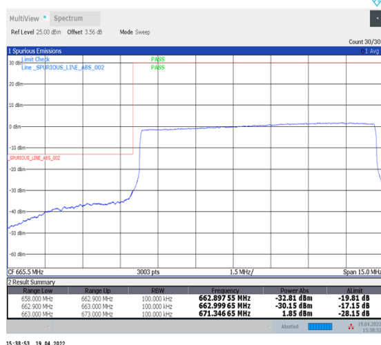
1-N71--15-10-L-6-CP-QPSK-Outer_Full-52@0-Ant1-PASS-see graph
