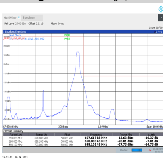
1-N71--15-5-H-5-CP-QPSK-Edge_1RB_Right-1@24-Ant1-PASS-see graph
