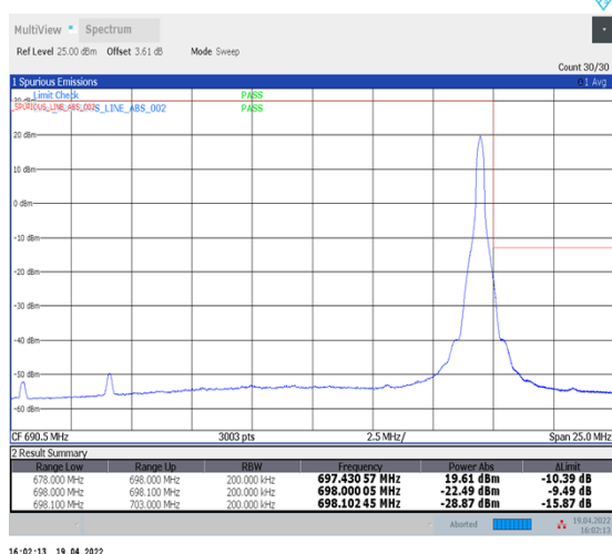
1-N71--15-20-H-5-CP-QPSK-Edge_1RB_Right-1@105-Ant1-PASS-see graph
