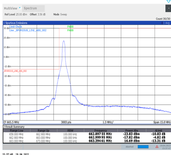
1-N71--15-10-L-4-CP-QPSK-Edge_1RB_Left-1@0-Ant1-PASS-see graph
