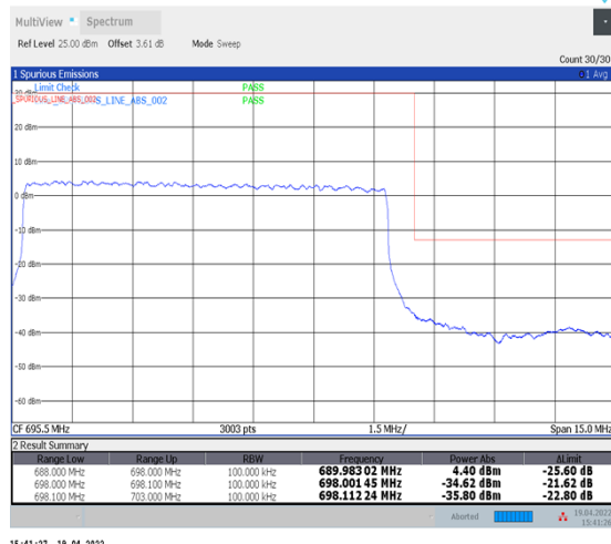
1-N71--15-10-H-3-DFT-PI2BPSK-Outer_Full-50@0-Ant1-PASS-see graph
