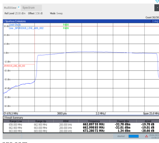
1-N71--15-20-L-6-CP-QPSK-Outer_Full-106@0-Ant1-PASS-see graph
