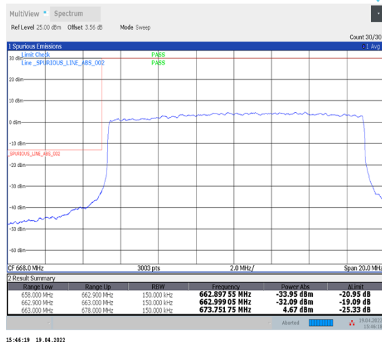
1-N71--15-15-L-3-DFT-PI2BPSK-Outer_Full-75@0-Ant1-PASS-see graph
