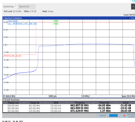
1-N71--15-15-L-6-CP-QPSK-Outer_Full-79@0-Ant1-PASS-see graph
