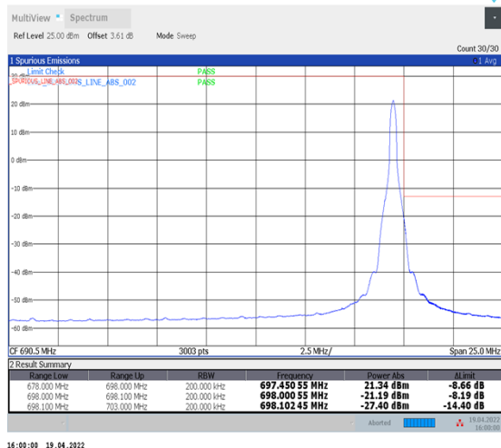
1-N71--15-20-H-2-DFT-PI2BPSK-Edge_1RB_Right-1@105-Ant1-PASS-see graph
