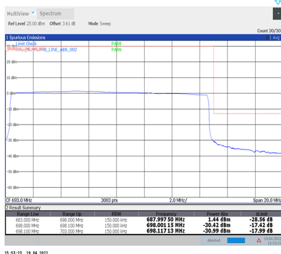
1-N71--15-15-H-6-CP-QPSK-Outer_Full-79@0-Ant1-PASS-see graph
