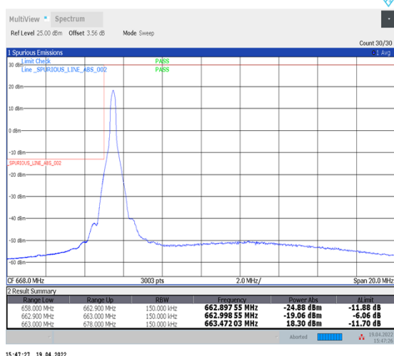
1-N71--15-15-L-4-CP-QPSK-Edge_1RB_Left-1@0-Ant1-PASS-see graph
