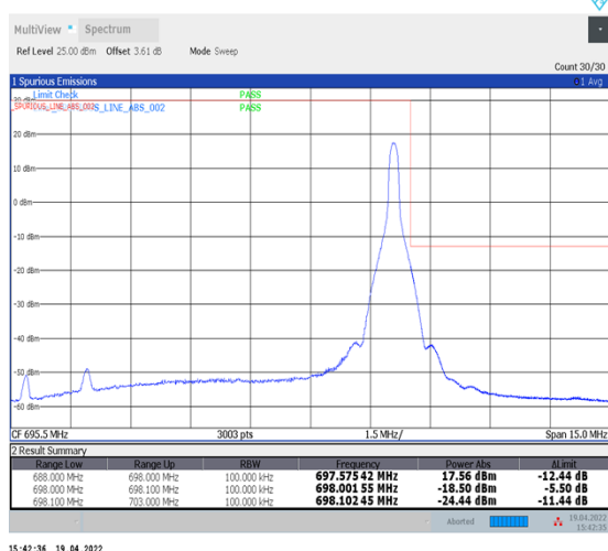
1-N71--15-10-H-5-CP-QPSK-Edge_1RB_Right-1@51-Ant1-PASS-see graph
