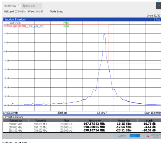
1-N71--15-10-H-2-DFT-PI2BPSK-Edge_1RB_Right-1@51-Ant1-PASS-see graph
