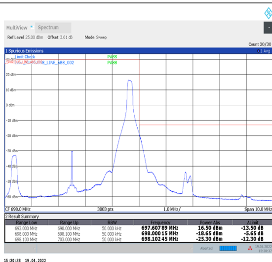
1-N71--15-5-H-2-DFT-PI2BPSK-Edge_1RB_Right-1@24-Ant1-PASS-see graph
