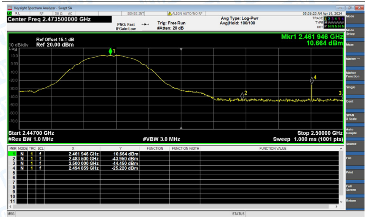
Restrict Band NVNT b 2462MHz Ant1 Average
