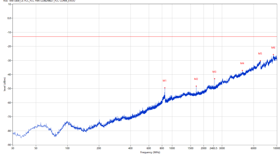
RSE Test case_FCC_FCC PART22824&27_FCC CDMA_EVDO
