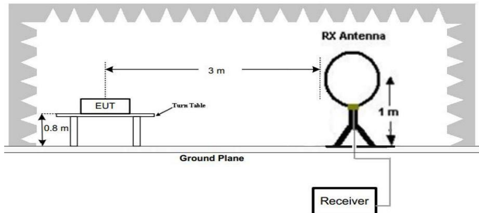
Figure 1. Below 30MHz
