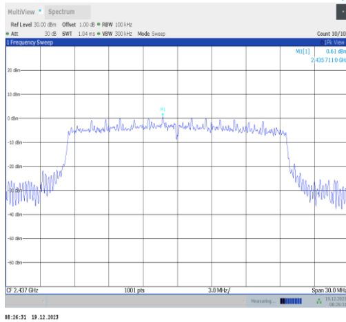
11ax20MIMO-Ant2-2437-0~Reference-PASS
