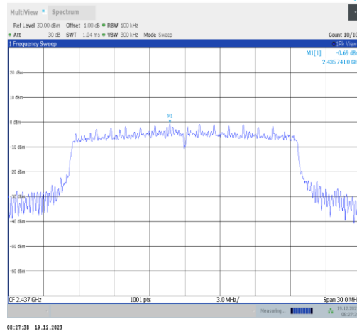
11ax20MIMO-Ant3-2437-0~Reference-PASS
