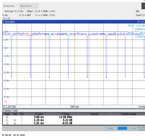
NTNV-11n40SISO-Ant2-2422
