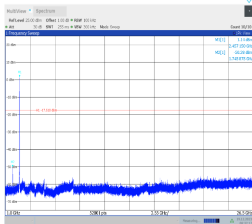
11ax20MIMO-Ant1-2462-1000~26500-PASS
