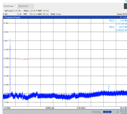
11ax40MIMO-Ant3-2437-1000~26500-PASS
