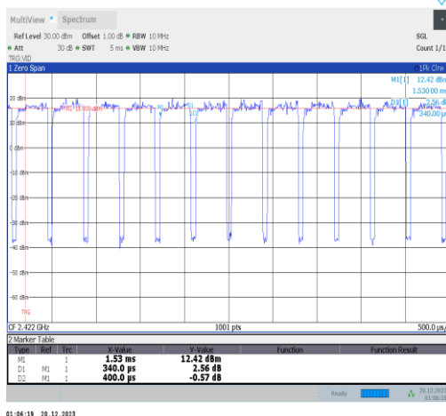
NTNV-11ax40MIMO-Ant2-2422
