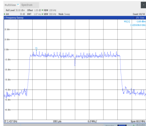
11ax40MIMO-Ant1-2437-0~Reference-PASS
