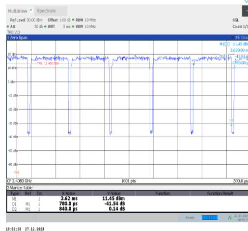
NTVN-11ax20MIMO-Ant2-2412-106Tone-RU53
