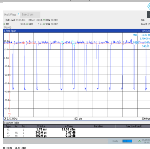
NTVN-11ax20MIMO-Ant3-2412
