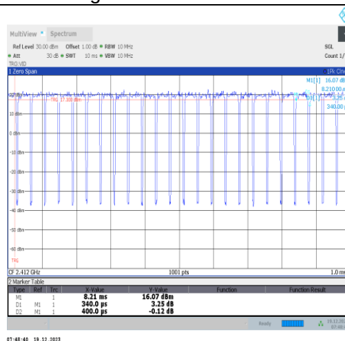
NTVN-11ax20MIMO-Ant1-2412
