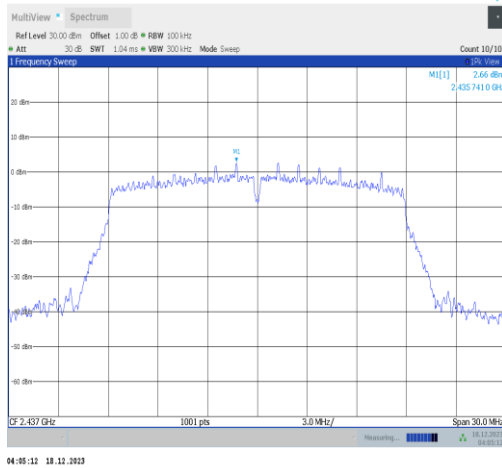
11n20SISO-Ant2-2437-0~Reference-PASS
