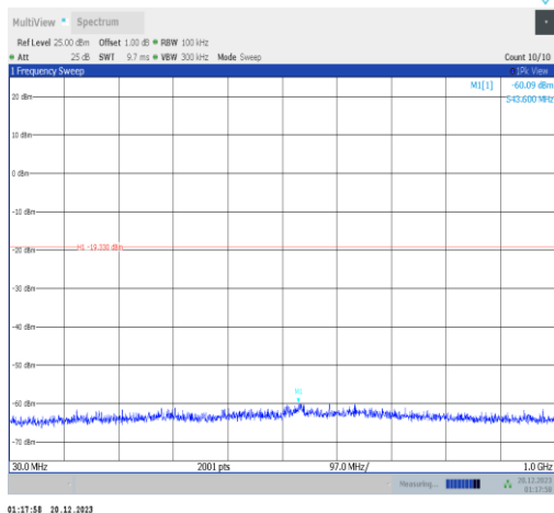
11ax40MIMO-Ant1-2452-30~1000-PASS
