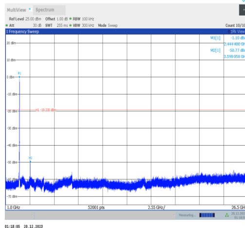
11ax40MIMO-Ant1-2452-1000~26500-PASS
