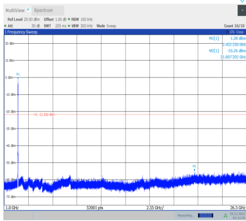
11ax40MIMO-Ant2-2437-1000~26500-PASS
