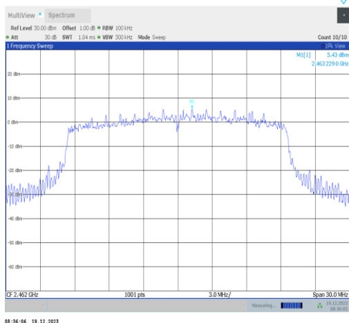
11ax20MIMO-Ant4-2462-0~Reference-PASS
