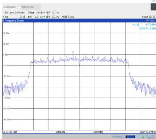
11ax20MIMO-Ant4-2437-0~Reference-PASS
