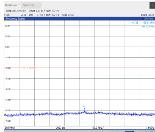
11ax40MIMO-Ant4-2422-30~1000-PASS
