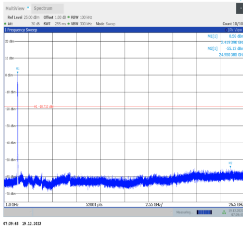
11n40SISO-Ant2-2422-1000~26500-PASS
