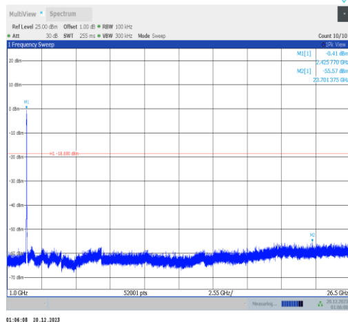
11ax40MIMO-Ant1-2422-1000~26500-PASS
