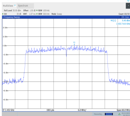
11ax40MIMO-Ant2-2452-0~Reference-PASS
