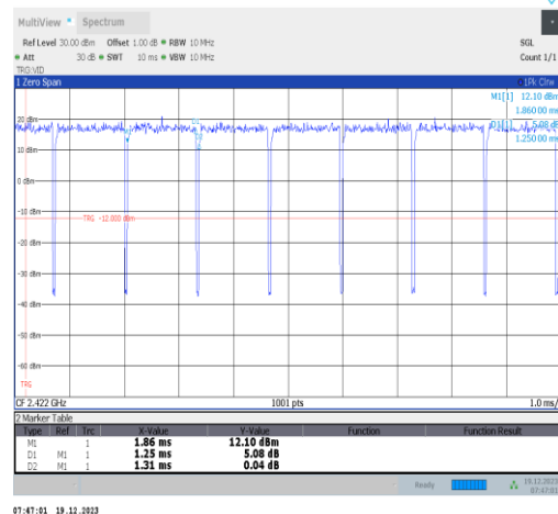
NTNV-11n40SISO-Ant3-2422
