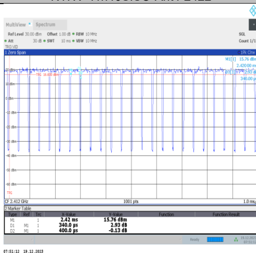
NTVN-11ax20MIMO-Ant2-2412
