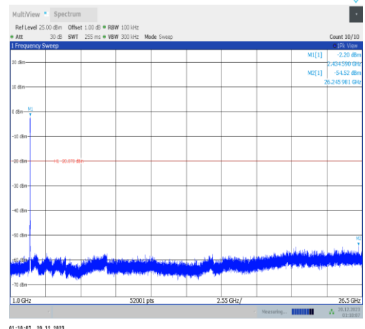
11ax40MIMO-Ant3-2422-1000~26500-PASS
