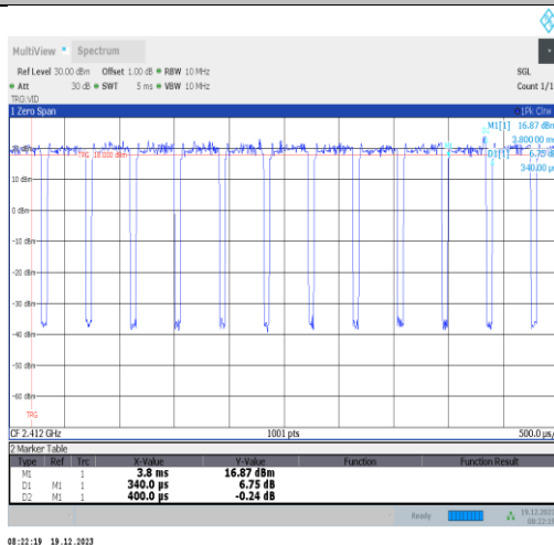
NTVN-11ax20MIMO-Ant4-2412
