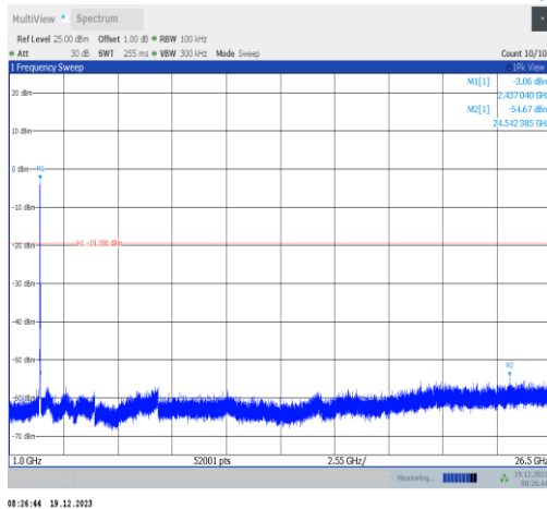
11ax20MIMO-Ant2-2437-1000~26500-PASS
