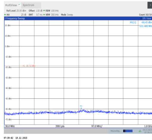
11n40SISO-Ant2-2422-30~1000-PASS
