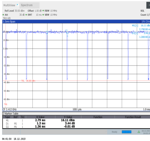
NTNV-11n20SISO-Ant2-2412
