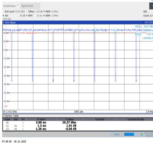
NTNV-11n20SISO-Ant4-2412
