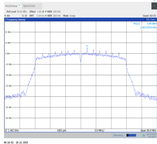
11n20SISO-Ant2-2462-0~Reference-PASS
