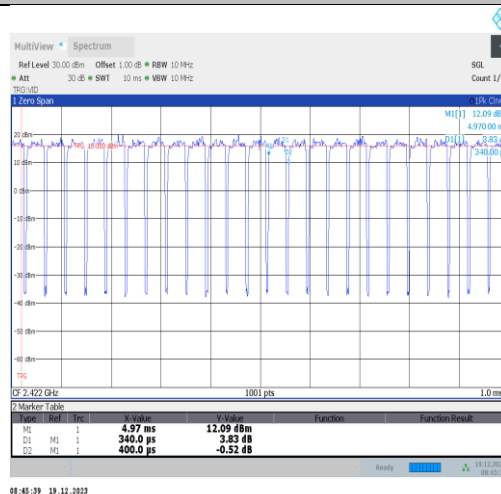
NTVN-11ax40MIMO-Ant1-2422
