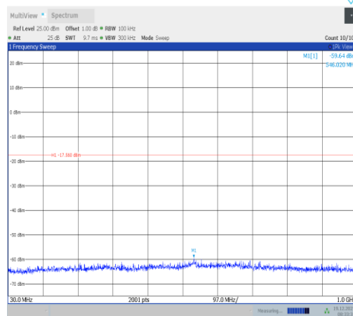
11ax20MIMO-Ant2-2462-30~1000-PASS
