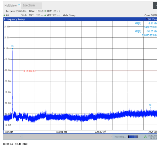
11ax20MIMO-Ant3-2437-1000~26500-PASS
