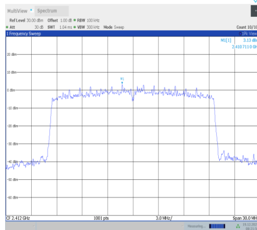
11ax20MIMO-Ant3-2412-0~Reference-PASS
