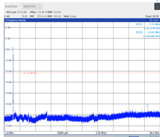
11ax40MIMO-Ant1-2437-1000~26500-PASS
