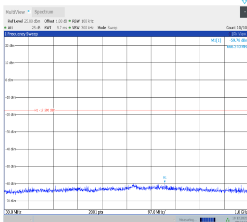
11ax20MIMO-Ant3-2462-30~1000-PASS
