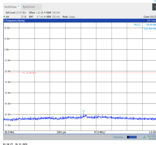
11ax40MIMO-Ant4-2437-30~1000-PASS
