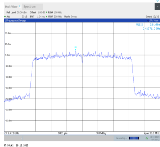
11ax20MIMO-Ant1-2412-0~Reference-PASS
