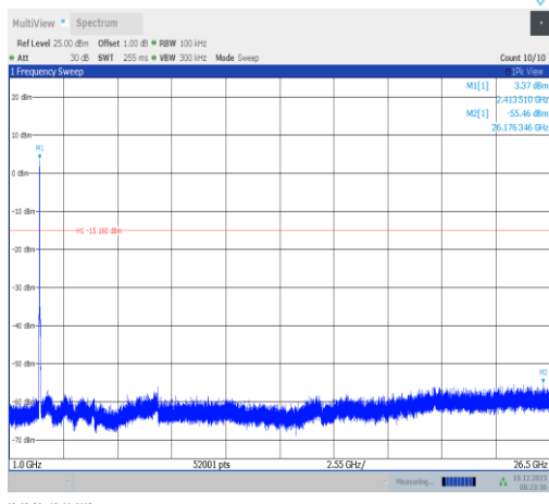
11ax20MIMO-Ant4-2412-1000~26500-PASS
