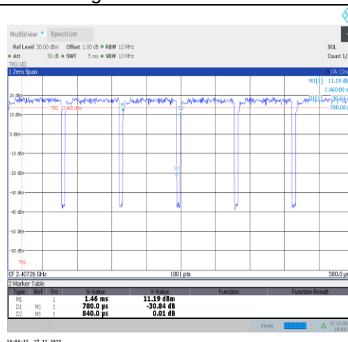
NTNV-11ax20MIMO-Ant4-2412-106Tone-RU53
