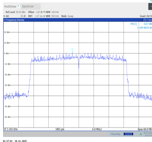
11ax40MIMO-Ant1-2452-0~Reference-PASS
