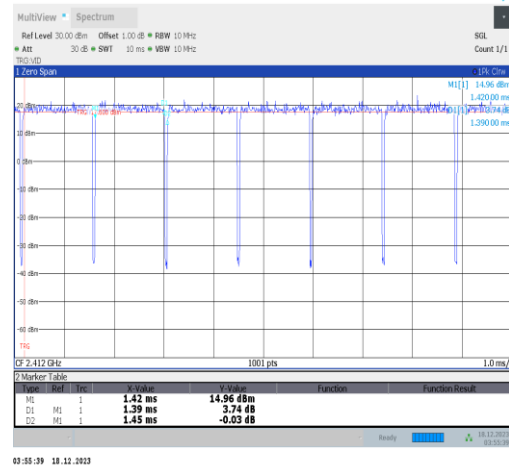
NTVN-11g-Ant1-2412
