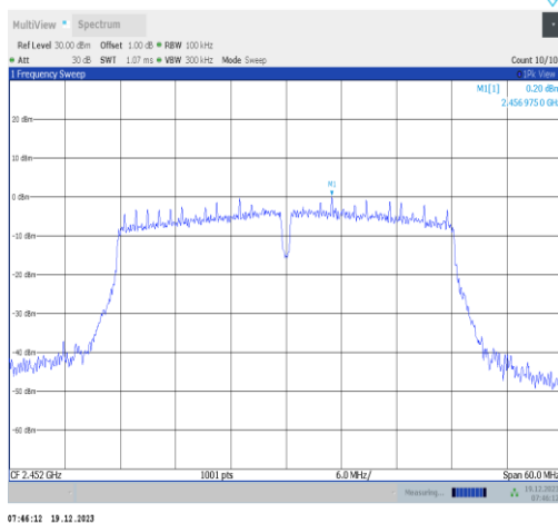
11n40SISO-Ant2-2452-0~Reference-PASS
