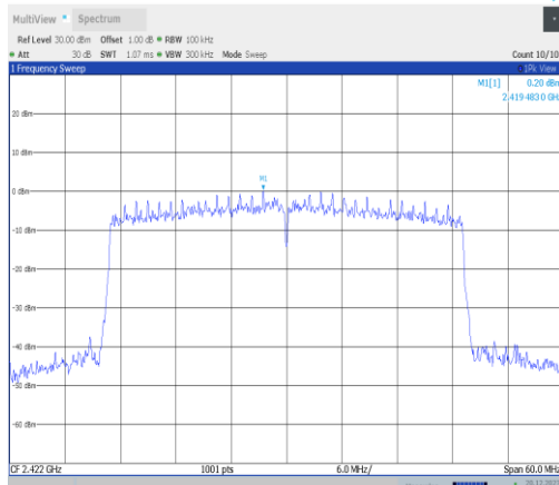
11ax40MIMO-Ant4-2422-0~Reference-PASS
