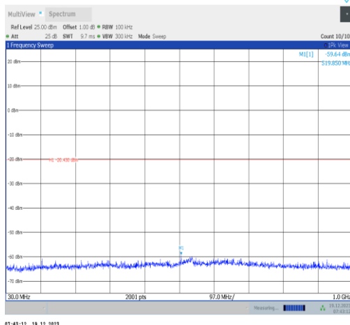
11n40SISO-Ant2-2437-30~1000-PASS
