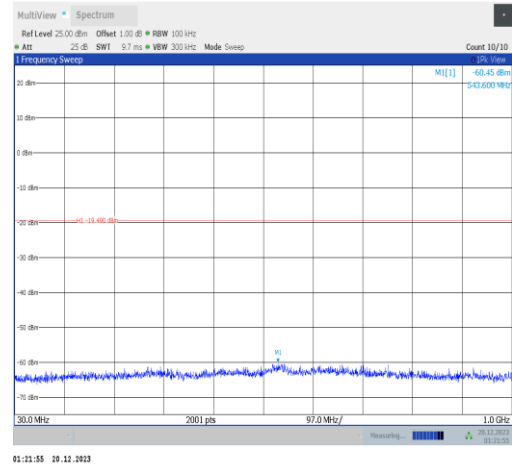
11ax40MIMO-Ant4-2452-30~1000-PASS
