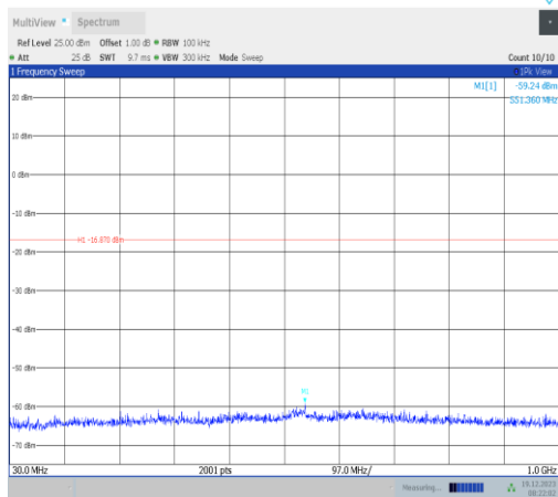
11ax20MIMO-Ant3-2412-30~1000-PASS
