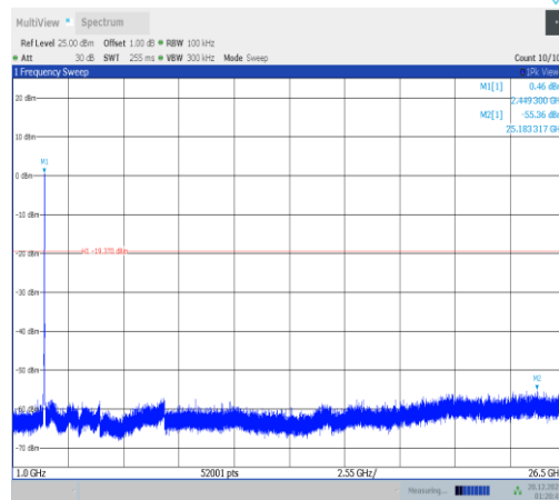
11ax40MIMO-Ant3-2452-1000~26500-PASS
