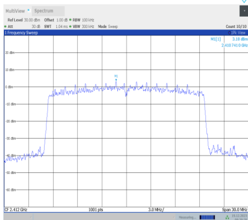
11ax20MIMO-Ant2-2412-0~Reference-PASS
