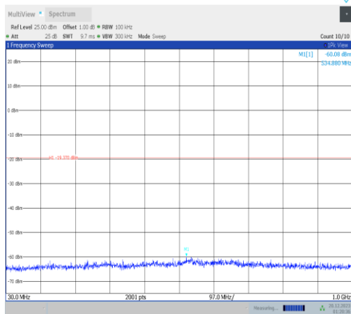
11ax40MIMO-Ant3-2452-30~1000-PASS
