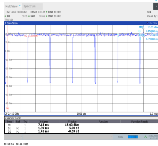
NTVN-11g-Ant3-2412
