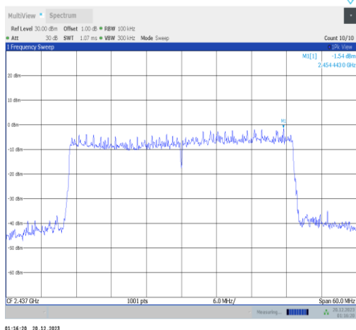
11ax40MIMO-Ant4-2437-0~Reference-PASS
