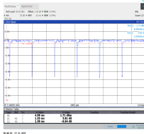
NTVN-11ax20MIMO-Ant4-2412-26Tone-RU0
