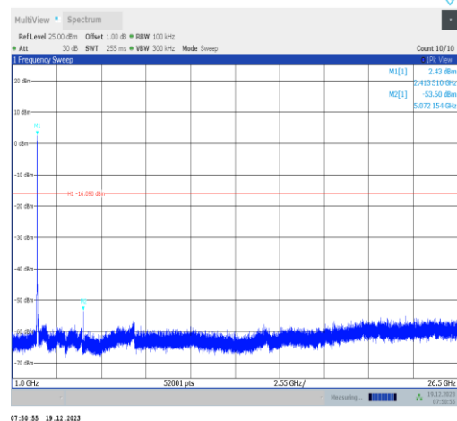
11ax20MIMO-Ant1-2412-1000~26500-PASS
