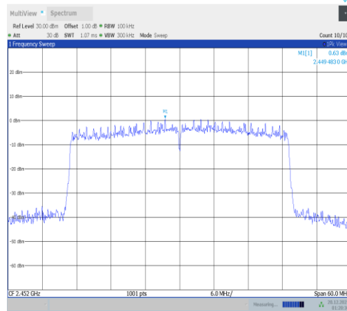
11ax40MIMO-Ant3-2452-0~Reference-PASS
