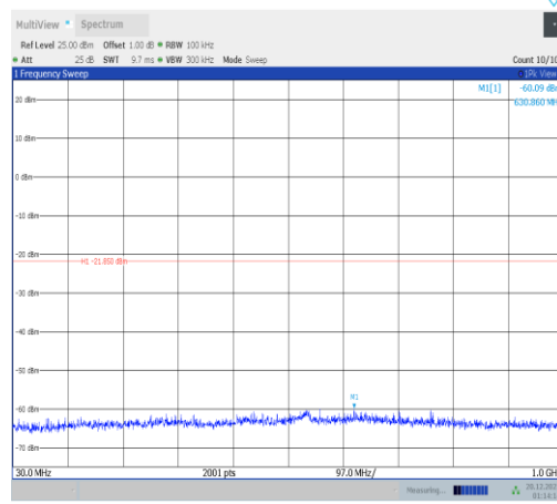
11ax40MIMO-Ant2-2437-30~1000-PASS
