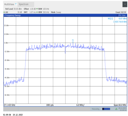
11ax40MIMO-Ant3-2422-0~Reference-PASS
