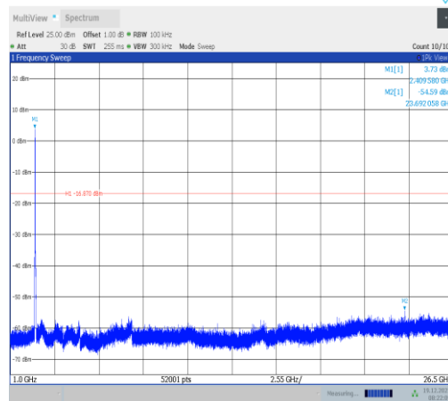
11ax20MIMO-Ant3-2412-1000~26500-PASS
