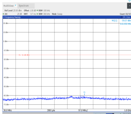
11ax20MIMO-Ant4-2412-30~1000-PASS
