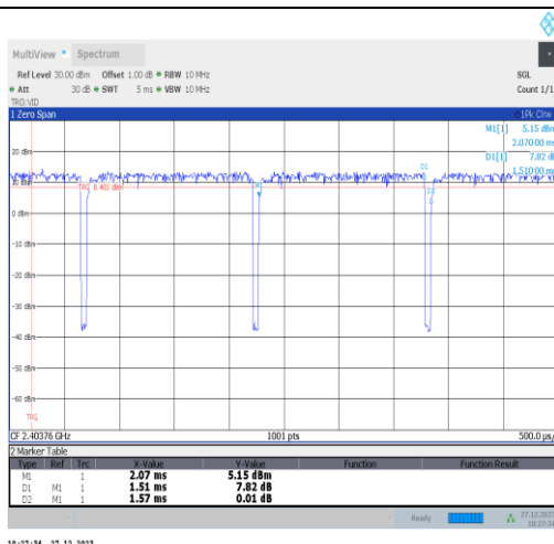
NTNV-11ax20MIMO-Ant4-2412-52Tone-RU37
