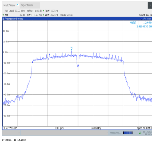
11n40SISO-Ant2-2422-0~Reference-PASS
