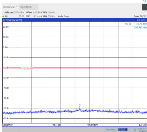
11ax40MIMO-Ant3-2437-30~1000-PASS
