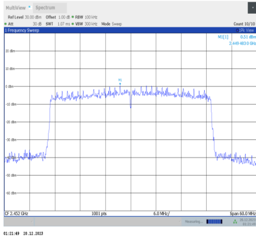
11ax40MIMO-Ant4-2452-0~Reference-PASS
