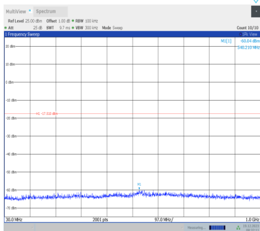
11ax20MIMO-Ant1-2462-30~1000-PASS
