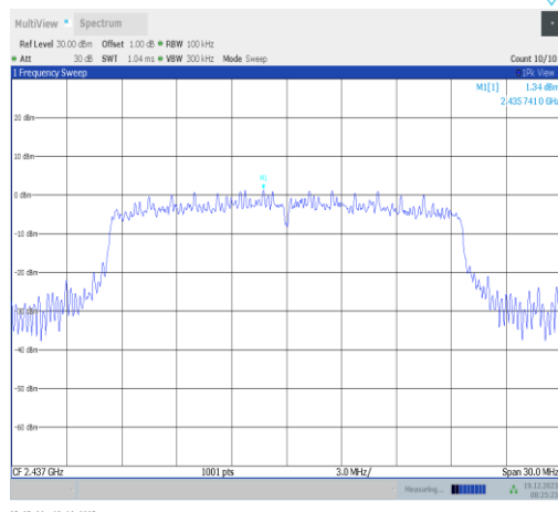
11ax20MIMO-Ant1-2437-0~Reference-PASS
