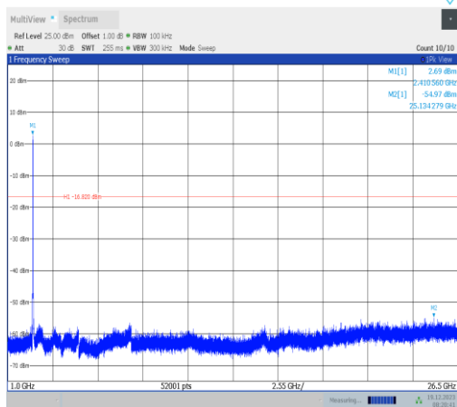
11ax20MIMO-Ant2-2412-1000~26500-PASS
