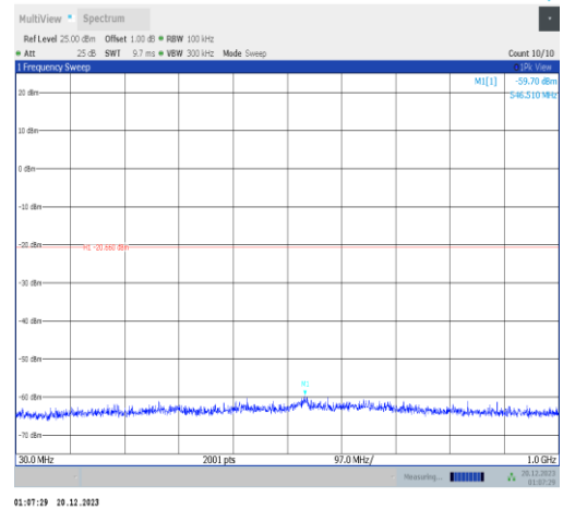
11ax40MIMO-Ant2-2422-30~1000-PASS
