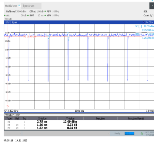
NTNV-11n40SISO-Ant1-2422
