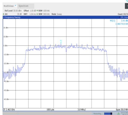
11ax20MIMO-Ant3-2462-0~Reference-PASS
