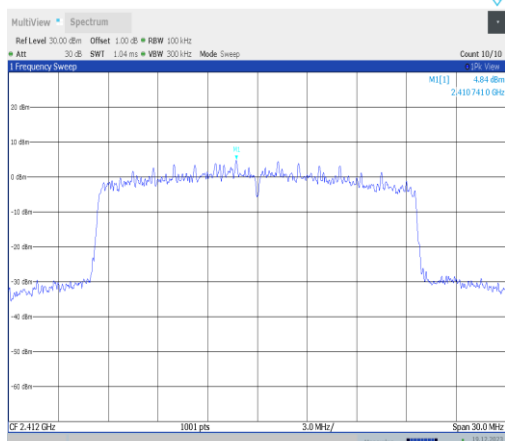
11ax20MIMO-Ant4-2412-0~Reference-PASS
