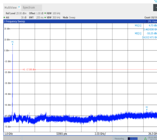
11ax20MIMO-Ant3-2462-1000~26500-PASS
