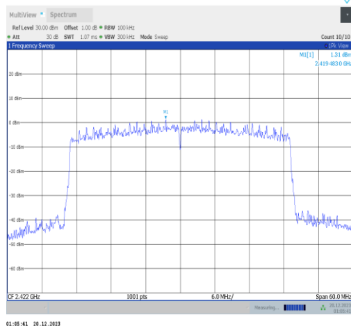
11ax40MIMO-Ant1-2422-0~Reference-PASS
