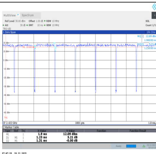
NTVN-11n40SISO-Ant4-2422
