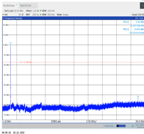
11n20SISO-Ant2-2437-1000~26500-PASS
