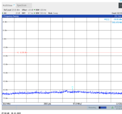
11ax20MIMO-Ant1-2412-30~1000-PASS
