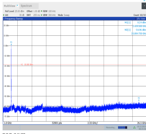
11ax20MIMO-Ant1-2437-1000~26500-PASS
