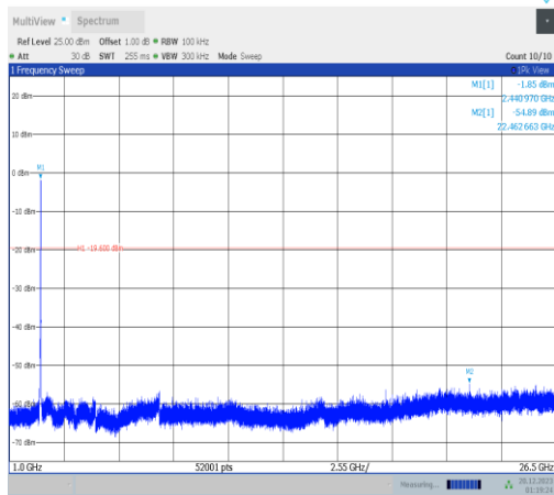
11ax40MIMO-Ant2-2452-1000~26500-PASS
