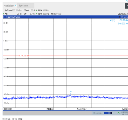
11ax20MIMO-Ant2-2412-30~1000-PASS
