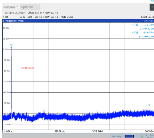
11ax20MIMO-Ant2-2462-1000~26500-PASS
