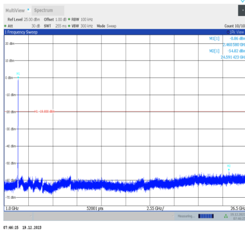
11n40SISO-Ant2-2452-1000~26500-PASS
