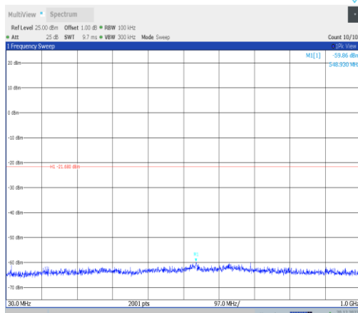
11ax40MIMO-Ant1-2437-30~1000-PASS
