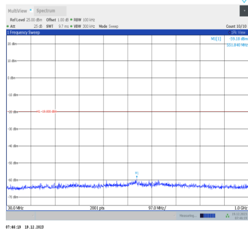
11n40SISO-Ant2-2452-30~1000-PASS
