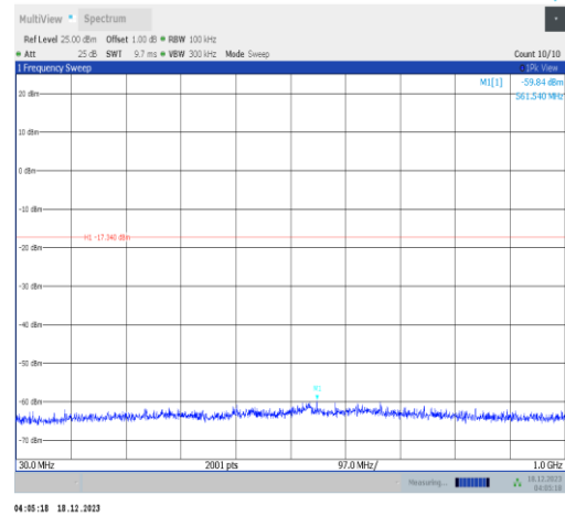
11n20SISO-Ant2-2437-30~1000-PASS
