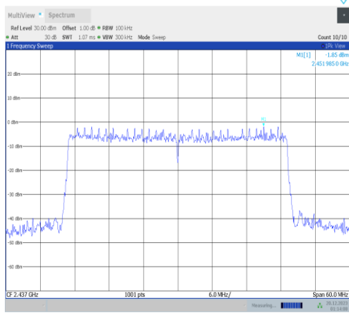
11ax40MIMO-Ant2-2437-0~Reference-PASS
