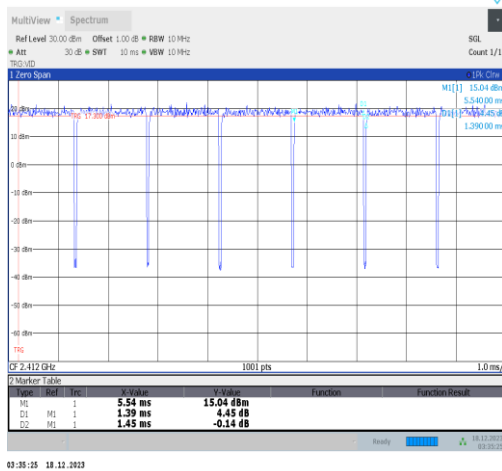
NTVN-11g-Ant2-2412
