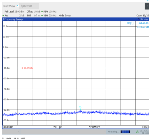
11ax40MIMO-Ant3-2422-30~1000-PASS
