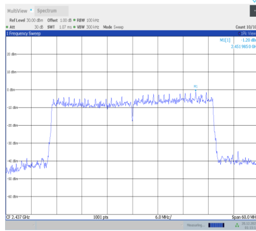
11ax40MIMO-Ant3-2437-0~Reference-PASS
