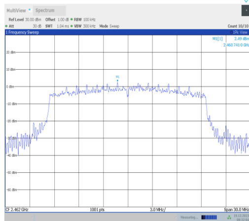
11ax20MIMO-Ant1-2462-0~Reference-PASS
