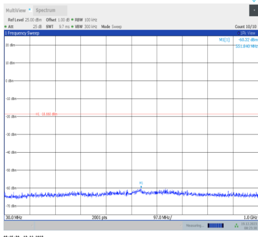
11ax20MIMO-Ant1-2437-30~1000-PASS
