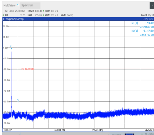
11ax40MIMO-Ant4-2422-1000~26500-PASS
