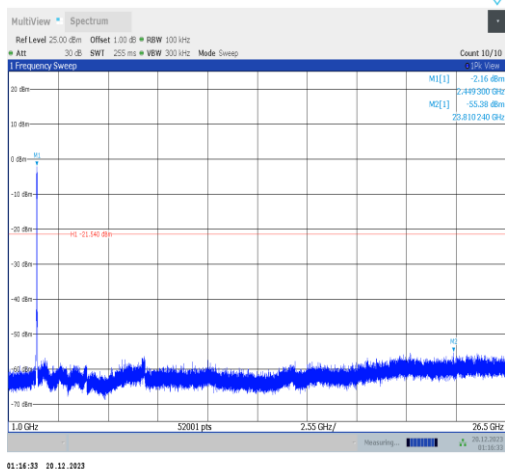
11ax40MIMO-Ant4-2437-1000~26500-PASS
