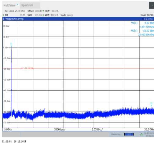
11ax40MIMO-Ant4-2452-1000~26500-PASS
