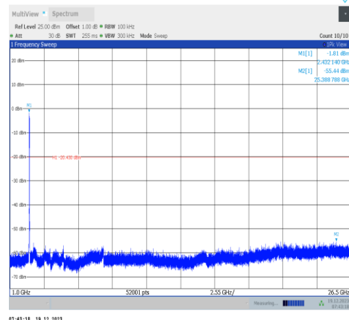
11n40SISO-Ant2-2437-1000~26500-PASS
