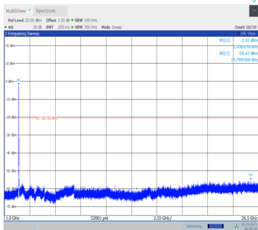
11ax20MIMO-Ant4-2437-1000~26500-PASS
