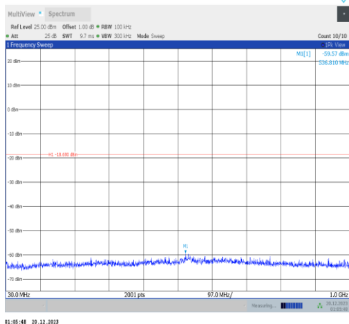
11ax40MIMO-Ant1-2422-30~1000-PASS
