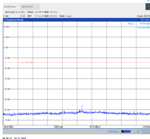
11ax20MIMO-Ant4-2462-30~1000-PASS
