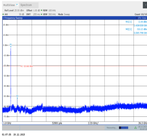
11ax40MIMO-Ant2-2422-1000~26500-PASS
