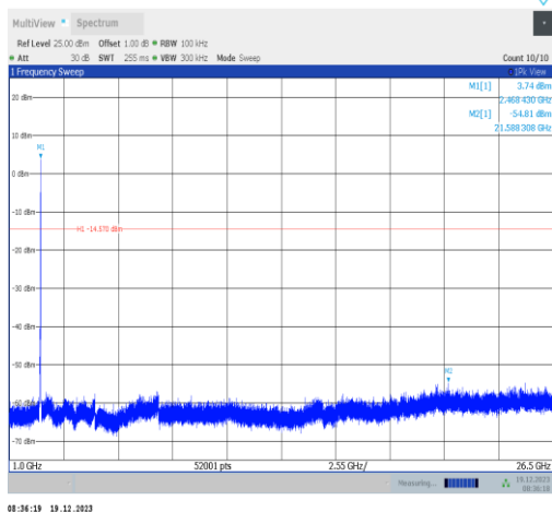
11ax20MIMO-Ant4-2462-1000~26500-PASS
