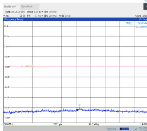
11ax40MIMO-Ant2-2452-30~1000-PASS
