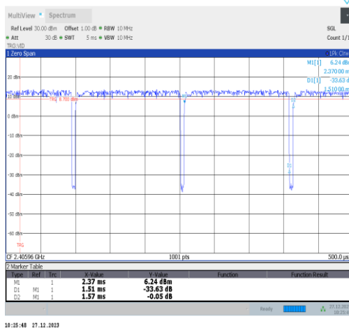
NTVN-11ax20MIMO-Ant2-2412-52Tone-RU37
