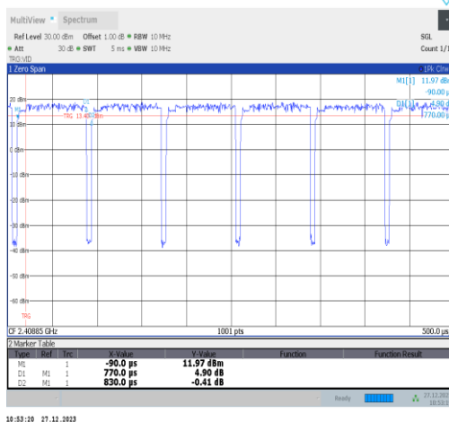
NTVN-11ax20MIMO-Ant3-2412-106Tone-RU53
