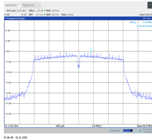
11n40SISO-Ant2-2437-0~Reference-PASS
