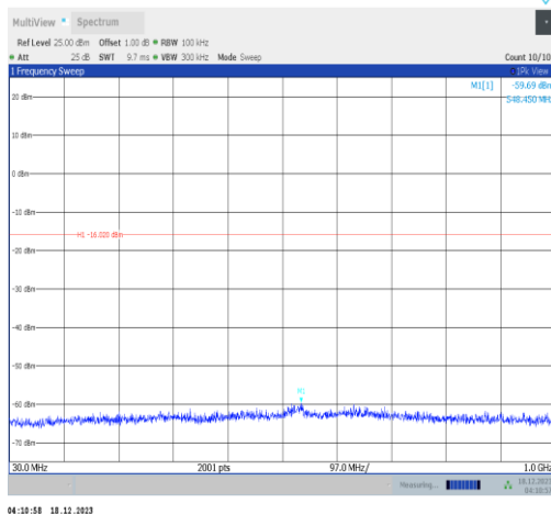
11n20SISO-Ant2-2462-30~1000-PASS
