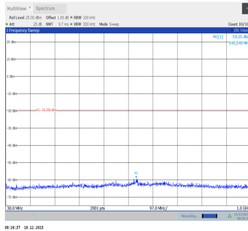
11ax20MIMO-Ant2-2437-30~1000-PASS
