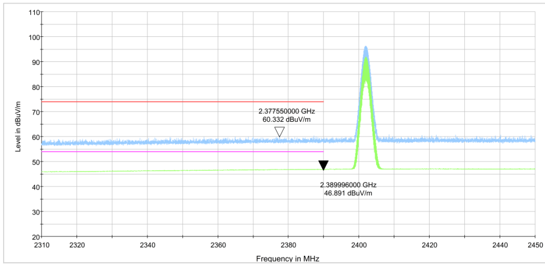
Fig.17. Frequency Band Edges: 8DPSK, Channel 0, Hopping Off, 2.31 GHz - 2.45GHz
