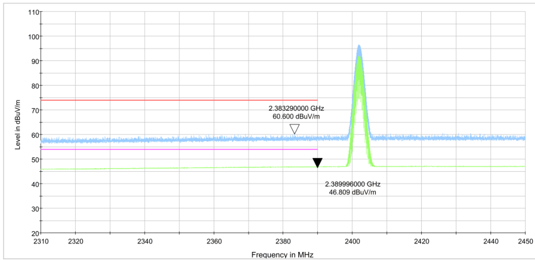
Fig.15. Frequency Band Edges: \pi/4 DQPSK, Channel 0, Hopping Off, 2.31 GHz - 2.45GHz
