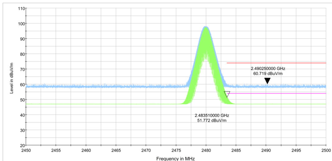
Fig.14. Frequency Band Edges: GFSK, Channel 78, Hopping Off, 2.45 GHz - 2.50GHz
