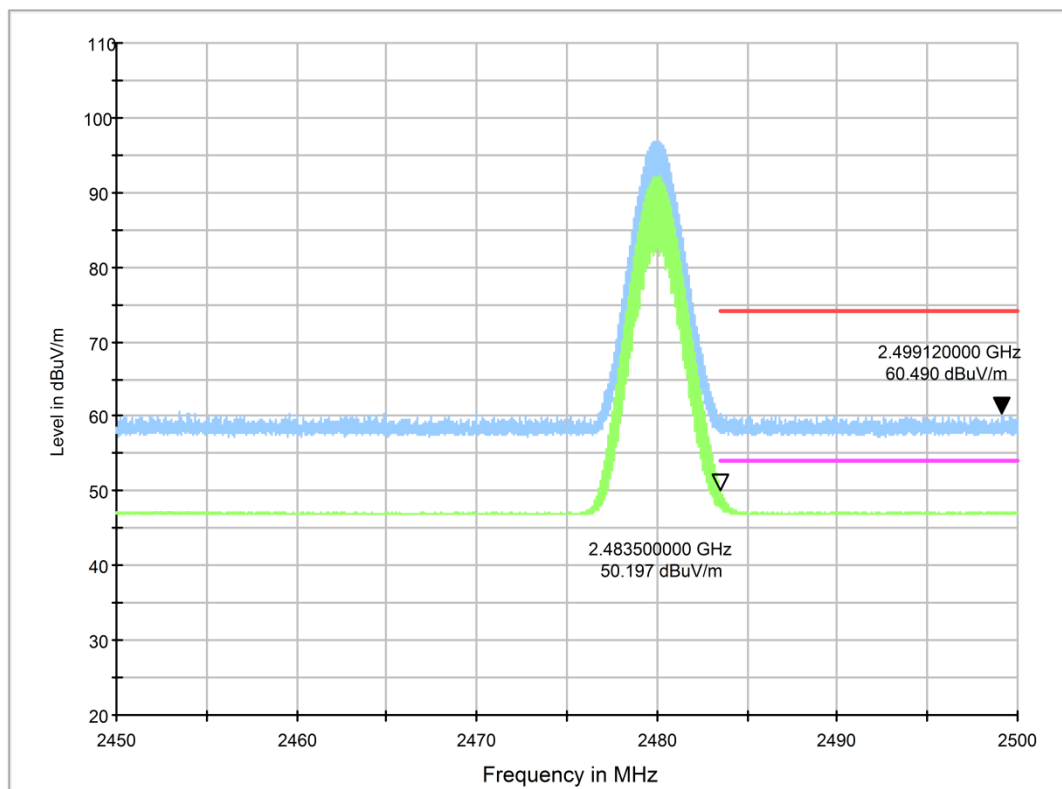
Fig.18. Frequency Band Edges: 8DPSK, Channel 78, Hopping Off, 2.45 GHz - 2.50GHz
