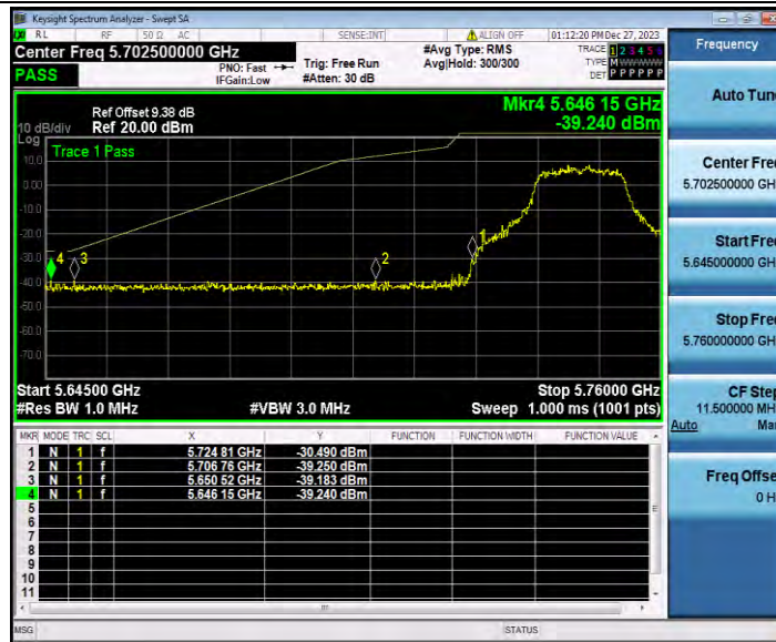
11A_Ant1_Low_5745
