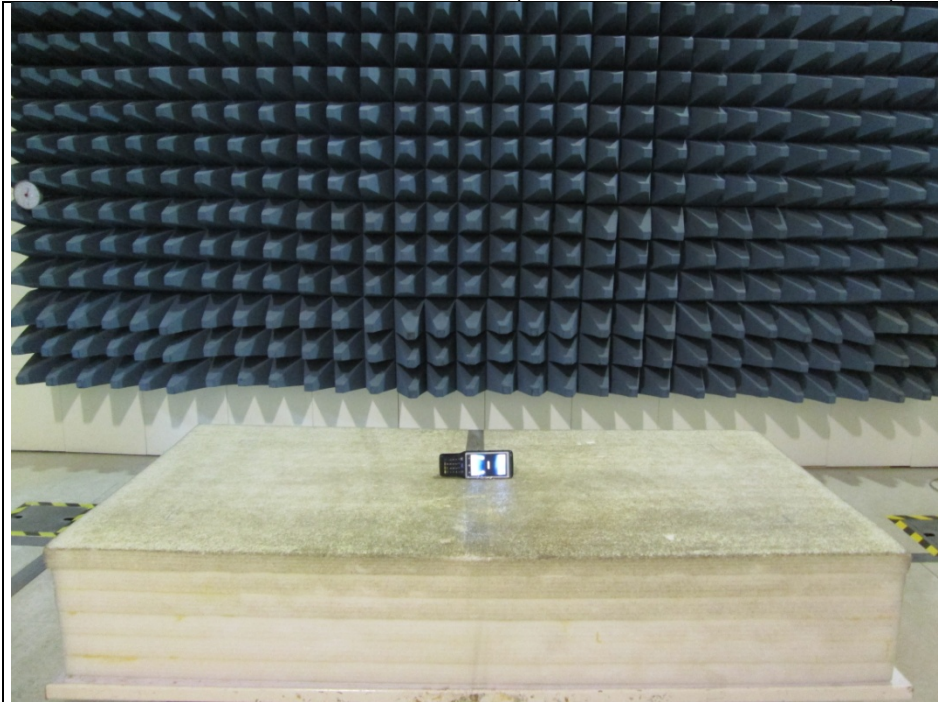
Radiated Emissions below 1 GHz Test (For WLAN 5GHz: Test Mode A)
