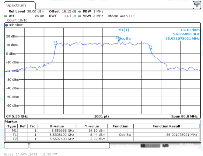
11AX40SISO-Ant1-5550
