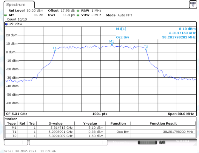
11AX40SISO-Ant1-5310
