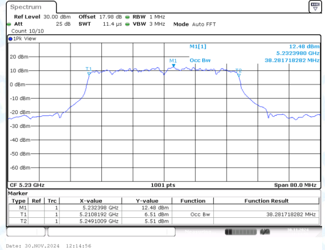
11AX40SISO-Ant1-5230
