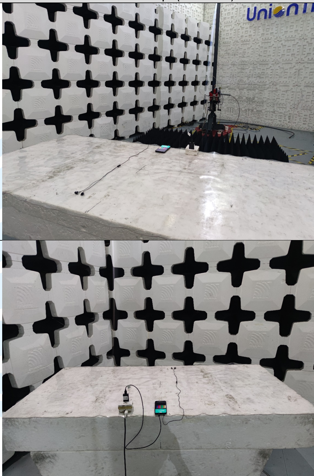
Radiated emission Test Setup-2 (Above 1 GHz) - Mode 1
