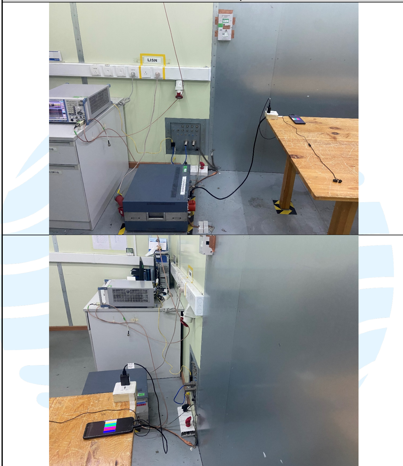
Conducted Emission Test Setup-3 - Mode 2
