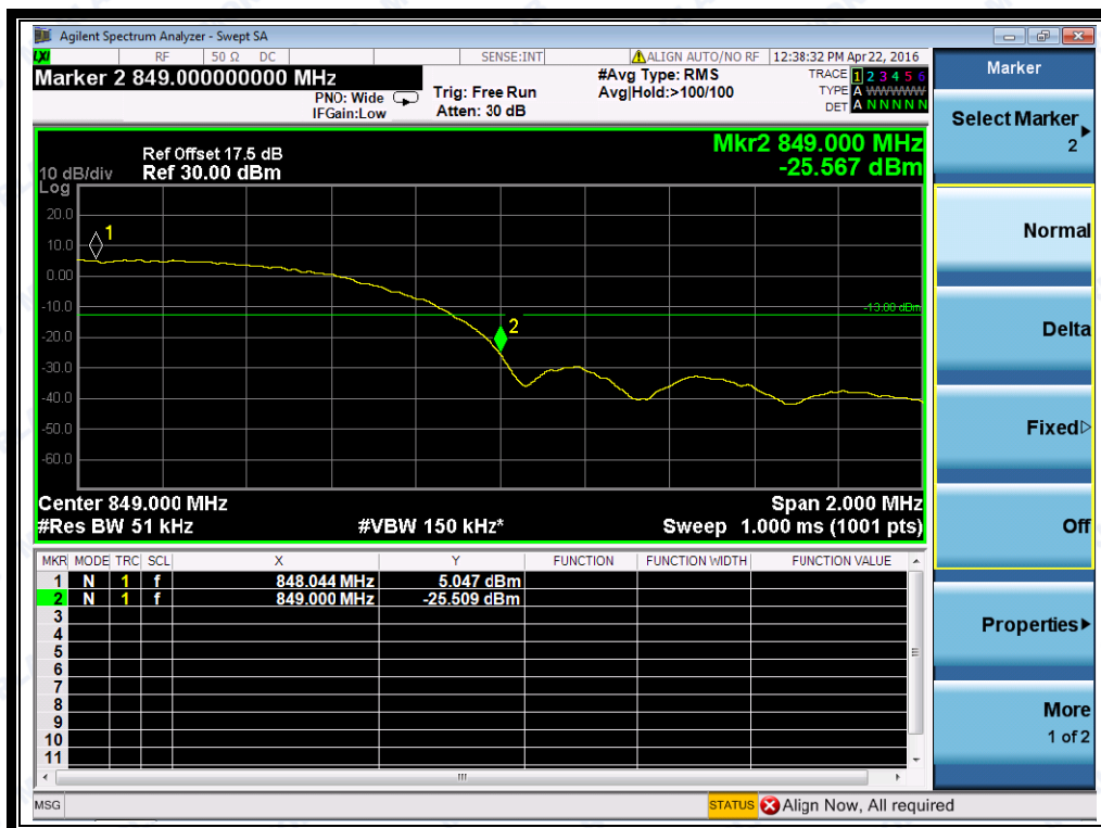
(Plot N2: HSPA+ 850 Channel = 4233)
