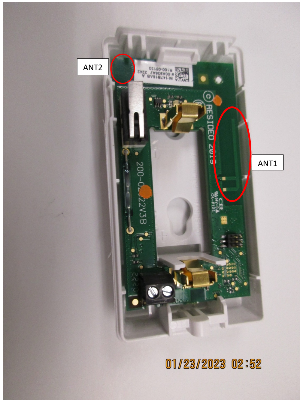
Figure 3 PCB with Antennas
