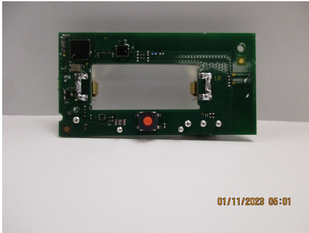
Figure 4 PCB BACK
