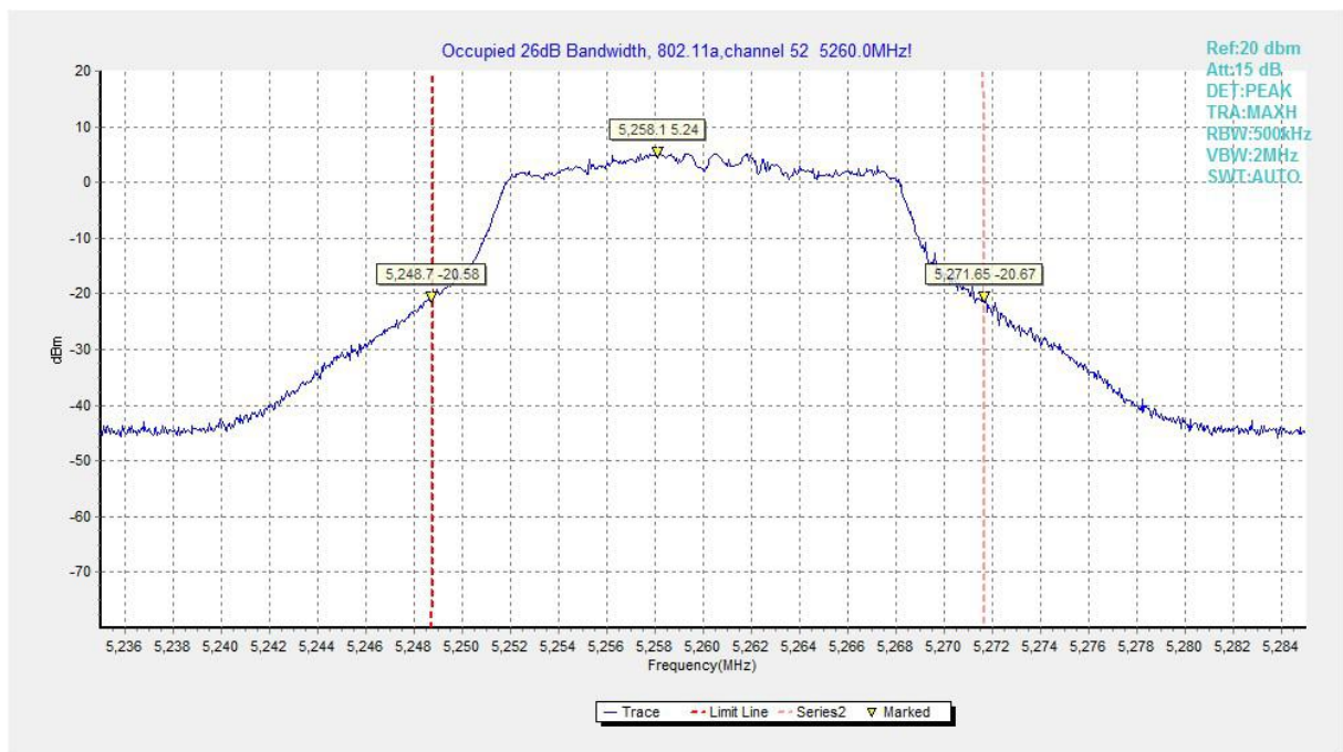
Fig.151 Occupied 26dB Bandwidth (802.11a, 5260MHz)
