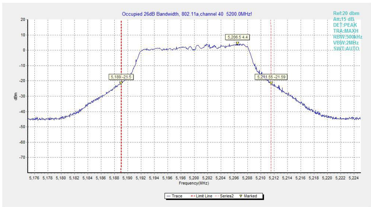
Fig.149 Occupied 26dB Bandwidth (802.11a, 5200MHz)
