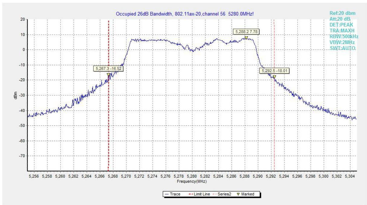
Fig.181 Occupied 26dB Bandwidth (802.11ax-HE20, 5280MHz)
