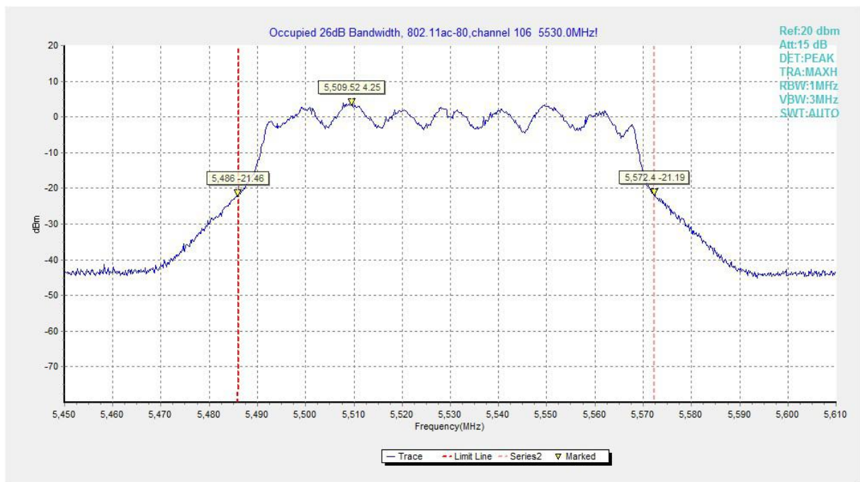
Fig.175 Occupied 26dB Bandwidth (802.11ac-HT80, 5530MHz)
