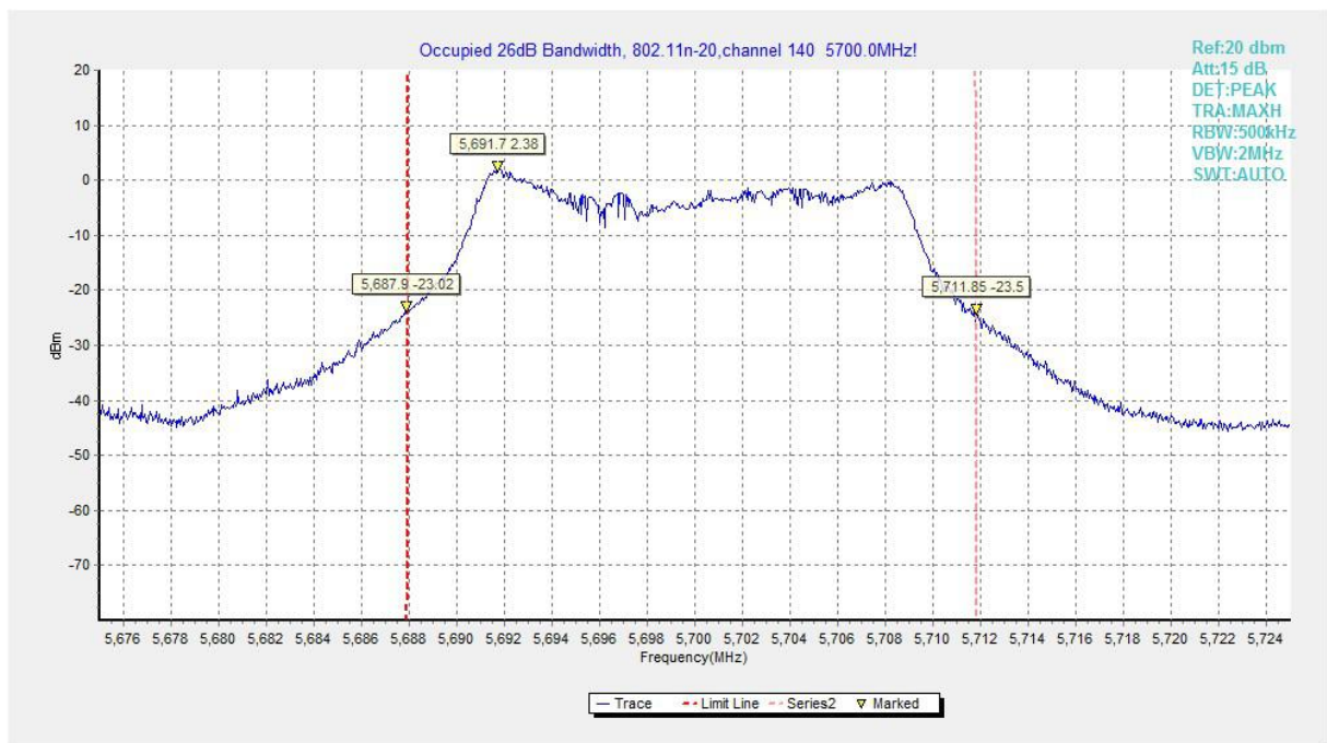
Fig.165 Occupied 26dB Bandwidth (802. 11n-HT20, 5700MHz)
