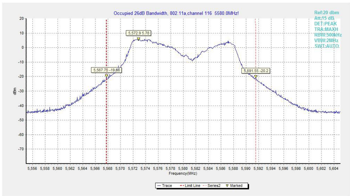
Fig.155 Occupied 26dB Bandwidth (802.11a, 5580MHz)
