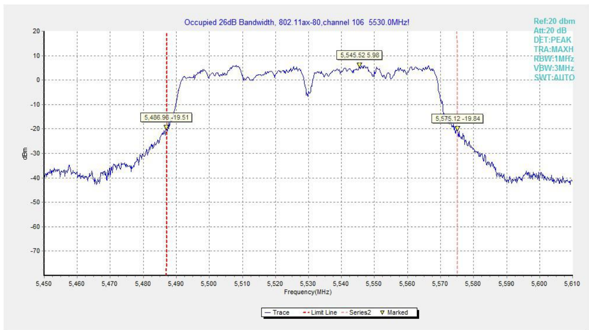
Fig.195 Occupied 26dB Bandwidth (802.11ax-HE80,5530MHz)
