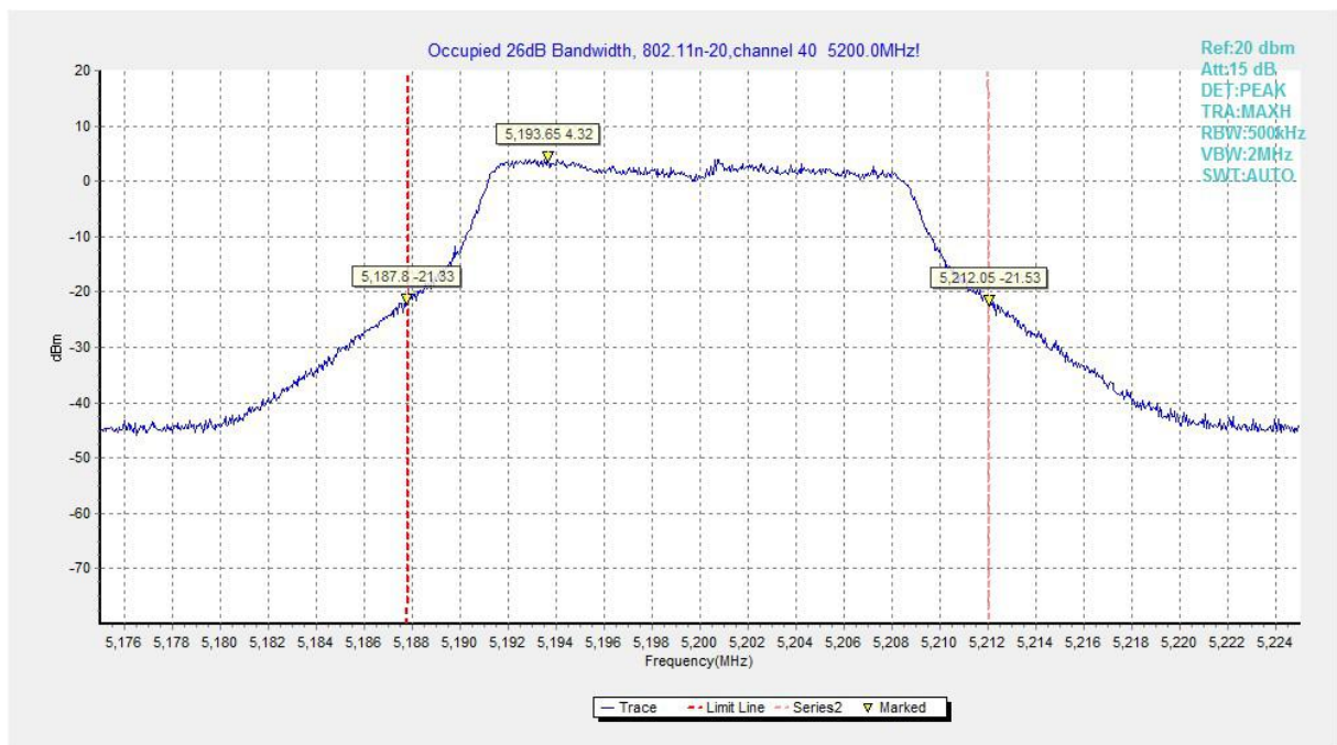
Fig.158 Occupied 26dB Bandwidth (802.11n-HT20, 5200MHz)
