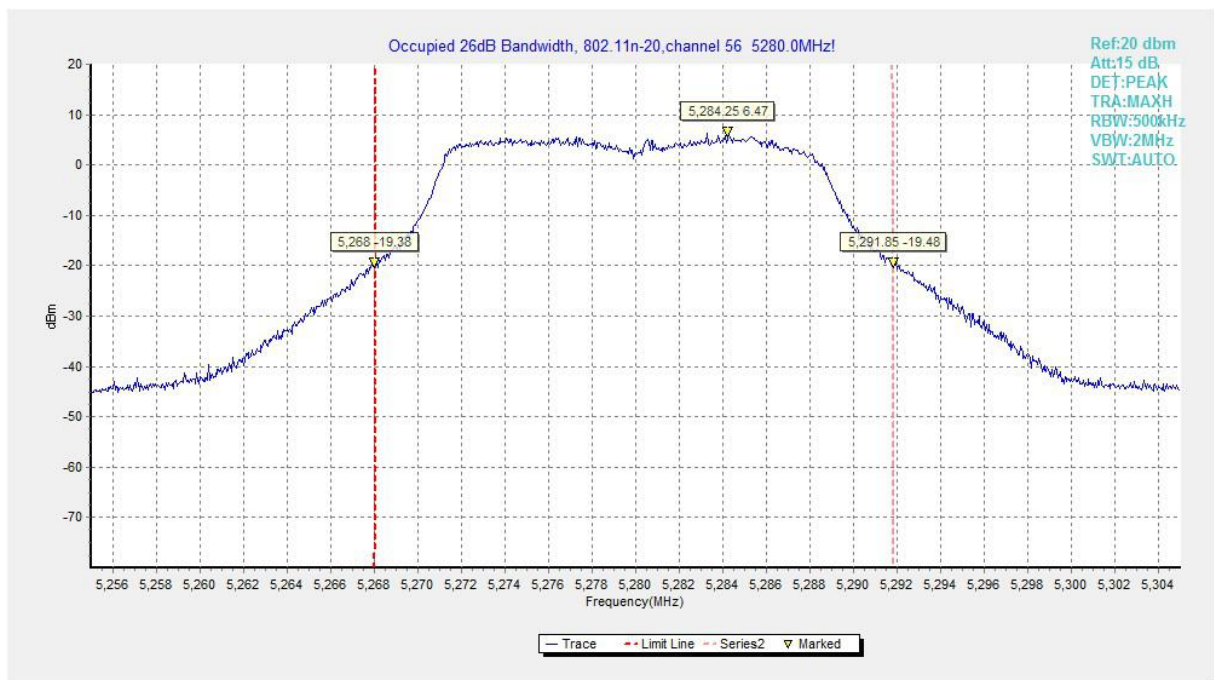
Fig.161 Occupied 26dB Bandwidth (802.11n-HT20, 5280MHz)
