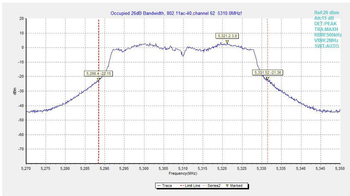
Fig.169 Occupied 26dB Bandwidth (802.11ac-HT40, 5310MHz)
