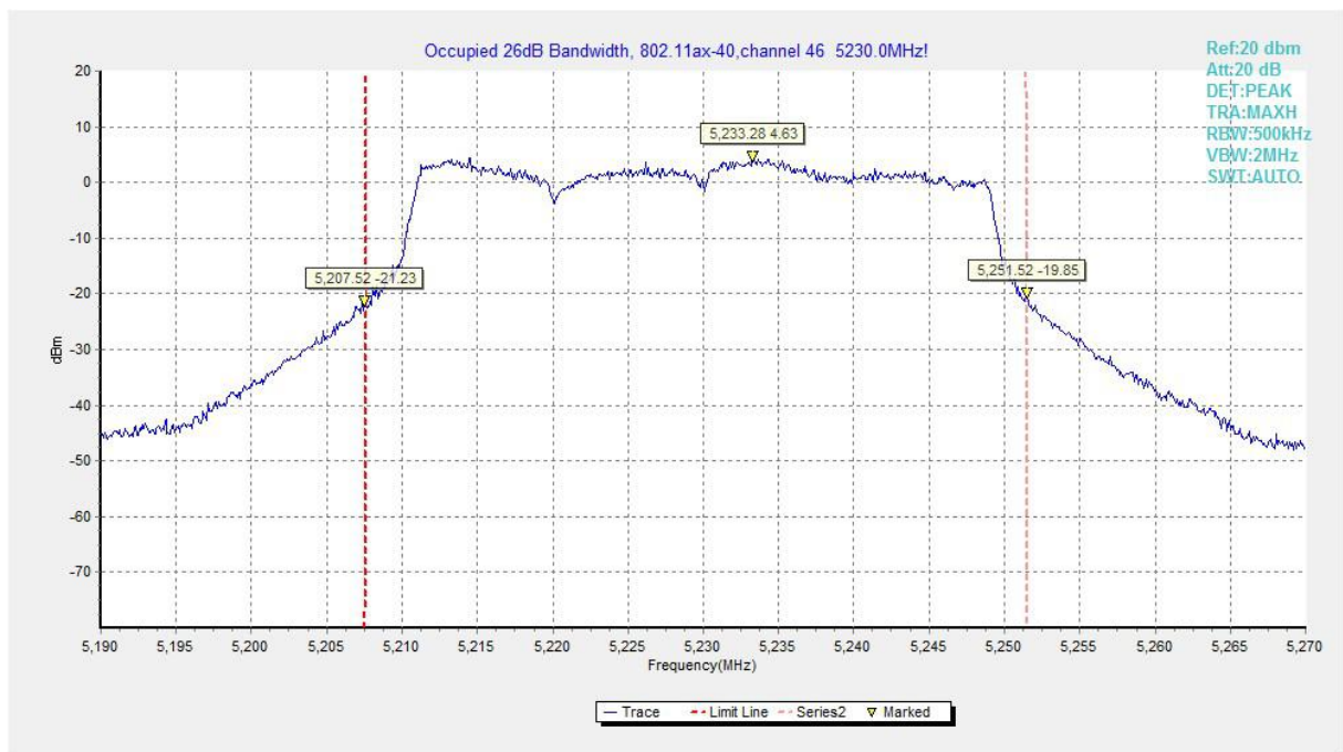
Fig.187 Occupied 26dB Bandwidth (802.11ax-HE40, 5230MHz)
