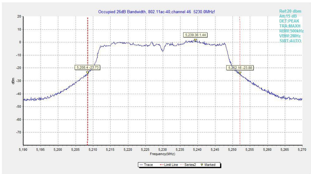
Fig.167 Occupied 26dB Bandwidth (802.11ac-HT40, 5230MHz)
