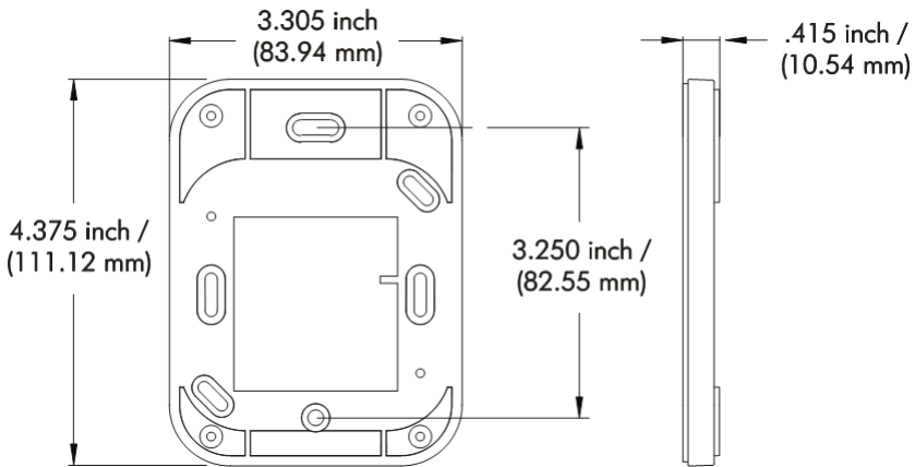
FIGURE 1. Model SWH-2100 Reader Backplate (includes tamper switch magnet)
