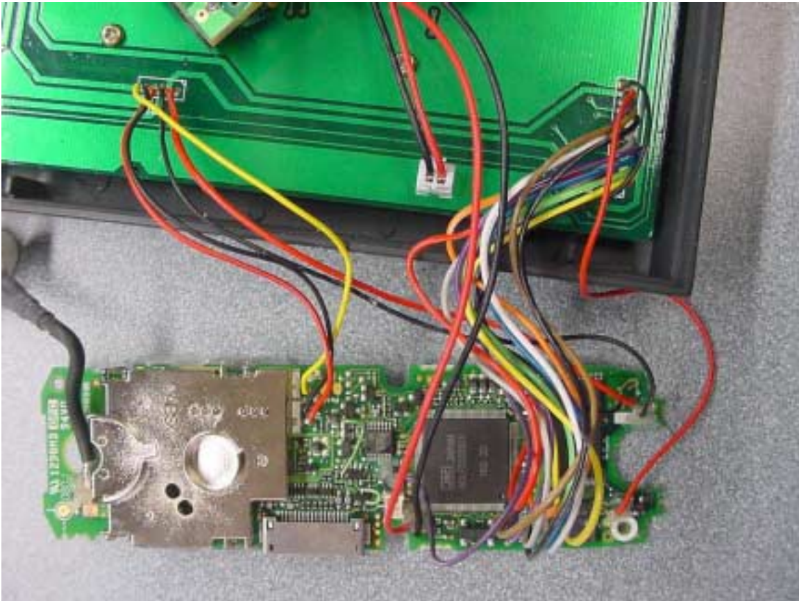
PHOTOGRAPH 30: RF PCB SHOWING CONNECTIONS TO KEYPAD PCB
