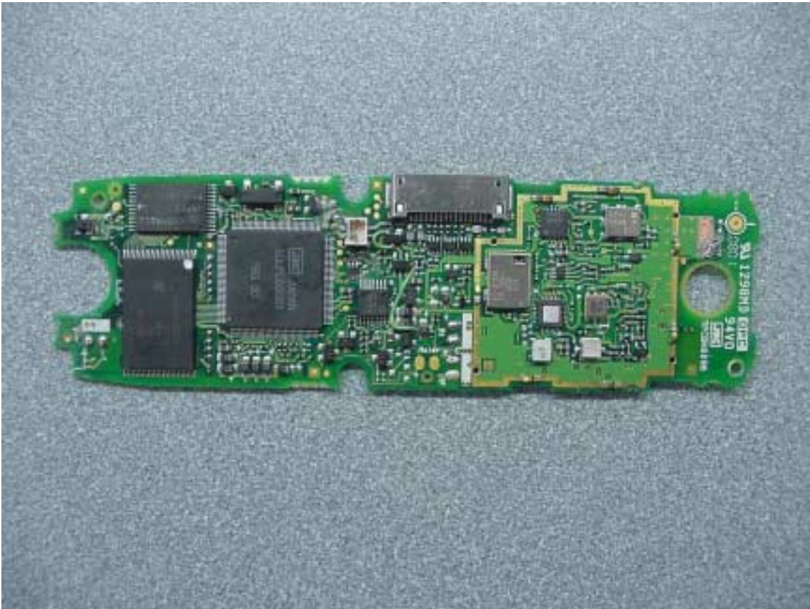
PHOTOGRAPH 44: COMPONENT SIDE OF RF PCB WITH COVER REMOVED
