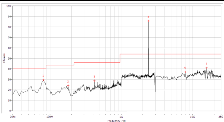
(Plot G.2: Antenna Horizontal, 30MHz to 25GHz)
