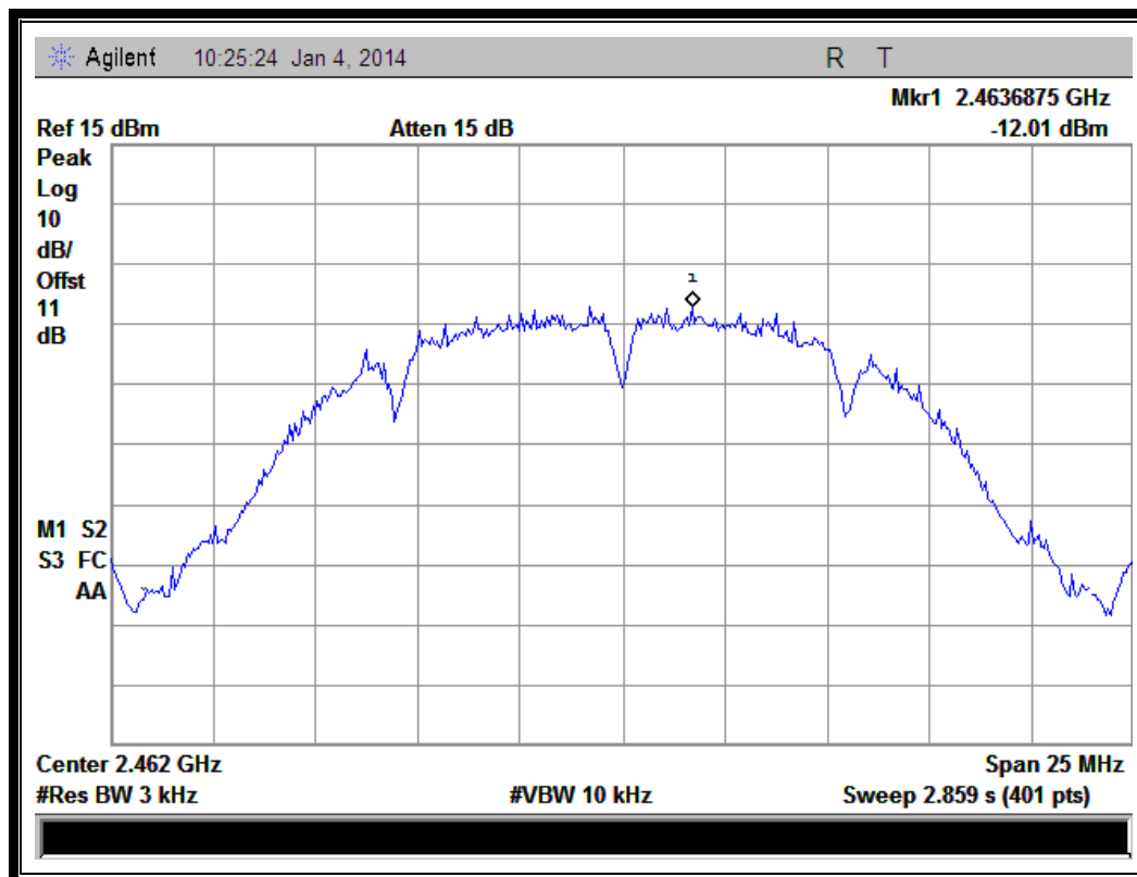
(Plot C: Channel = 11 @ 802.11b)
