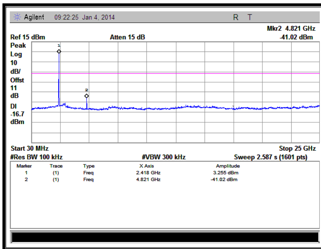
(Plot A.1: Channel = 1, 30MHz to 25GHz)
