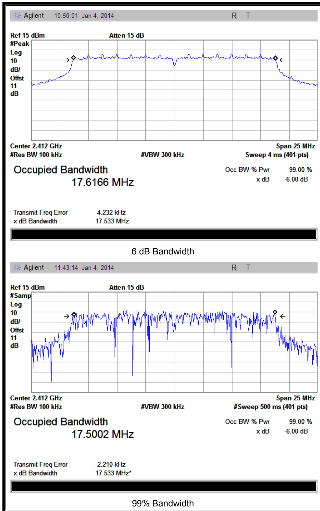
(Plot G: Channel 1: 2412MHz @ 802.11n-20)
