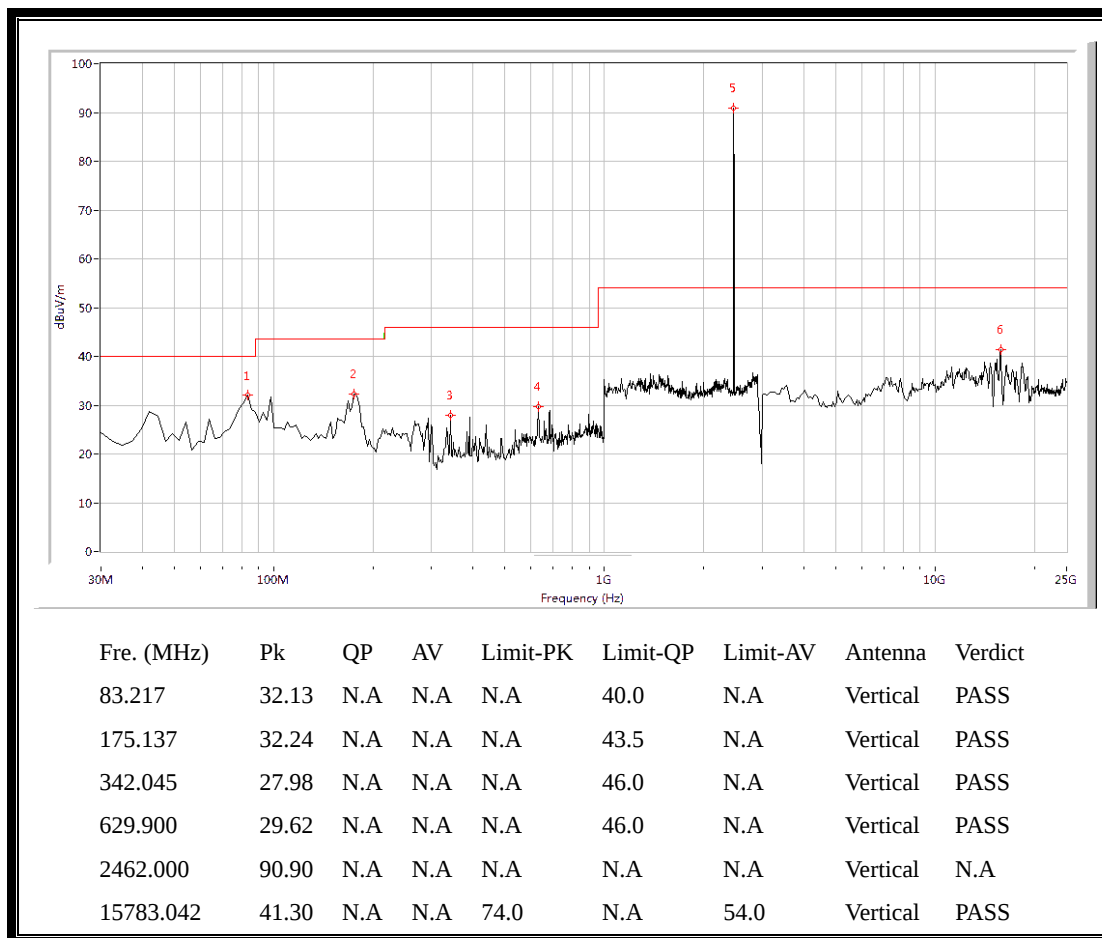
(Plot F.3: Antenna Vertical, 30MHz to 25GHz)
