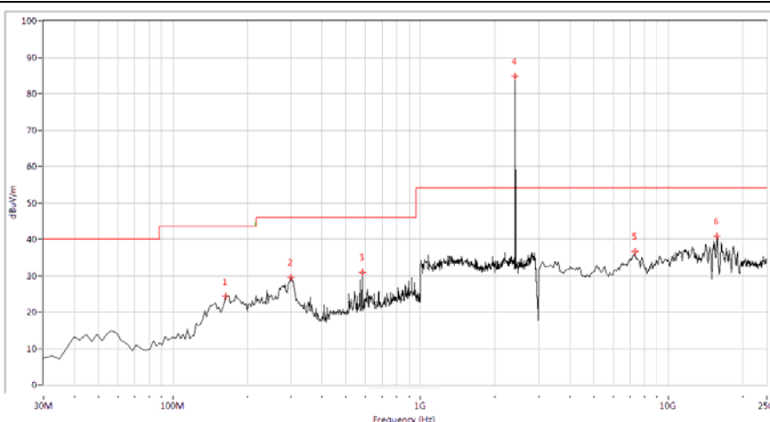
(Plot A.2: Antenna Horizontal, 30MHz to 25GHz)
