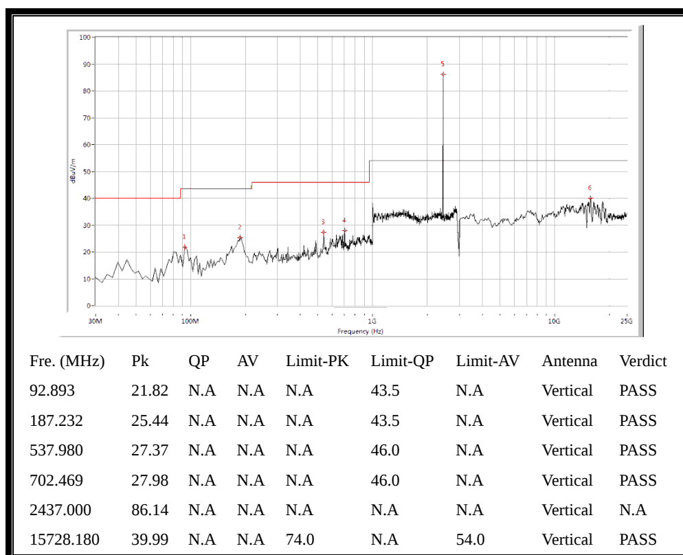
(Plot H.3: Antenna Vertical, 30MHz to 25GHz)
