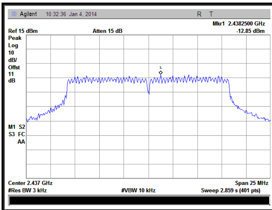
(Plot E: Channel = 6 @ 802.11g)
