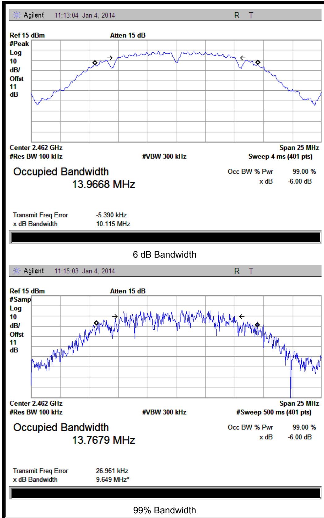
(Plot C: Channel 11: 2462MHz @ 802.11b)
