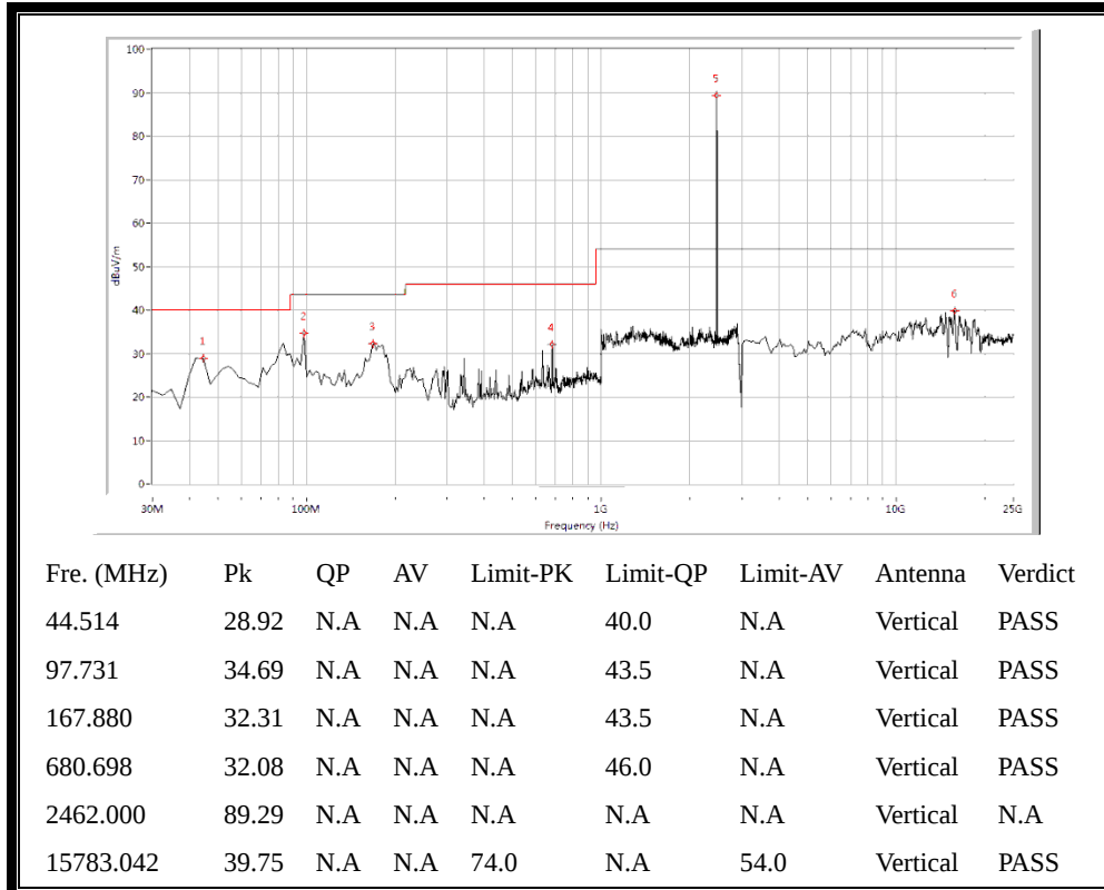
(Plot C.3: Antenna Vertical, 30MHz to 25GHz)
