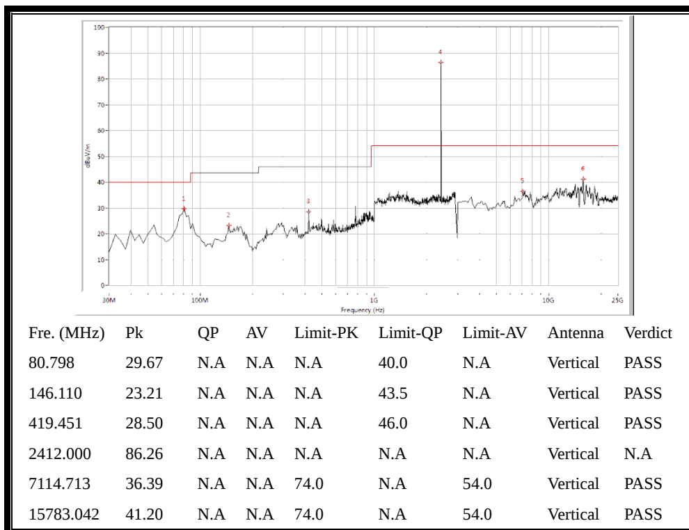
(Plot D.3: Antenna Vertical, 30MHz to 25GHz)
