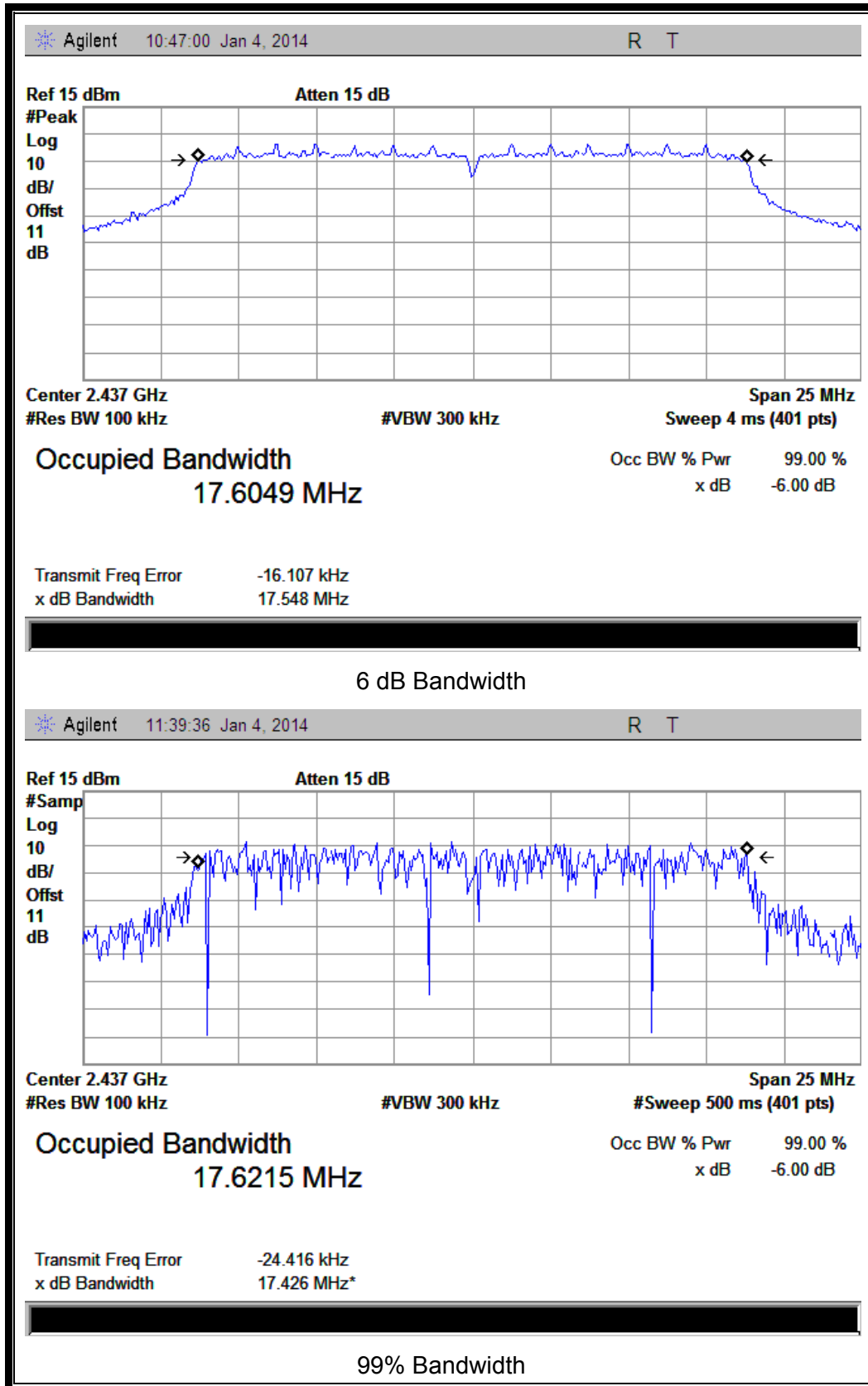
(Plot H: Channel 6: 2437MHz @ 802.11n-20)
