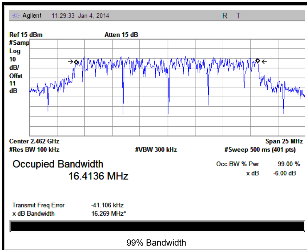
(Plot F: Channel 11: 2462MHz @ 802.11g)
