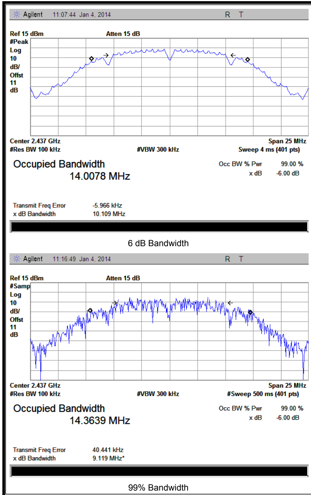
(Plot B: Channel 6: 2437 MHz @ 802.11b)
