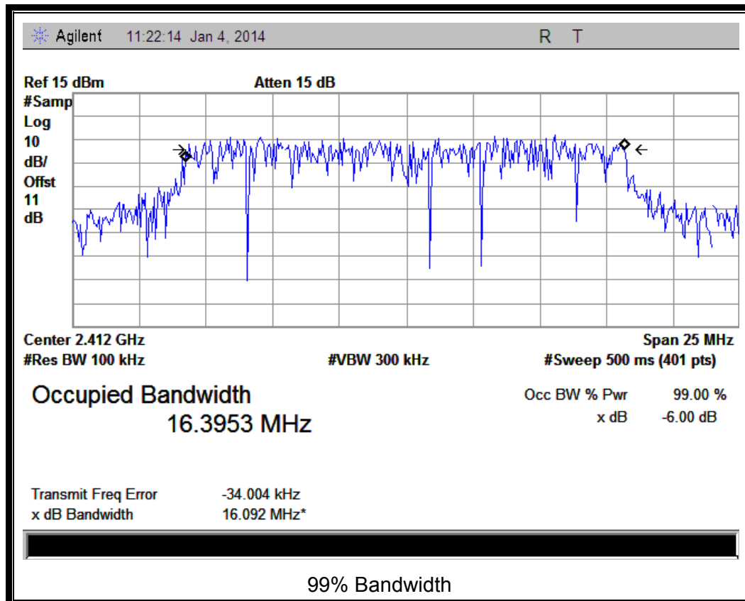
(Plot D: Channel 1: 2412MHz @ 802.11g)
