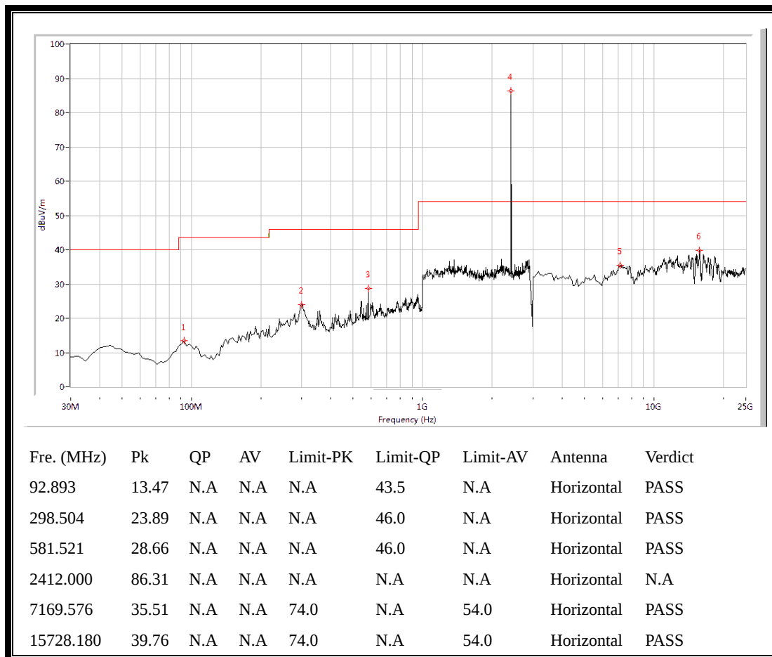
(Plot D.2: Antenna Horizontal, 30MHz to 25GHz)
