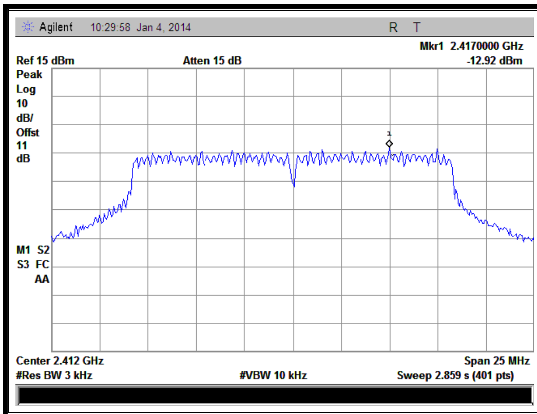
(Plot D: Channel = 1 @ 802.11g)
