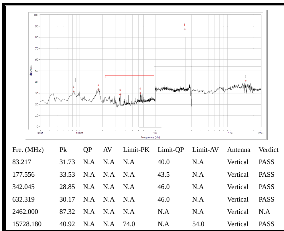
(Plot I.3: Antenna Vertical, 30MHz to 25GHz)
