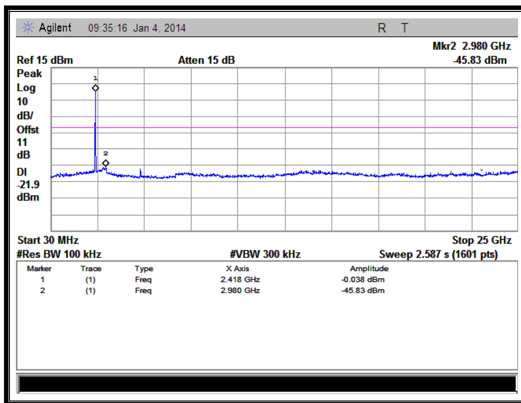
(Plot D.1: Channel = 1, 30MHz to 25GHz)
