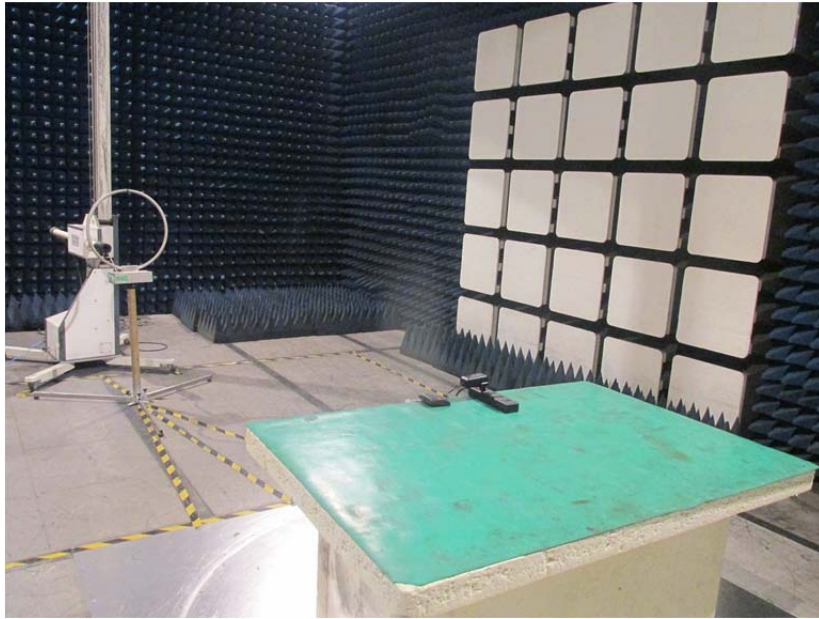
Test Setup
