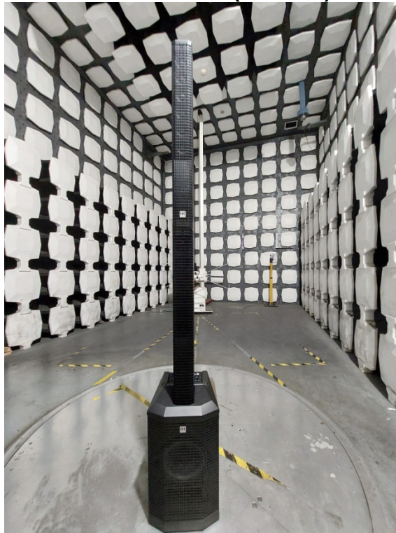
RadiatedEmission(Below 1G)
