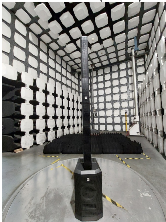
Radiated Emission (Above 1G)
