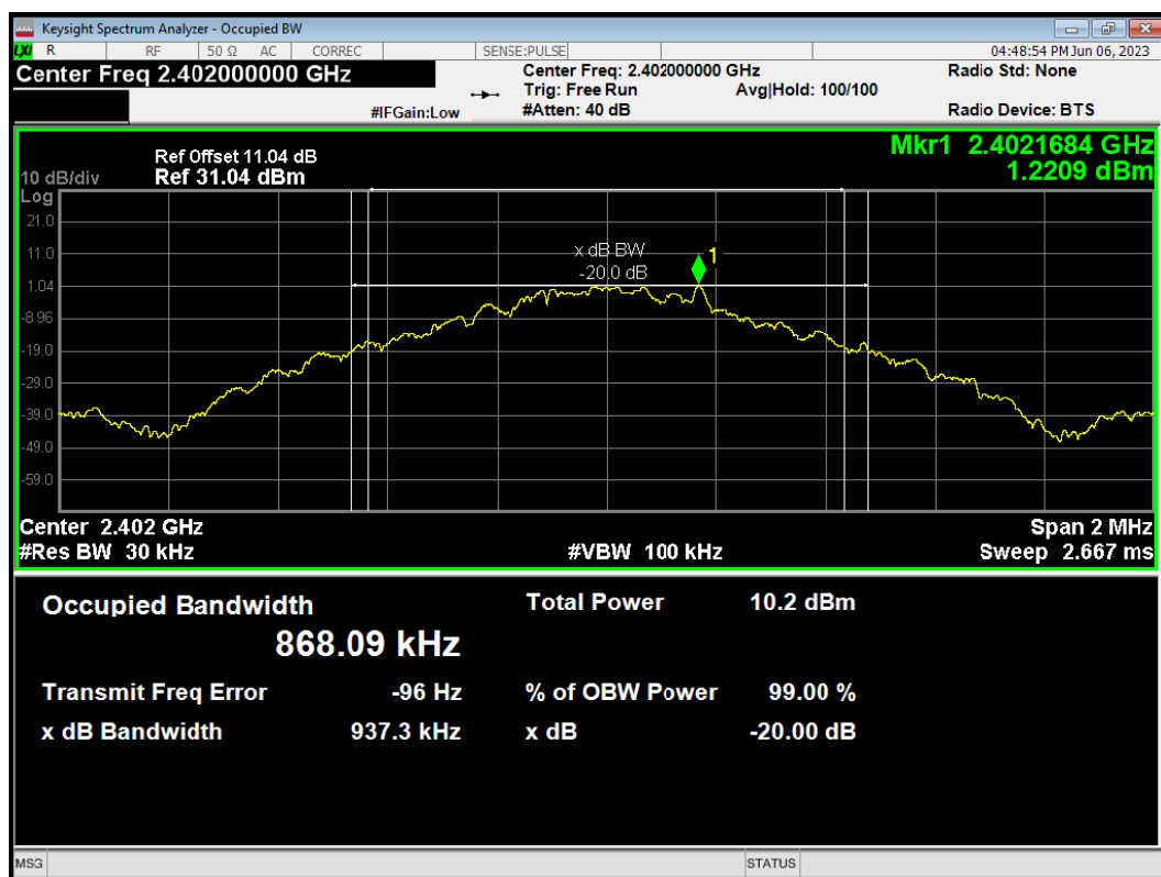
-20dB Bandwidth 1-DH5 2402MHz
