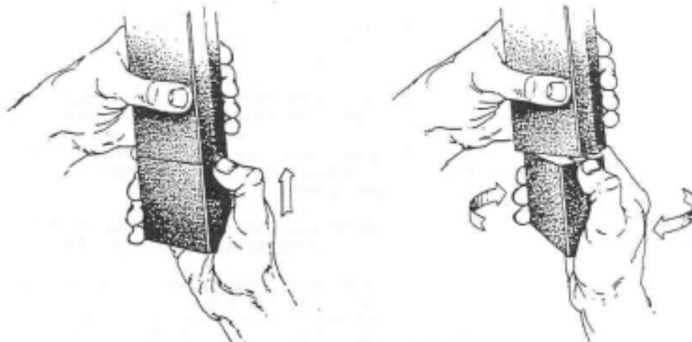
FIGURE 2-1 BATTERY INSTALLATION
