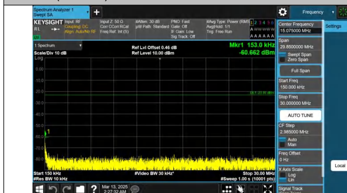
Band26(824-849)-3MHz-QPSK-26805-1RB#14-0.15~30-PASS
