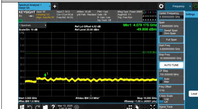
Band26(824-849)-15MHz-QPSK-26865-1RB#0-3000~10000-PAS
