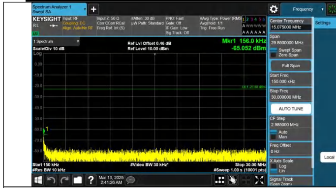
Band26(824-849)-5MHz-QPSK-27015-1RB#24-0.15~30-PASS
