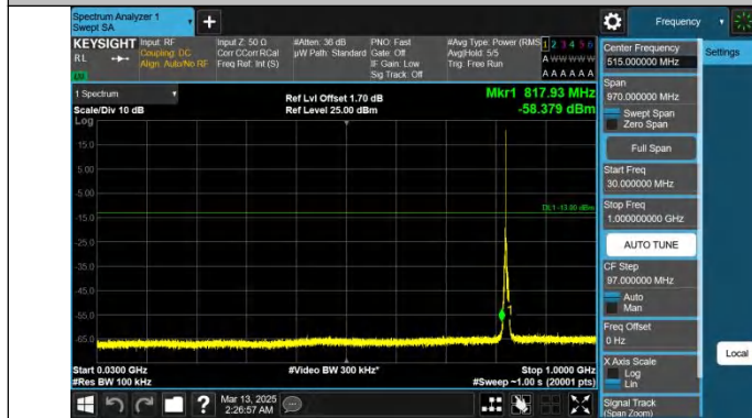
Band26(824-849)-3MHz-QPSK-26805-1RB#0-30~1000-PASS
