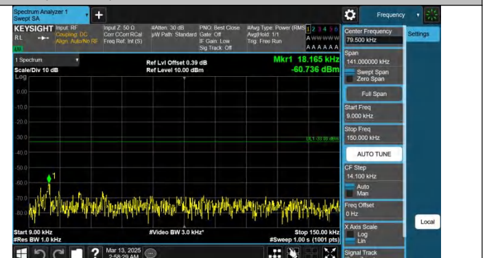
Band26(824-849)-15MHz-QPSK-26865-1RB#0-1000~3000-PASS
