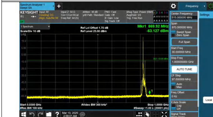
Band26(824-849)-15MHz-QPSK-26865-1RB#0-30~1000-PASS
