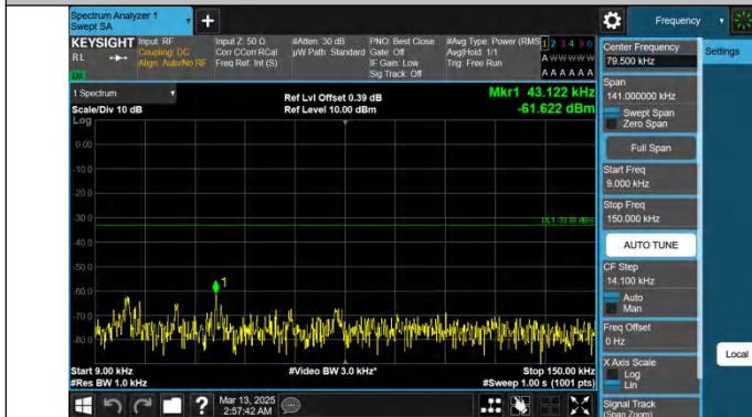
Band26(824-849)-15MHz-QPSK-26865-1RB#0-0.009~0.15-PASS
