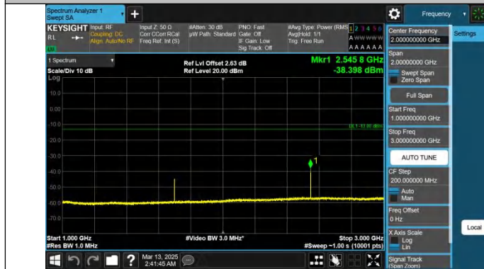
Band26(824-849)-5MHz-QPSK-27015-1RB#24-1000~3000-PASS
