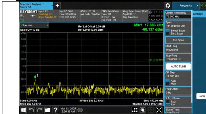
Band26(824-849)-3MHz-QPSK-26805-1RB#0-0.009~0.15-PASS
