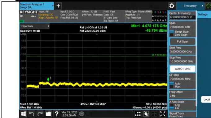
Band26(824-849)-15MHz-QPSK-26915-1RB#0-3000~10000-PAS S
