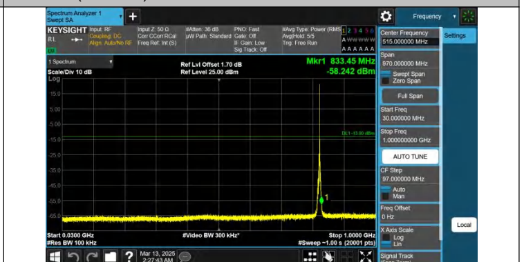
Band26(824-849)-3MHz-QPSK-26805-1RB#14-30~1000-PASS
