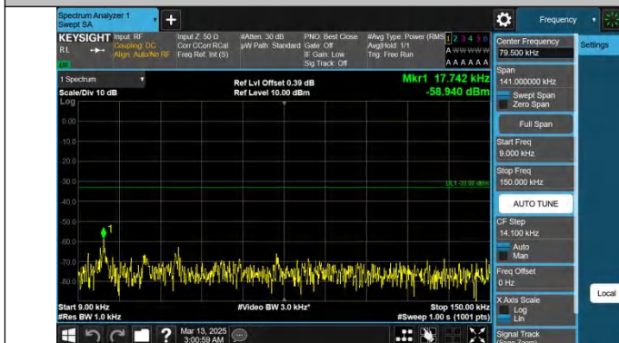
Band26(824-849)-15MHz-QPSK-26965-1RB#0-0.009~0.15-PASS
