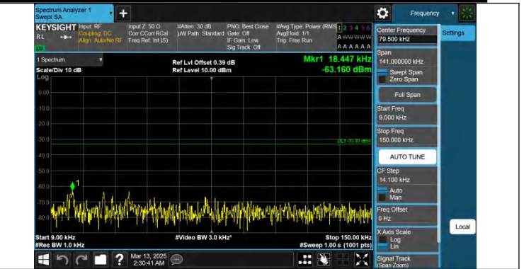
Band26(824-849)-3MHz-QPSK-27025-1RB#14-0.009~0.15-PASS
