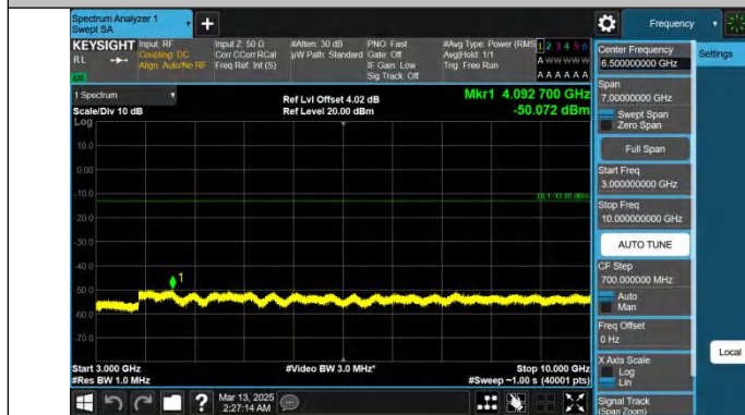
Band26(824-849)-3MHz-QPSK-26805-1RB#0-3000~10000-PASS
