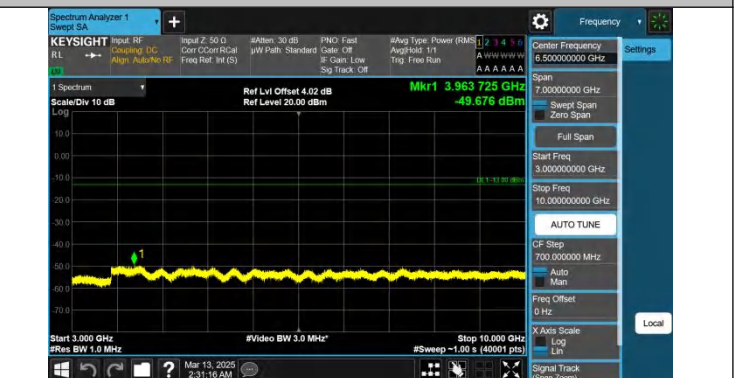
Band26(824-849)-3MHz-QPSK-27025-1RB#14-3000~10000-PASS
