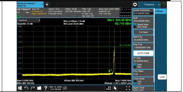
Band26(824-849)-5MHz-QPSK-27015-1RB#24-30~1000-PASS
