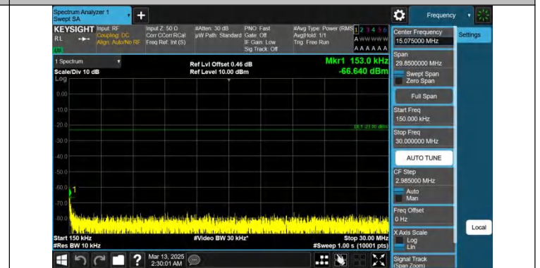
Band26(824-849)-3MHz-QPSK-27025-1RB#0-0.15~30-PASS
