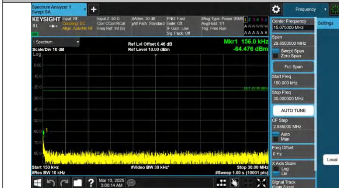
Band26(824-849)-15MHz-QPSK-26915-1RB#74-0.15~30-PASS
