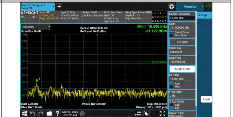
Band26(824-849)-3MHz-QPSK-26805-1RB#14-0.009~0.15-PASS
