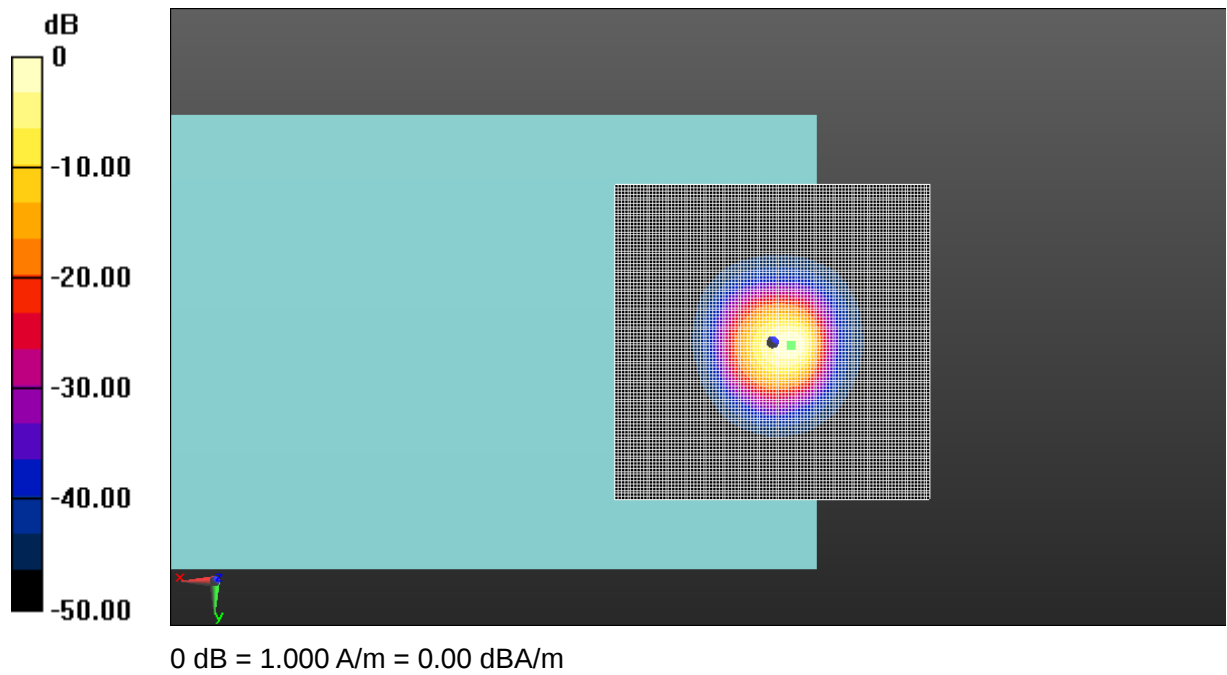
Fig A.21 T-Coil LTE-Band 25
