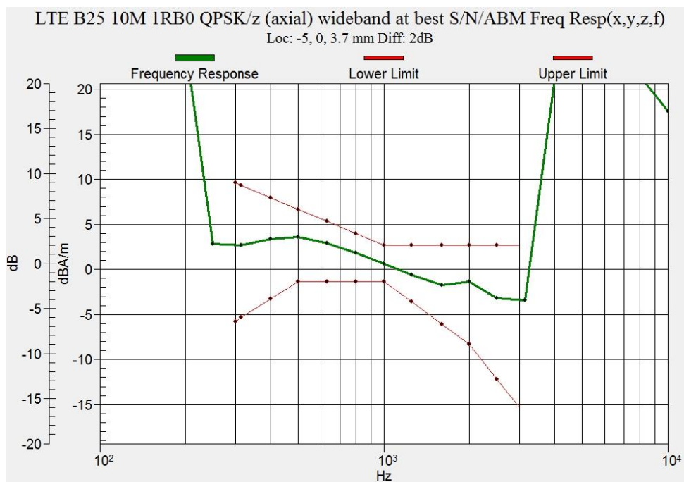
Figure B.11 Frequency Response of LTE-Band 25
