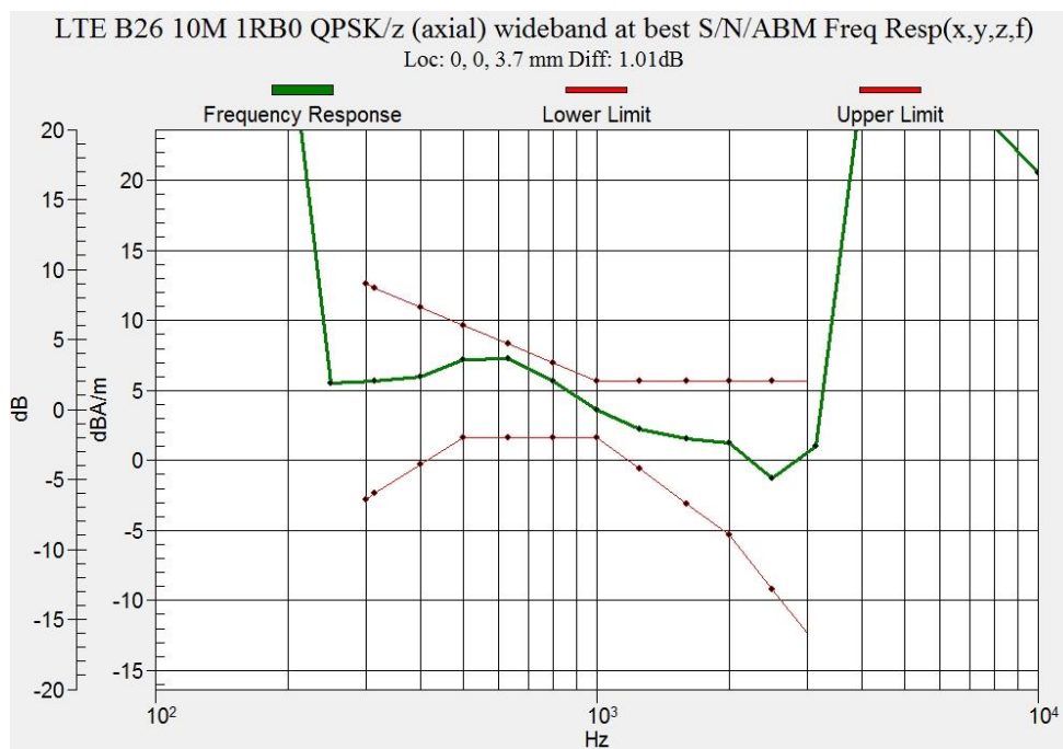
Figure B.12 Frequency Response of LTE-Band 26
