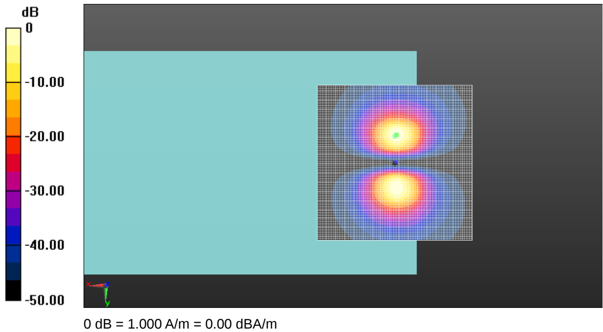
Fig A.26 T-Coil LTE-Band 41
