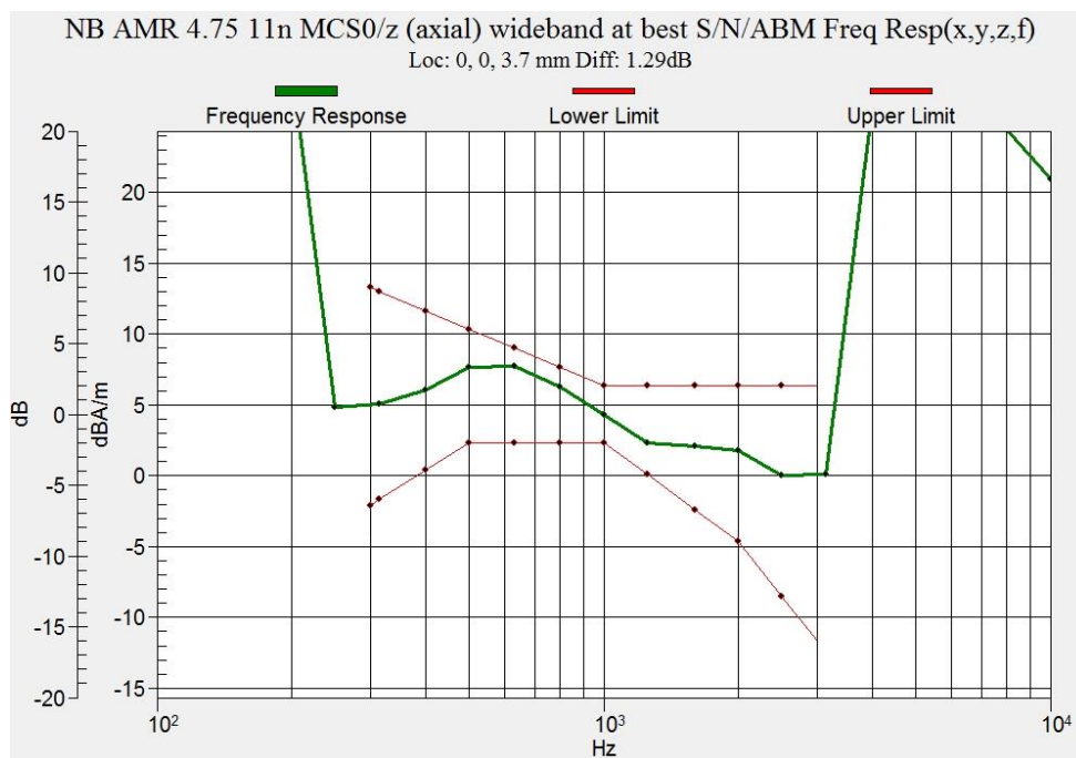
Figure B.14 Frequency Response of WIFI 2.4G
