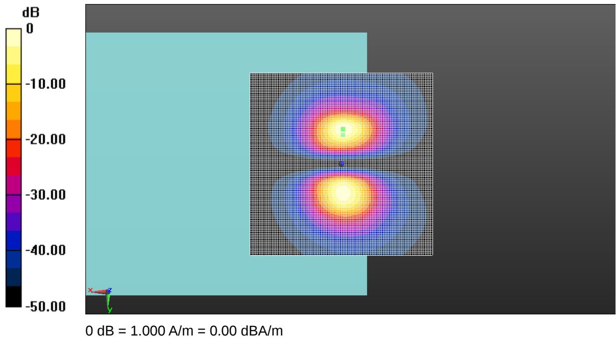
Fig A.2 T-Coil GSM 850
