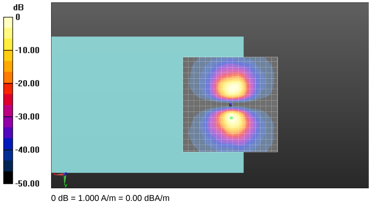
Fig A.10 T-Coil CDMA BC10
