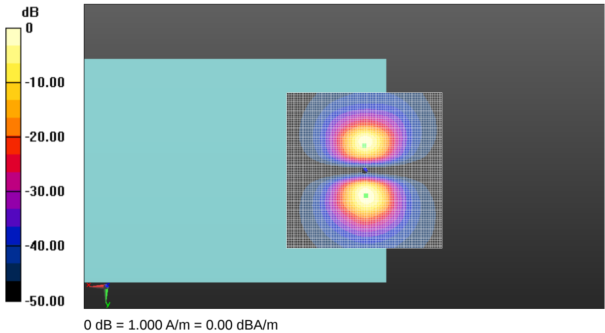
Fig A.22 T-Coil LTE-Band 25
