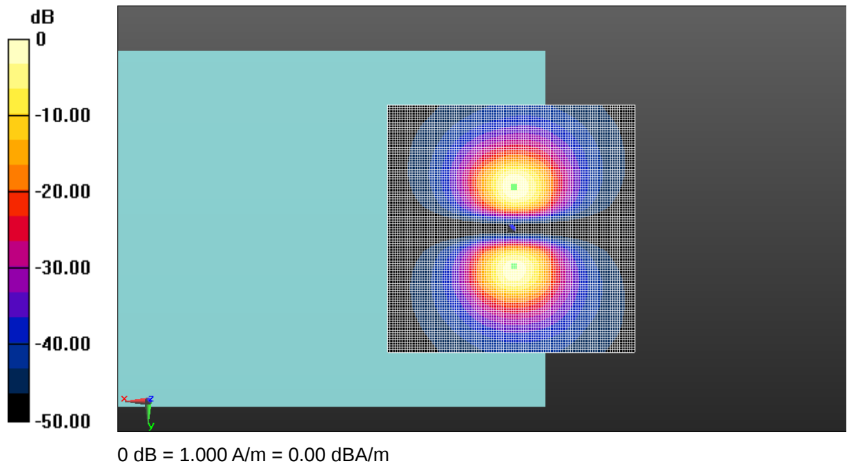
Fig A.4 T-Coil GSM 1900
