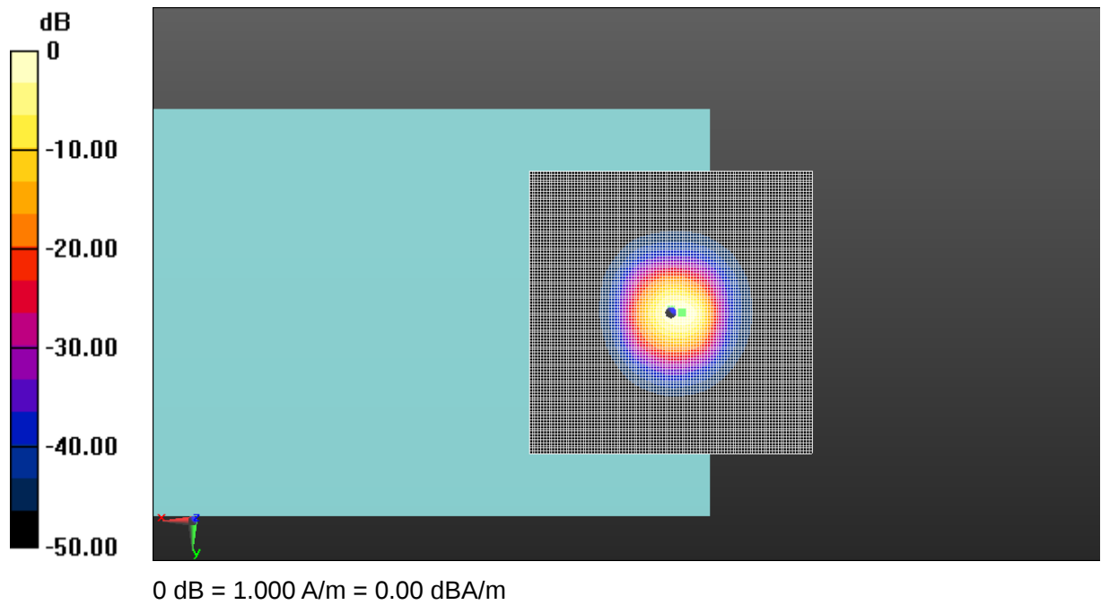
Fig A.13 T-Coil LTE-Band 4
