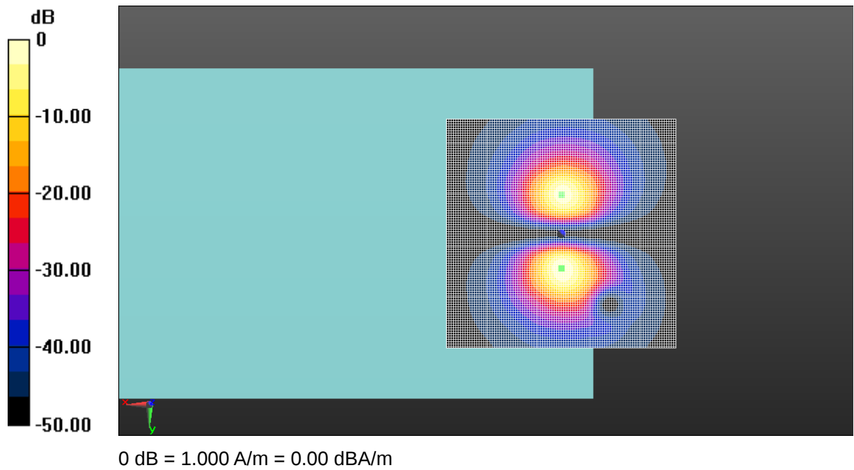
Fig A.24 T-Coil LTE-Band 26
