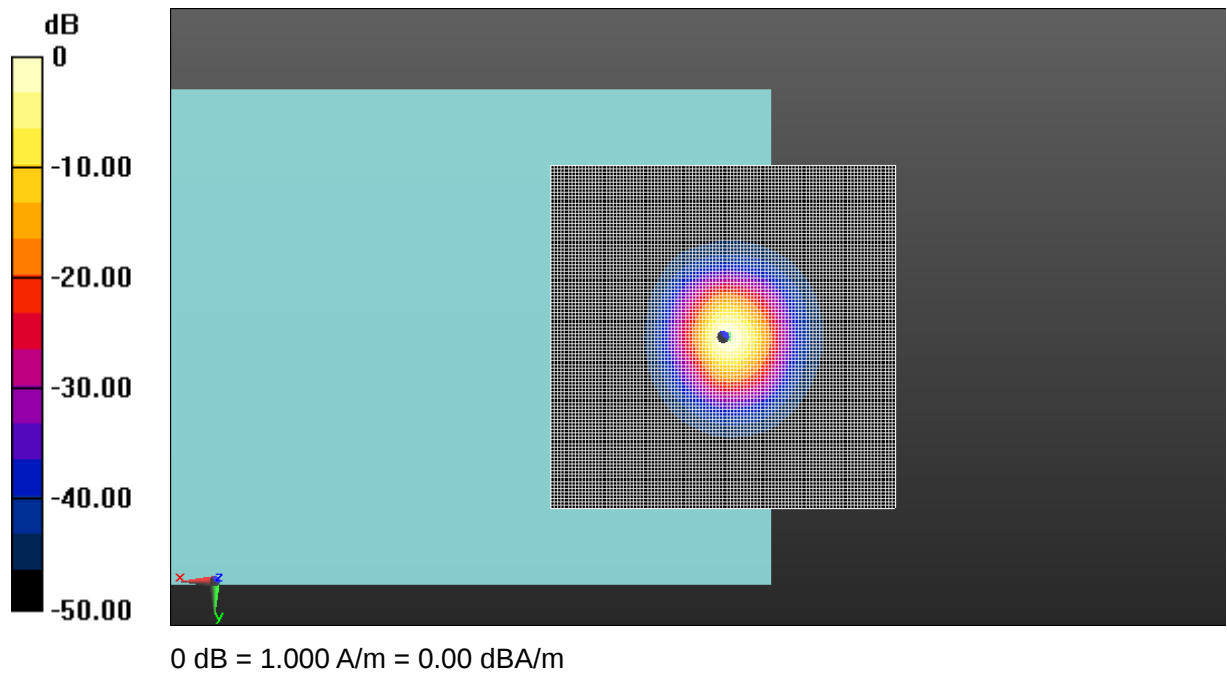
Fig A.1 T-Coil GSM 850
