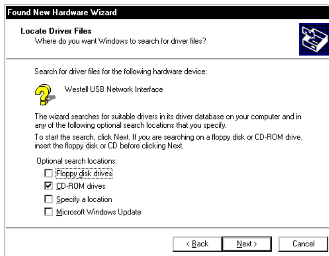
Figure 24. Windows 2000
