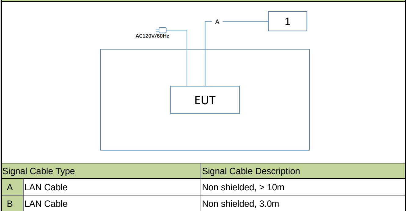
Connection Diagram – Radiated Emission testing (CDD mode) & AC Conducted Emissions
