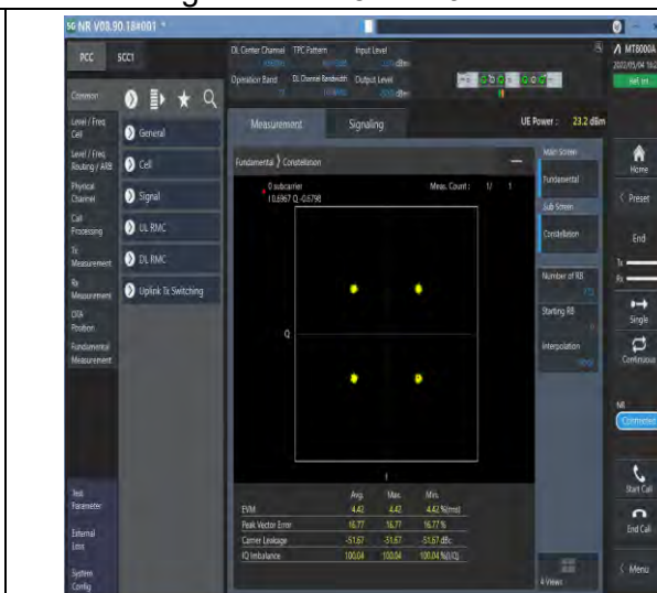
1-N77-3700-3980-PC2-30-100-M-6-CP-QPSK-Outer _Full-273@0-Ant1-see graph-PASS
