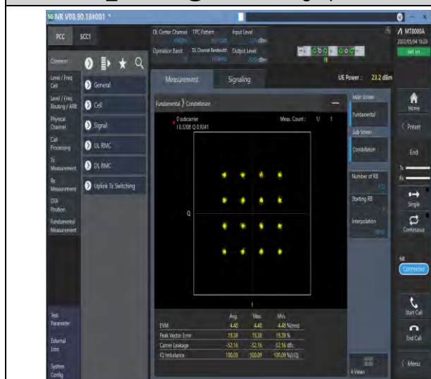
1-N77-3700-3980-PC2-30-100-M-7-CP-16QAM-Outer r_Full-273@0-Ant1-see graph-PASS
