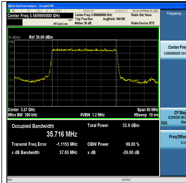
NTNV-n48-PC3-30-40-L-DFT-BPSK-Outer_Full-Ant1- PASS
