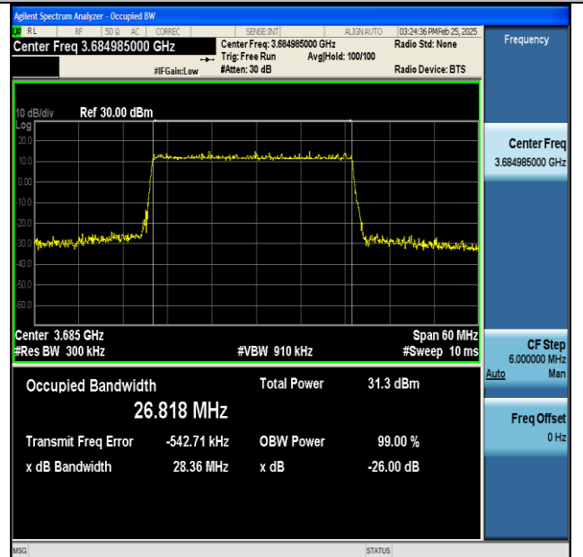
NTNV-n48-PC3-30-30-H-DFT-256QAM-Outer_Full-Ant1- PASS
