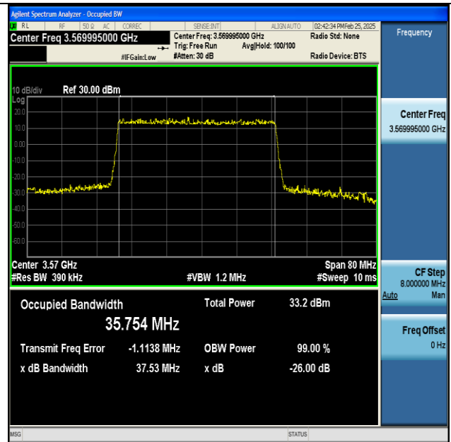
NTNV-n48-PC3-30-40-L-DFT-QPSK-Outer_Full-Ant1- PASS
