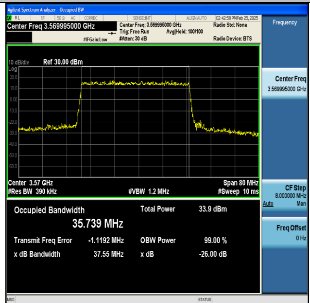
NTNV-n48-PC3-30-40-L-DFT-64QAM-Outer_Full-Ant1- PASS
