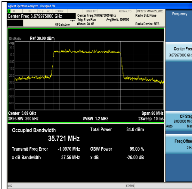
NTNV-n48-PC3-30-40-H-DFT-16QAM-Outer_Full-Ant1- PASS
