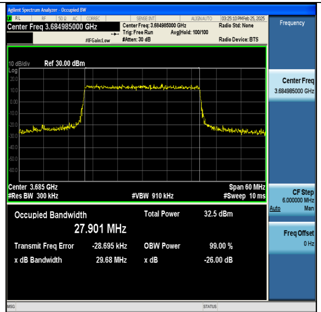
NTNV-n48-PC3-30-30-H-CP-16QAM-Outer_Full-Ant1-PASS
