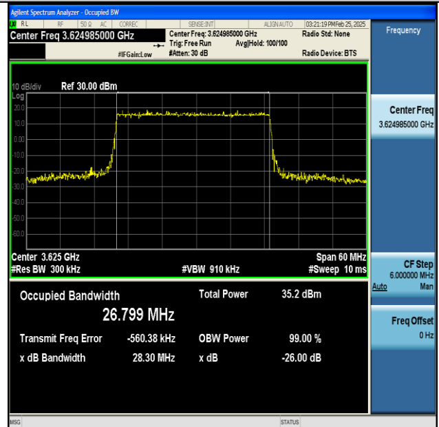
NTNV-n48-PC3-30-30-M-DFT-QPSK-Outer_Full-Ant1- PASS
