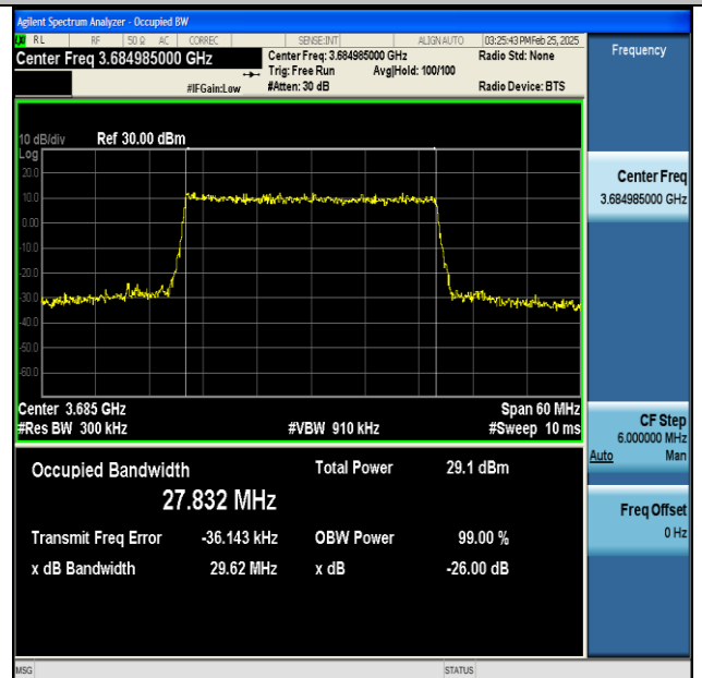
NTNV-n48-PC3-30-30-H-CP-256QAM-Outer_Full-Ant1-PASS
