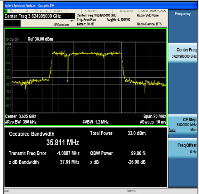
NTNV-n48-PC3-30-40-M-DFT-16QAM-Outer_Full-Ant1- PASS
