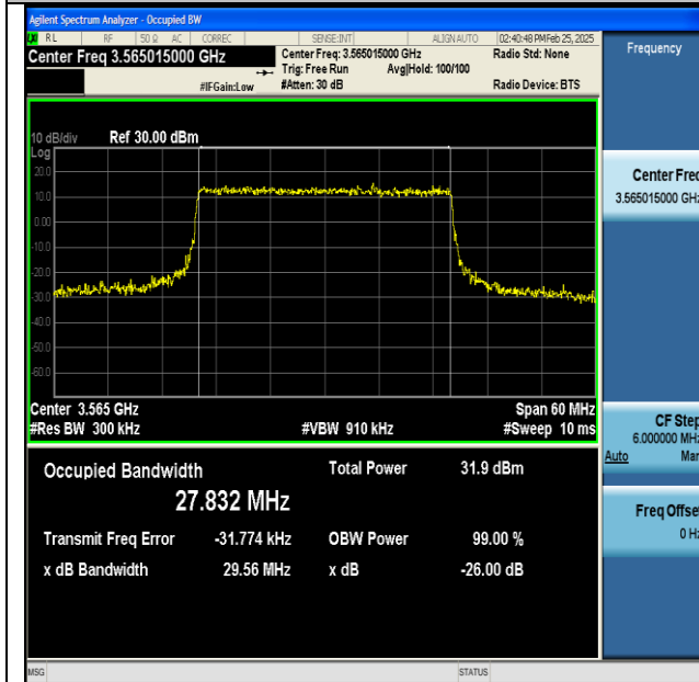
NTNV-n48-PC3-30-30-L-DFT-64QAM-Outer_Full-Ant1- PASS
