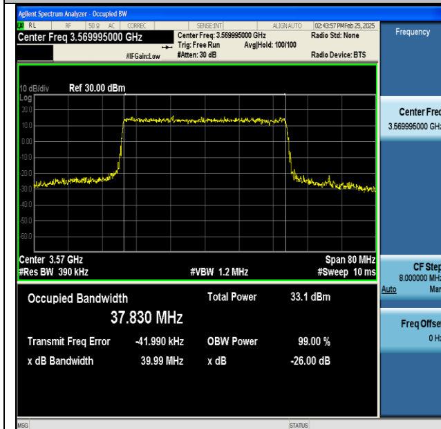
NTNV-n48-PC3-30-40-L-CP-16QAM-Outer_Full-Ant1-PASS
