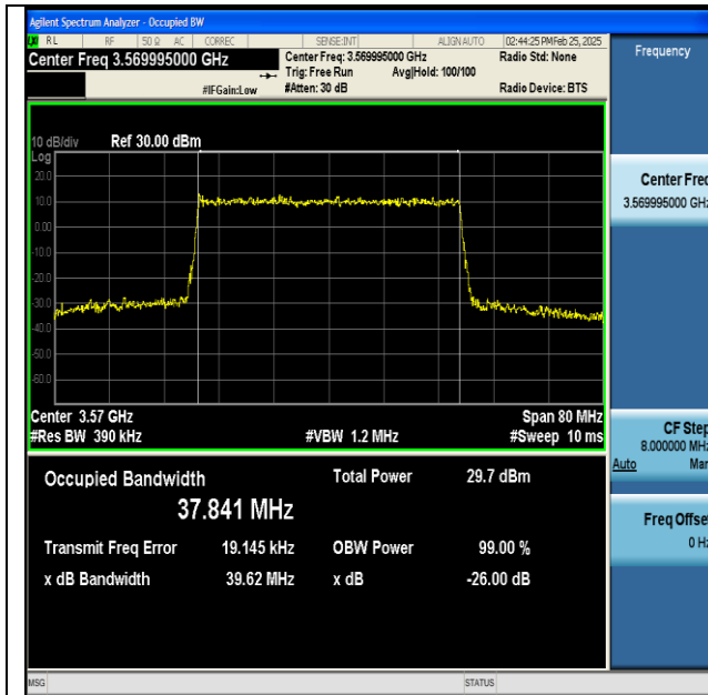
NTNV-n48-PC3-30-40-L-CP-256QAM-Outer_Full-Ant1- PASS
