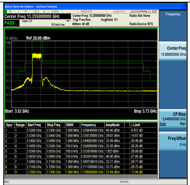
NTNV-n48-PC3-30-15-L-DFT-BPSK-Outer_Full-PASS
