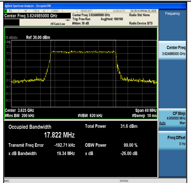
NTNV-n48-PC3-30-20-M-DFT-256QAM-Outet_Full-Ant1- PASS
