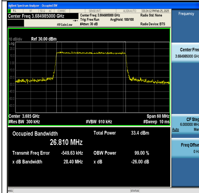
NTNV-n48-PC3-30-30-H-DFT-64QAM-Outer_Full-Ant1- PASS
