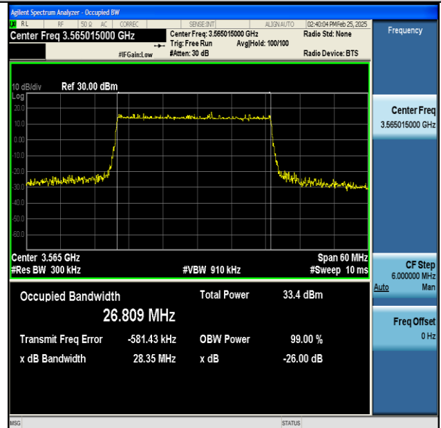
NTNV-n48-PC3-30-30-L-DFT-16QAM-Outer_Full-Ant1- PASS
