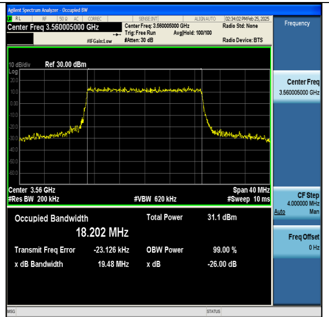
NTNV-n48-PC3-30-20-L-CP-64QAM-Outer_Full-Ant1- PASS
