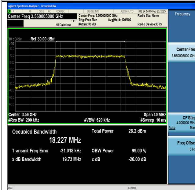
NTNV-n48-PC3-30-20-L-CP-256QAM-Outer_Full-Ant1- PASS
