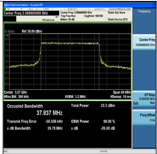
NTNV-n48-PC3-30-40-L-CP-QPSK-Outer_Full-Ant1-PASS
