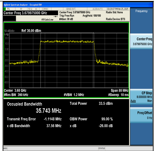
NTNV-n48-PC3-30-40-H-DFT-64QAM-Outer_Full-Ant1- PASS
