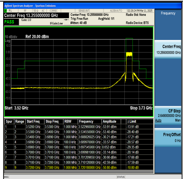
NTNV-n48-PC3-30-10-H-CP-QPSK-Outer_Full-PASS
