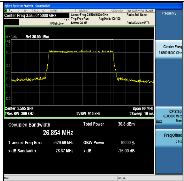
NTNV-n48-PC3-30-30-L-DFT-256QAM-Outer_Full-Ant1- PASS
