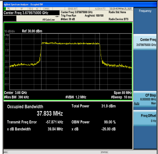
NTNV-n48-PC3-30-40-H-DFT-64QAM-Outer_Full-Ant1- PASS
