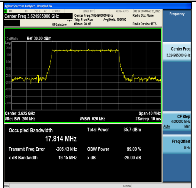
NTNV-n48-PC3-30-20-M-DFT-BPSK-Outer_Full-Ant1- PASS
