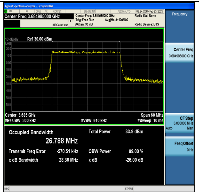
NTNV-n48-PC3-30-30-H-DFT-16QAM-Outer_Full-Ant1- PASS
