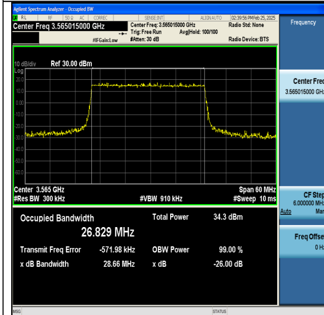
NTNV-n48-PC3-30-30-L-DFT-QPSK-Outer_Full-Ant1- PASS
