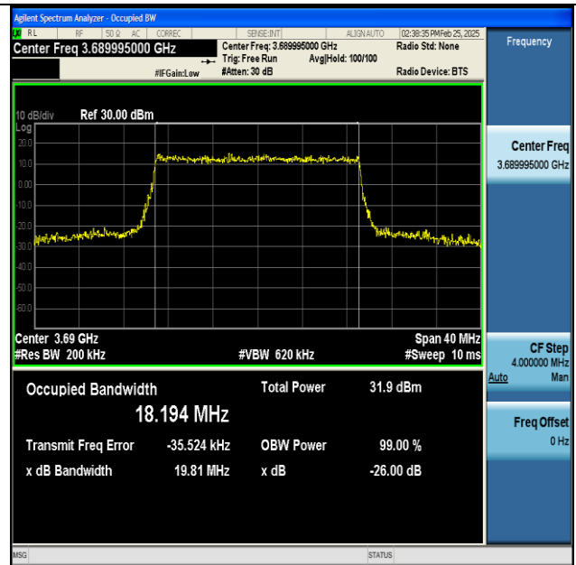
NTNV-n48-PC3-30-20-H-CP-QPSK-Outer_Full-Ant1-PASS
