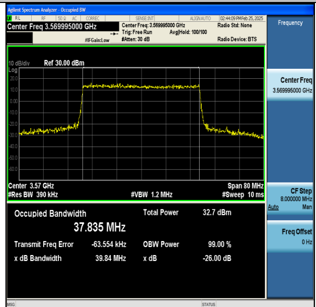
NTNV-n48-PC3-30-40-L-CP-64QAM-Outer_Full-Ant1-PASS
