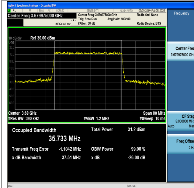
NTNV-n48-PC3-30-40-H-DFT-256QAM-Outer_Full-Ant1- PASS
