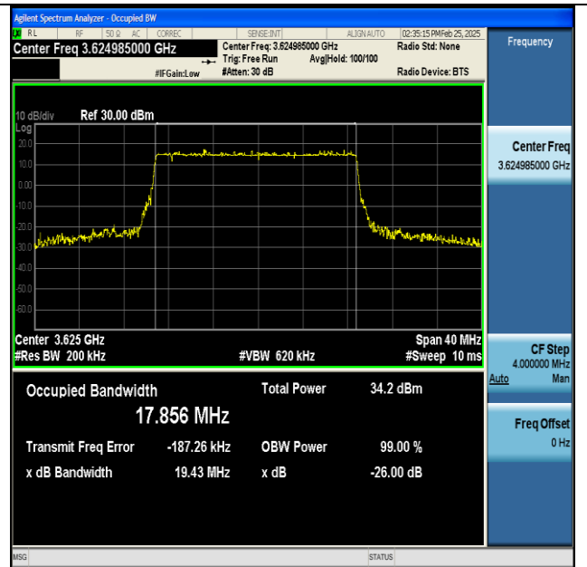
NTNV-n48-PC3-30-20-M-DFT-16QAM-Outet_Full-Ant1- PASS
