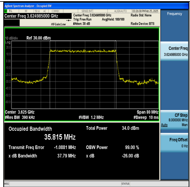
NTNV-n48-PC3-30-40-M-DFT-BPSK-Outer_Full-Ant1- PASS
