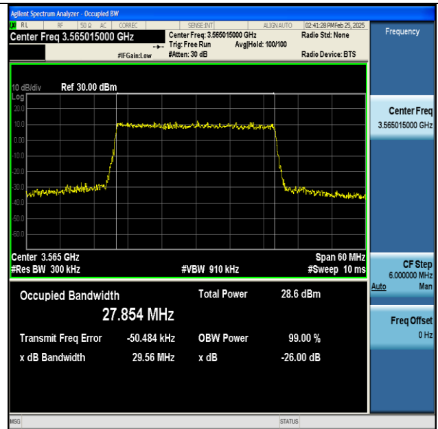
NTNV-n48-PC3-30-30-L-CP-256QAM-Outer_Full-Ant1- PASS
