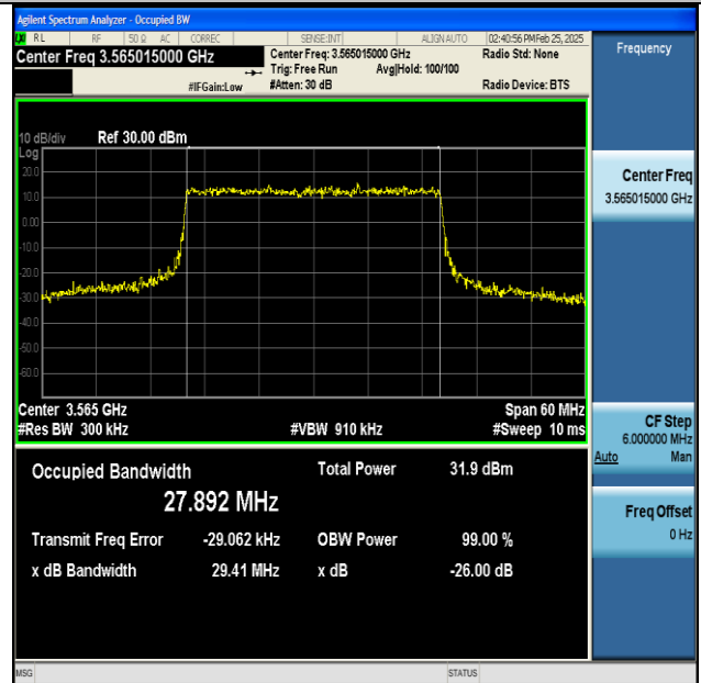
NTNV-n48-PC3-30-30-L-CP-16QAM-Outer_Full-Ant1- PASS
