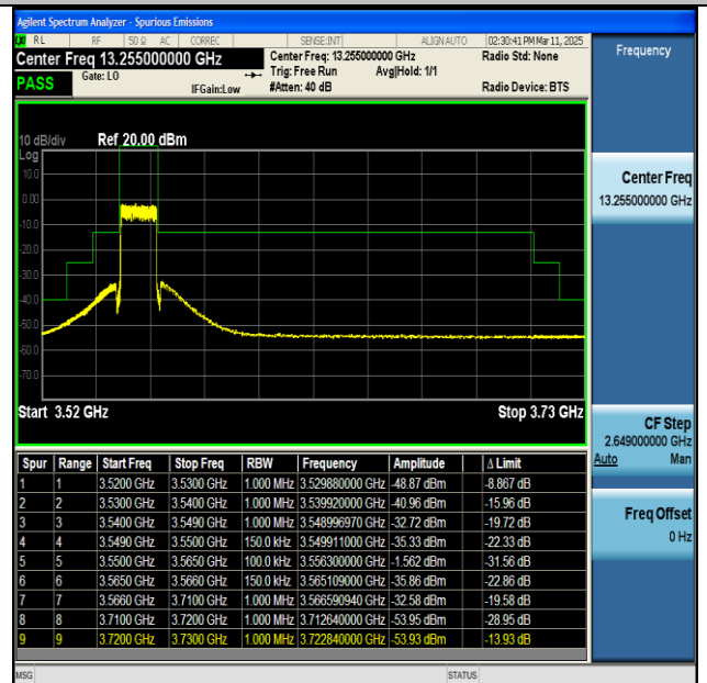
NTNV-n48-PC3-30-15-L-CP-QPSK-Outer_Full-PASS
