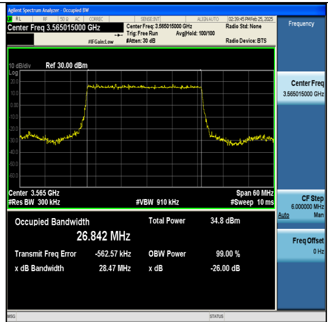
NTNV-n48-PC3-30-30-L-DFT-BPSK-Outer_Full-Ant1- PASS
