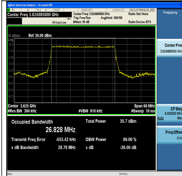
NTNV-n48-PC3-30-30-M-DFT-BPSK-Outer_Full-Ant1- PASS
