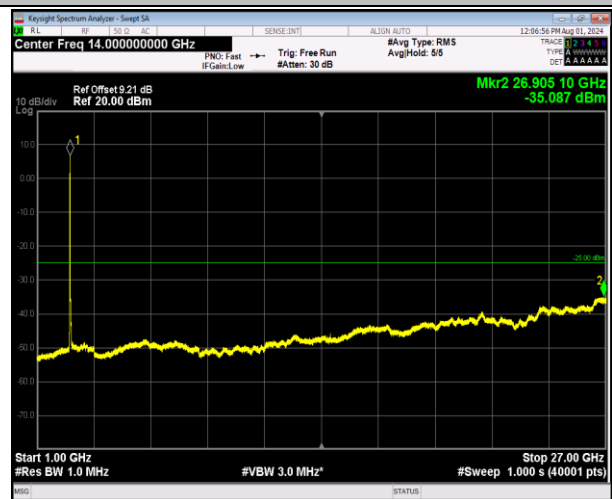
7-7-20MHz-10MHz-64QAM-64QAM-20850-20994-100RB#0 -50RB#0-1000~27000MHz-PASS
