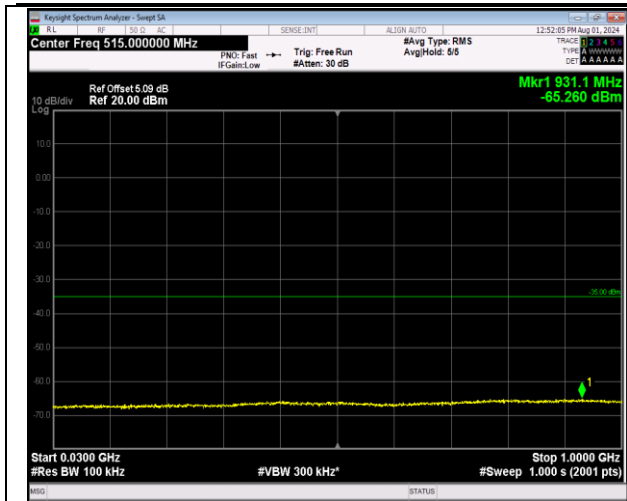
7-7-20MHz-20MHz-64QAM-64QAM-20850-21048-1RB#0 -1RB#99-30~1000MHz-PASS
