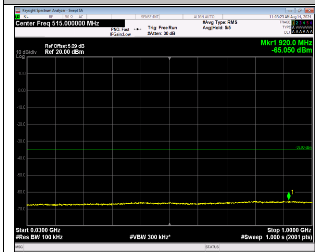
7-7-20MHz-20MHz-QPSK-QPSK-20850-21048-1RB#0-1 RB#99-30~1000MHz-PASS
