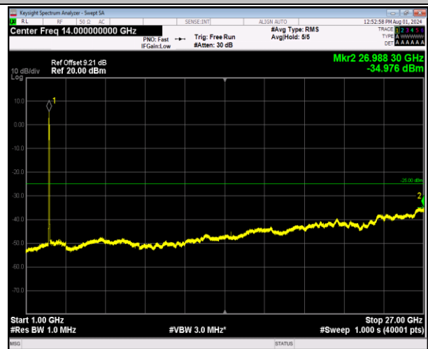
7-7-20MHz-20MHz-64QAM-64QAM-20850-21048-100RB#0- -100RB#0-1000~27000MHz-PASS
