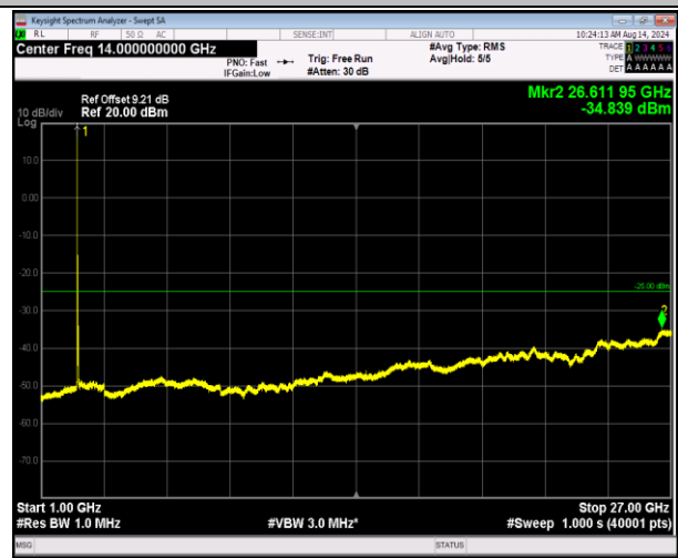
7-7-20MHz-10MHz-16QAM-16QAM-20850-20994-1RB#0-0 RB#0-1000~27000MHz-PASS
