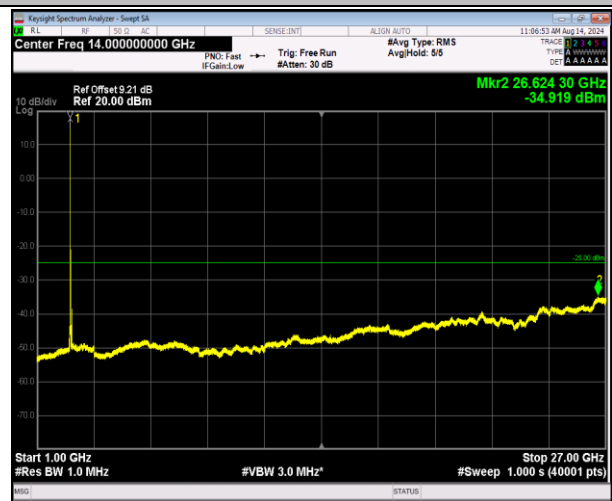
7-7-20MHz-20MHz-16QAM-16QAM-21001-21199-1RB#0-0 RB#0-1000~27000MHz-PASS
