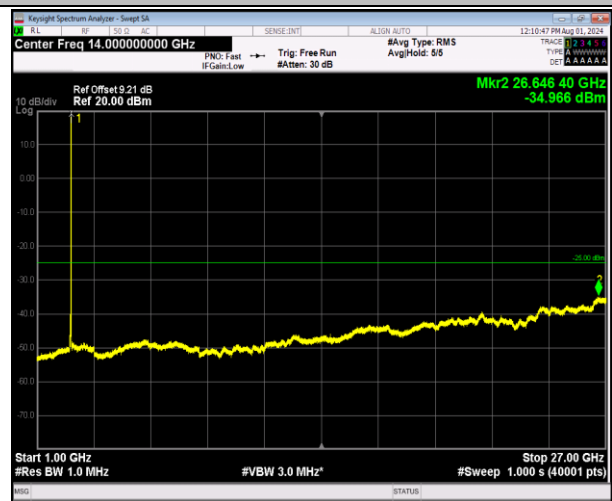
7-7-20MHz-10MHz-64QAM-64QAM-21251-21395-1RB#99- 0RB#0-1000~27000MHz-PASS
