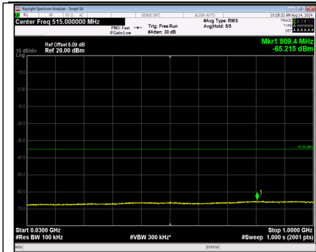
7-7-20MHz-10MHz-QPSK-QPSK-21051-21195-1RB#0-0 RB#0-30~1000MHz-PASS
