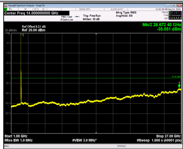
7-7-20MHz-20MHz-16QAM-16QAM-20850-21048-1RB#0-0 RB#0-1000~27000MHz-PASS
