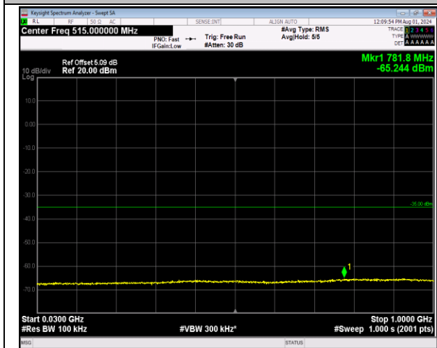
7-7-20MHz-10MHz-64QAM-64QAM-21251-21395-1RB#0 -0RB#0-30~1000MHz-PASS
