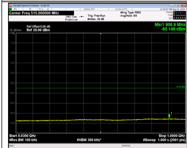
7-7-20MHz-20MHz-QPSK-QPSK-20850-21048-1RB#99-9 ORB#0-30~1000MHz-PASS
