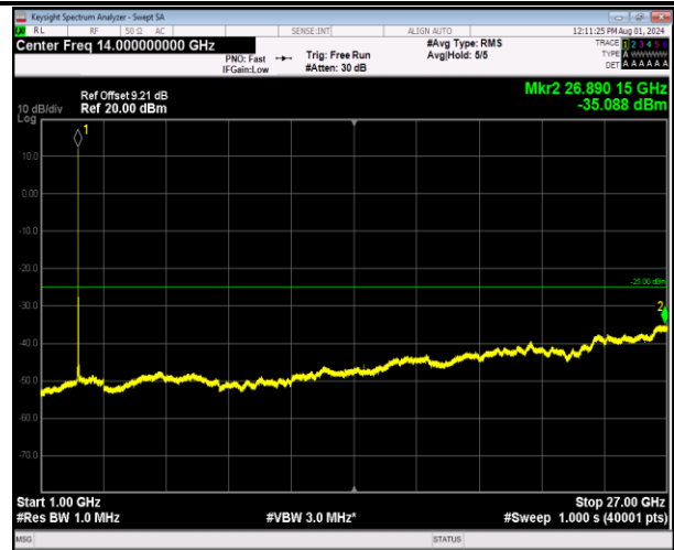
7-7-20MHz-10MHz-64QAM-64QAM-21251-21395-1RB#0-1 RB#49-1000~27000MHz-PASS
