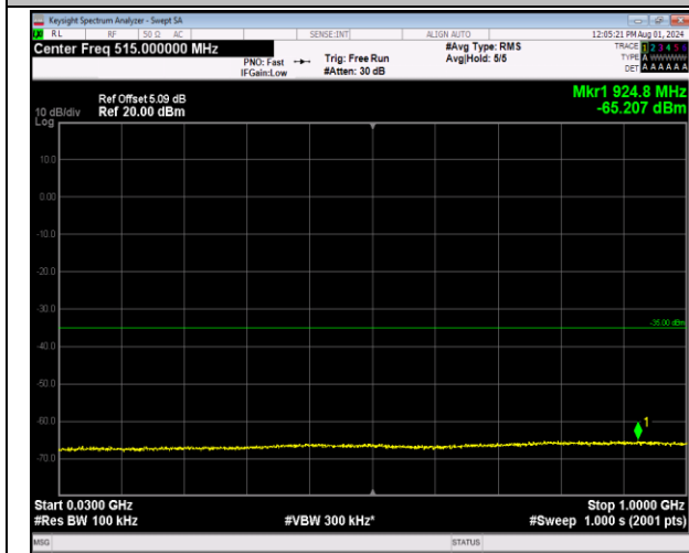
7-7-20MHz-10MHz-64QAM-64QAM-20850-20994-1RB#9 9-0RB#0-30~1000MHz-PASS
