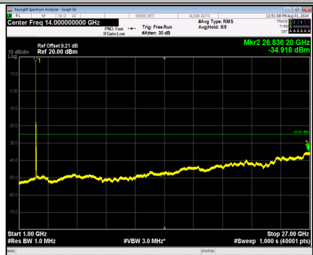
7-7-20MHz-20MHz-64QAM-64QAM-20850-21048-1RB#0-0 RB#0-1000~27000MHz-PASS
