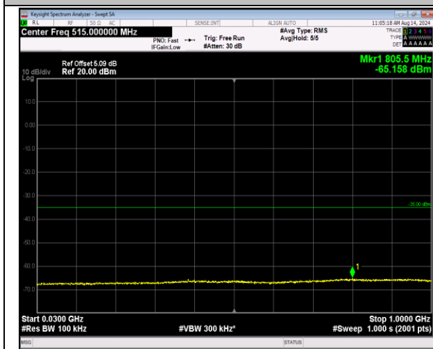
7-7-20MHz-20MHz-16QAM-16QAM-20850-21048-100RB #0-100RB#0-30~1000MHz-PASS
