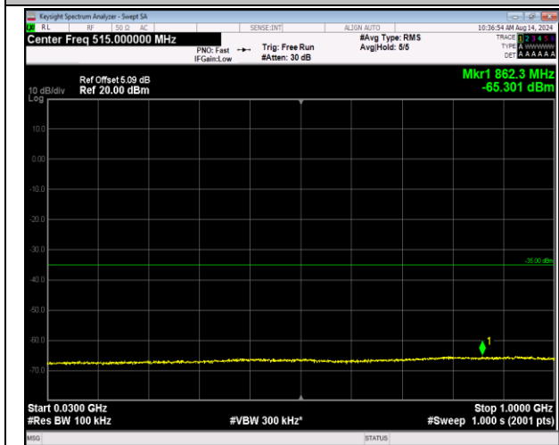
7-7-20MHz-10MHz-16QAM-16QAM-21251-21395-1RB#0 -1RB#49-30~1000MHz-PASS
