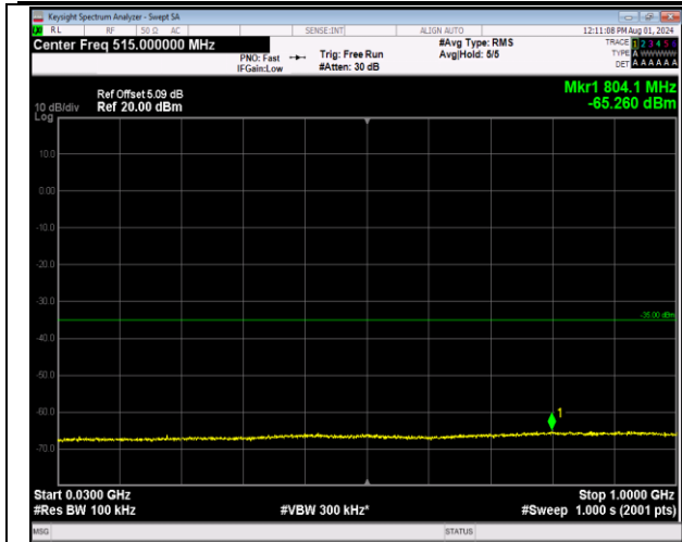
7-7-20MHz-10MHz-64QAM-64QAM-21251-21395-1RB#0 -1RB#49-30~1000MHz-PASS
