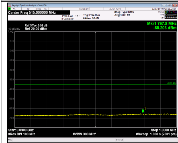
7-7-20MHz-10MHz-64QAM-64QAM-21051-21195-1RB#9 9-0RB#0-30~1000MHz-PASS
