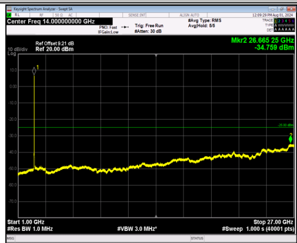
7-7-20MHz-10MHz-64QAM-64QAM-21051-21195-100RB#0 -50RB#0-1000~27000MHz-PASS
