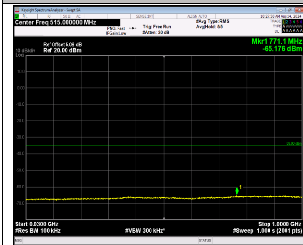
7-7-20MHz-10MHz-16QAM-16QAM-20850-20994-100RB #0-50RB#0-30~1000MHz-PASS
