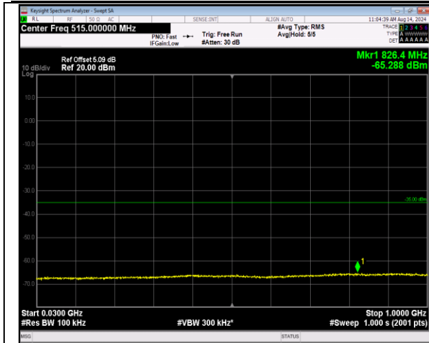
7-7-20MHz-20MHz-QPSK-QPSK-20850-21048-100RB#0 -100RB#0-30~1000MHz-PASS
