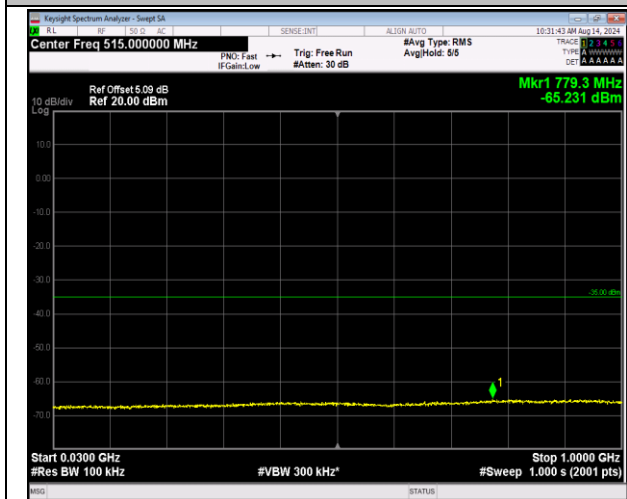
7-7-20MHz-10MHz-16QAM-16QAM-21051-21195-1RB#0 -1RB#49-30~1000MHz-PASS
