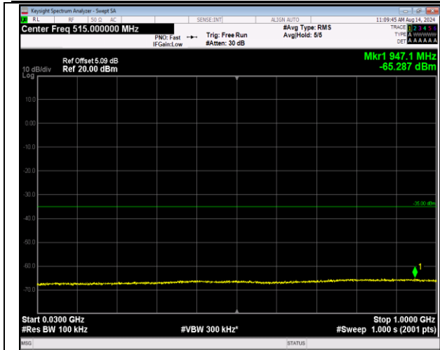
7-7-20MHz-20MHz-QPSK-QPSK-21001-21199-100RB#0 -100RB#0-30~1000MHz-PASS
