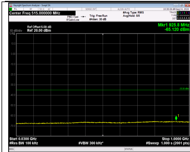
7-7-20MHz-10MHz-16QAM-16QAM-21051-21195-1RB#9 9-ORB#0-30~1000MHz-PASS
