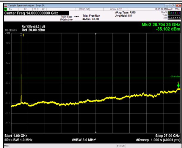
7-7-20MHz-10MHz-64QAM-64QAM-21251-21395-1RB#0-0 RB#0-1000~27000MHz-PASS
