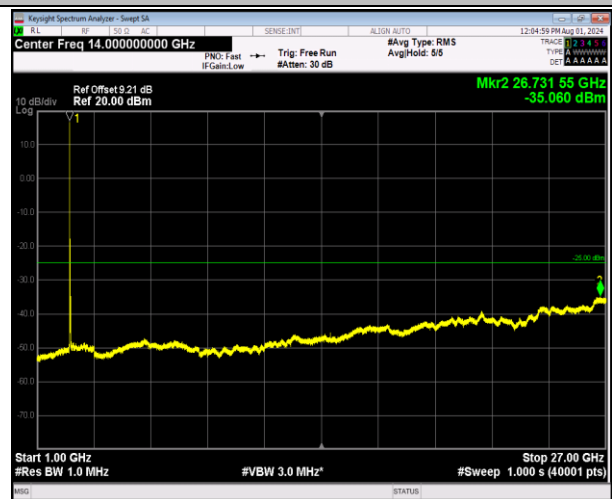
7-7-20MHz-10MHz-64QAM-64QAM-20850-20994-1RB#0-0 RB#0-1000~27000MHz-PASS
