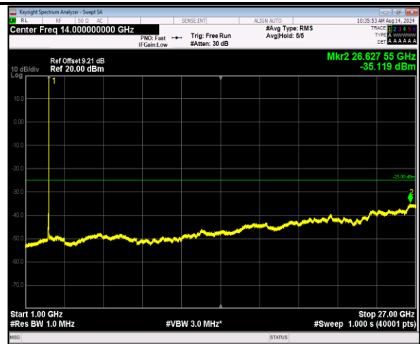
7-7-20MHz-10MHz-16QAM-16QAM-21251-21395-1RB#99- 0RB#0-1000~27000MHz-PASS
