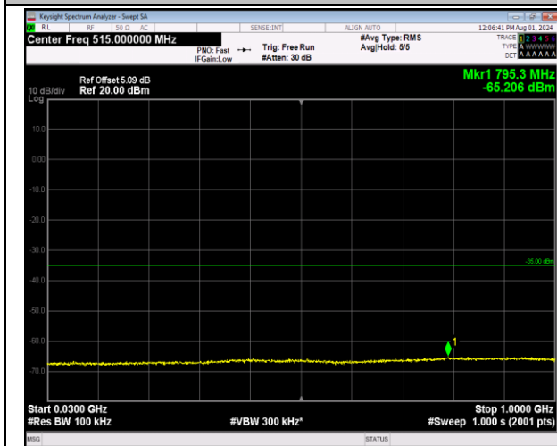
7-7-20MHz-10MHz-64QAM-64QAM-20850-20994-100RB #0-50RB#0-30~1000MHz-PASS
