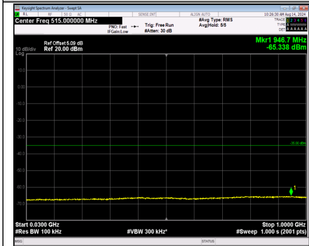
7-7-20MHz-10MHz-16QAM-16QAM-20850-20994-1RB#0 -1RB#49-30~1000MHz-PASS
