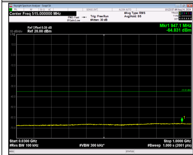
7-7-20MHz-10MHz-16QAM-16QAM-20850-20994-1RB#0 -0RB#0-30~1000MHz-PASS
