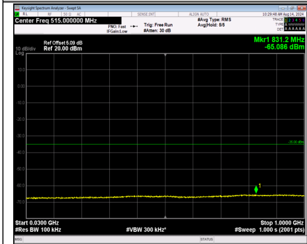
7-7-20MHz-10MHz-QPSK-QPSK-21051-21195-1RB#99-99 ORB#0-30~1000MHz-PASS
