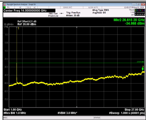
7-7-20MHz-10MHz-64QAM-64QAM-20850-20994-1RB#99- 0RB#0-1000~27000MHz-PASS
