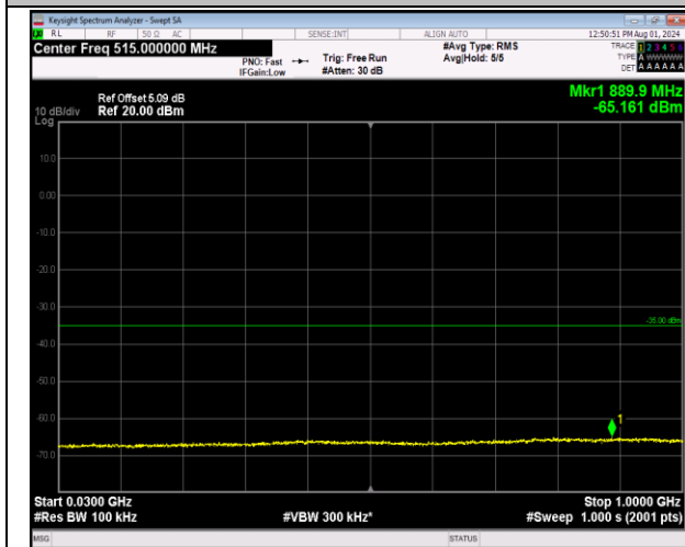
7-7-20MHz-20MHz-64QAM-64QAM-20850-21048-1RB#0 -ORB#0-30~1000MHz-PASS
