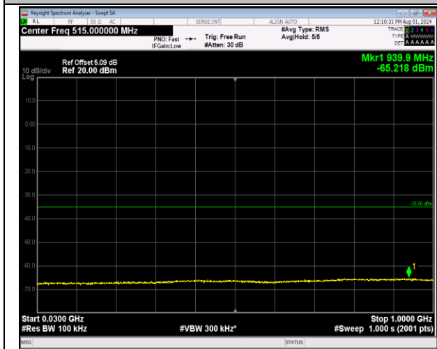
7-7-20MHz-10MHz-64QAM-64QAM-21251-21395-1RB#9 9-0RB#0-30~1000MHz-PASS
