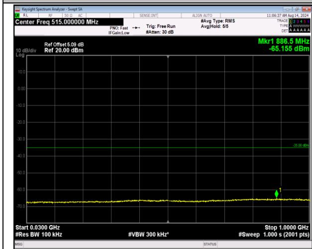
7-7-20MHz-20MHz-16QAM-16QAM-21001-21199-1RB#0 -0RB#0-30~1000MHz-PASS
