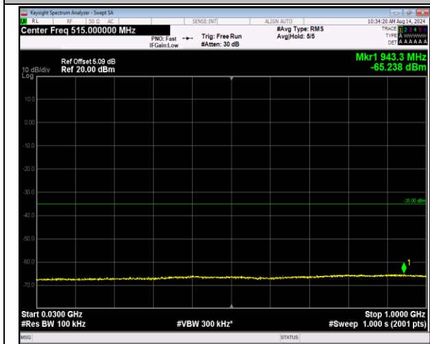
7-7-20MHz-10MHz-16QAM-16QAM-21251-21395-1RB#0 -0RB#0-30~1000MHz-PASS
