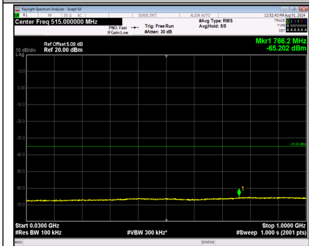
7-7-20MHz-20MHz-64QAM-64QAM-20850-21048-100RB #0-100RB#0-30~1000MHz-PASS
