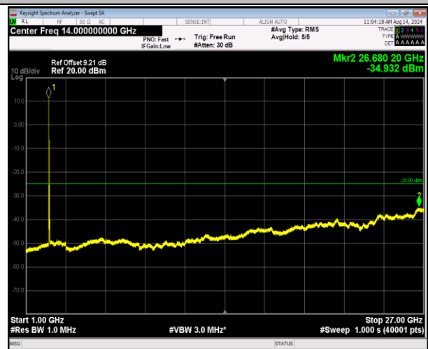
7-7-20MHz-20MHz-16QAM-16QAM-20850-21048-1RB#0-1 RB#99-1000~27000MHz-PASS
