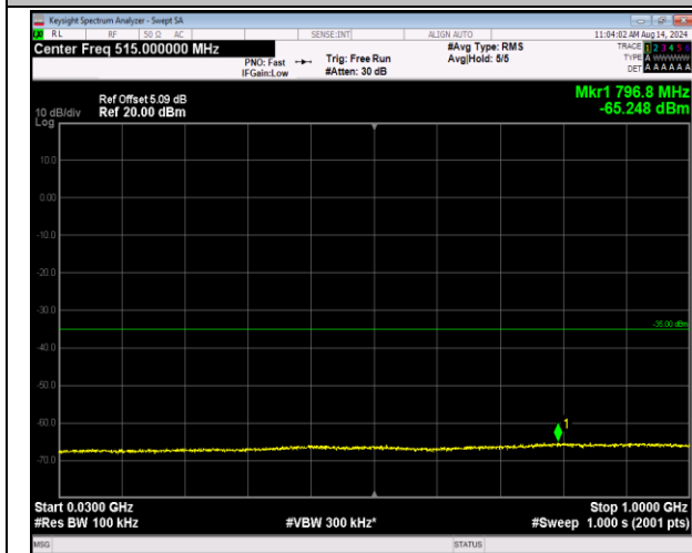
7-7-20MHz-20MHz-16QAM-16QAM-20850-21048-1RB#0 -1RB#99-30~1000MHz-PASS
