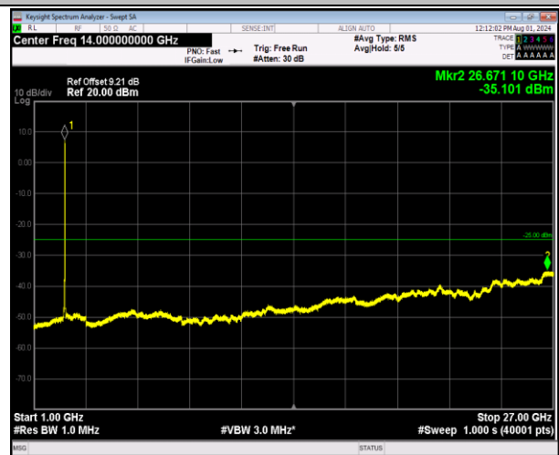
7-7-20MHz-10MHz-64QAM-64QAM-21251-21395-100RB#0 -50RB#0-1000~27000MHz-PASS
