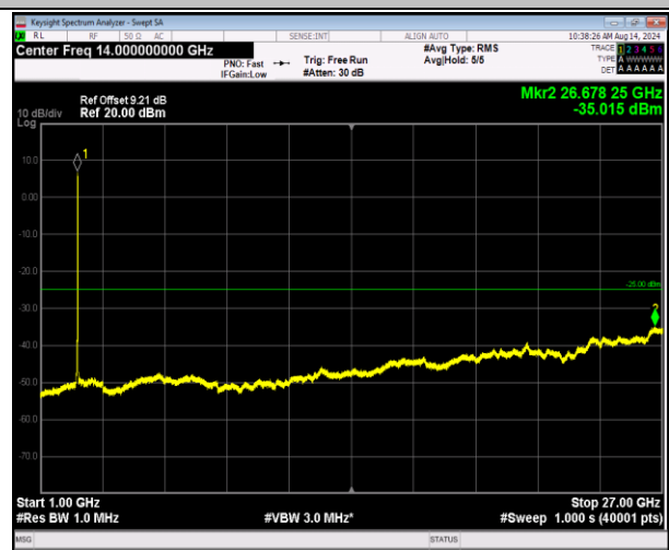
7-7-20MHz-10MHz-16QAM-16QAM-21251-21395-100RB#0 -50RB#0-1000~27000MHz-PASS
