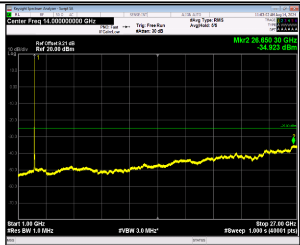
7-7-20MHz-20MHz-16QAM-16QAM-20850-21048-1RB#99- ORB#0-1000~27000MHz-PASS
