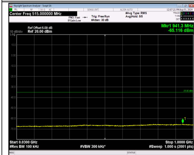
7-7-20MHz-10MHz-64QAM-64QAM-21051-21195-1RB#0 -ORB#0-30~1000MHz-PASS
