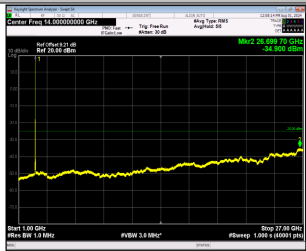
7-7-20MHz-10MHz-64QAM-64QAM-21051-21195-1RB#99- 0RB#0-1000~27000MHz-PASS
