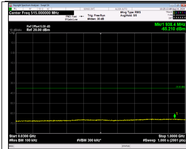
7-7-20MHz-10MHz-16QAM-16QAM-20850-20994-1RB#9 9-0RB#0-30~1000MHz-PASS
