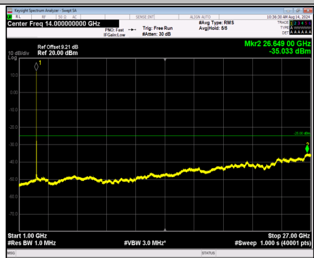
7-7-20MHz-10MHz-QPSK-QPSK-21251-21395-1RB#0-1RB #49-1000~27000MHz-PASS
