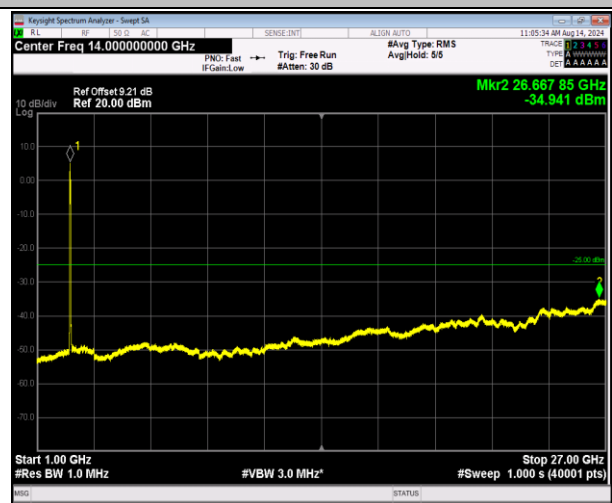
7-7-20MHz-20MHz-16QAM-16QAM-20850-21048-100RB#0 -100RB#0-1000~27000MHz-PASS
