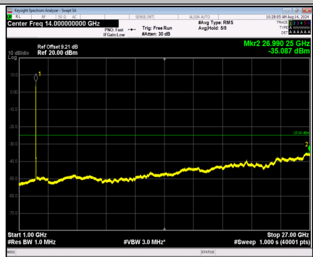
7-7-20MHz-10MHz-16QAM-16QAM-20850-20994-100RB#0 -50RB#0-1000~27000MHz-PASS
