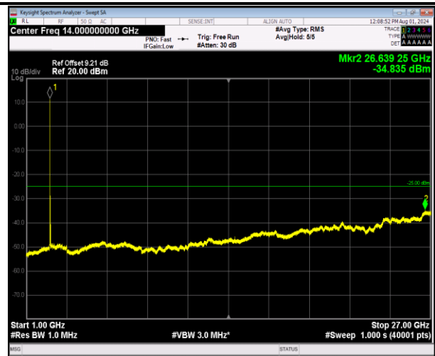
7-7-20MHz-10MHz-64QAM-64QAM-21051-21195-1RB#0-1 RB#49-1000~27000MHz-PASS
