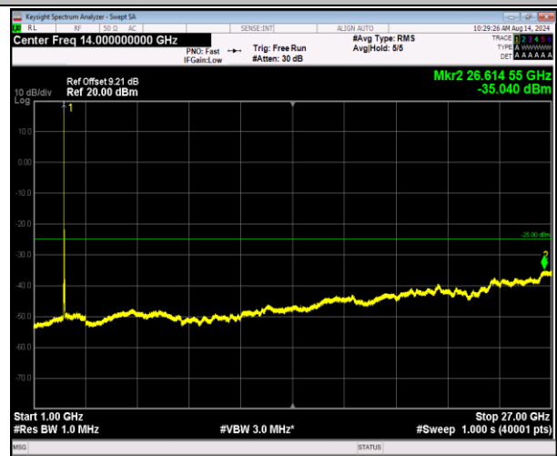
7-7-20MHz-10MHz-16QAM-16QAM-21051-21195-1RB#0-0 RB#0-1000~27000MHz-PASS
