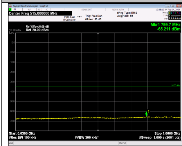
7-7-20MHz-10MHz-16QAM-16QAM-21251-21395-100RB #0-50RB#0-30~1000MHz-PASS
