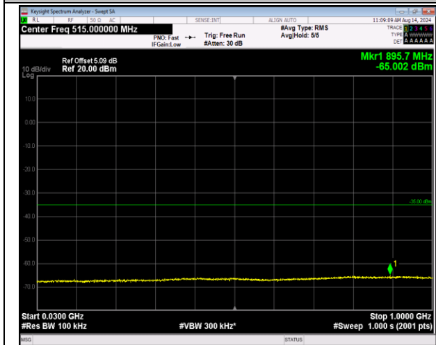
7-7-20MHz-20MHz-16QAM-16QAM-21001-21199-1RB#0 -1RB#99-30~1000MHz-PASS
