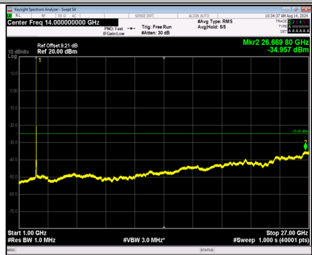
7-7-20MHz-10MHz-16QAM-16QAM-21251-21395-1RB#0-0 RB#0-1000~27000MHz-PASS
