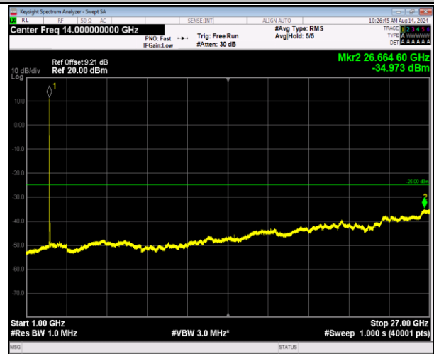
7-7-20MHz-10MHz-16QAM-16QAM-20850-20994-1RB#0-1 RB#49-1000~27000MHz-PASS
