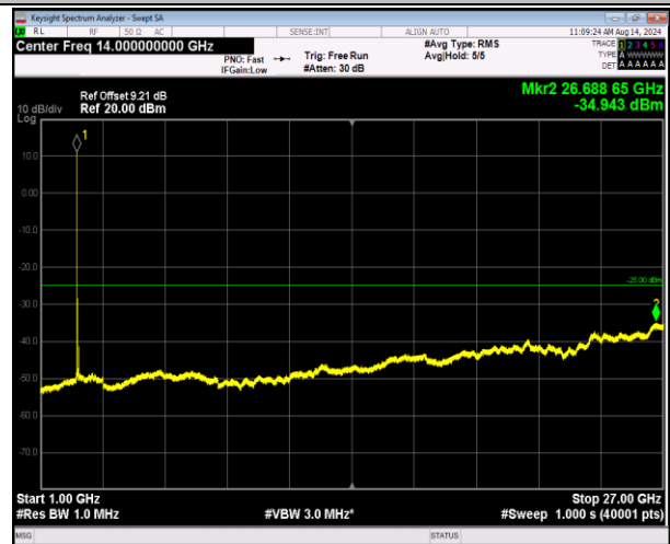
7-7-20MHz-20MHz-16QAM-16QAM-21001-21199-1RB#0-1 RB#99-1000~27000MHz-PASS
