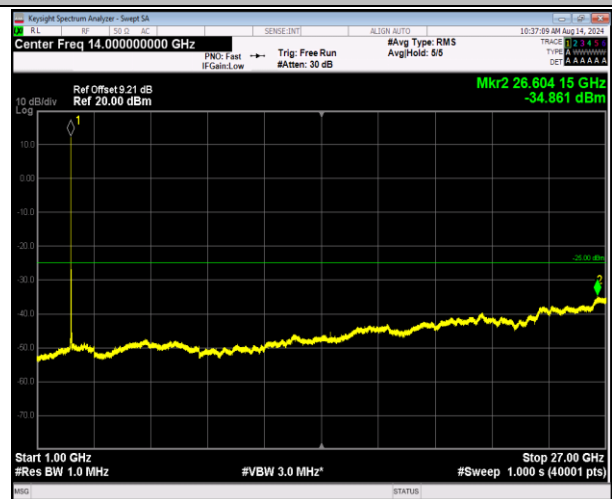
7-7-20MHz-10MHz-16QAM-16QAM-21251-21395-1RB#0-1 RB#49-1000~27000MHz-PASS
