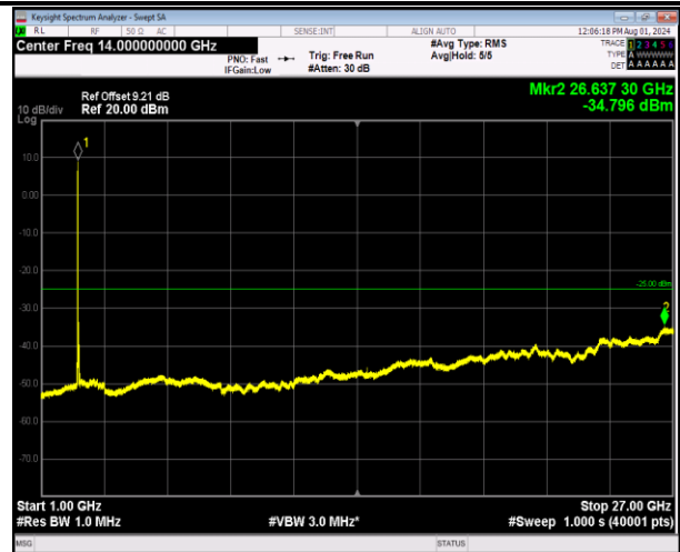
7-7-20MHz-10MHz-64QAM-64QAM-20850-20994-1RB#0-1 RB#49-1000~27000MHz-PASS
