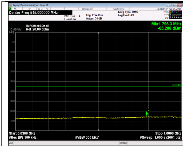
7-7-20MHz-10MHz-16QAM-16QAM-21251-21395-1RB#9 9-0RB#0-30~1000MHz-PASS
