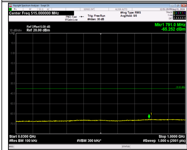
7-7-20MHz-20MHz-64QAM-64QAM-20850-21048-1RB#9 9-0RB#0-30~1000MHz-PASS
