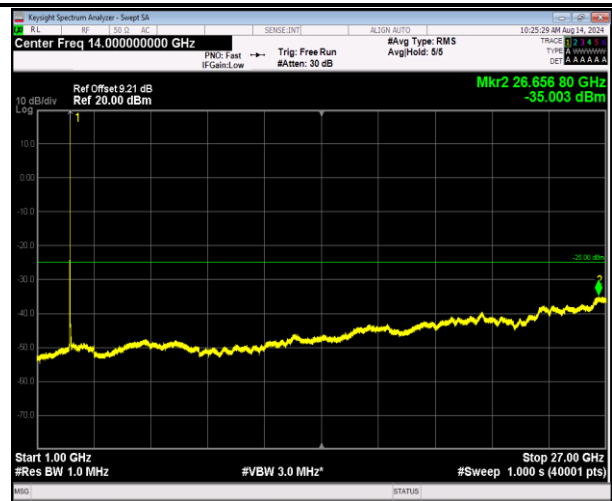
7-7-20MHz-10MHz-16QAM-16QAM-20850-20994-1RB#99- 0RB#0-1000~27000MHz-PASS
