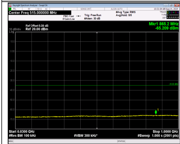
7-7-20MHz-10MHz-QPSK-QPSK-21051-21195-1RB#0-1 RB#49-30~1000MHz-PASS
