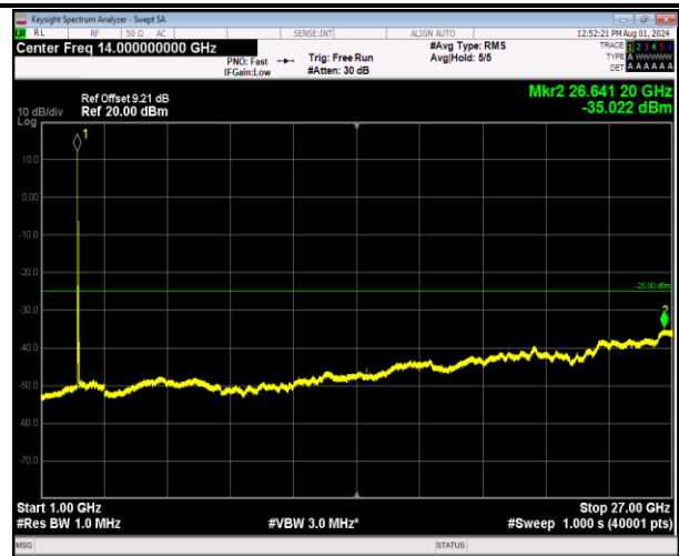
7-7-20MHz-20MHz-64QAM-64QAM-20850-21048-1RB#0-1 RB#99-1000~27000MHz-PASS
