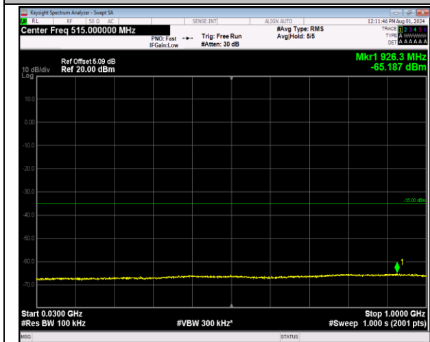
7-7-20MHz-10MHz-64QAM-64QAM-21251-21395-100RB #0-50RB#0-30~1000MHz-PASS
