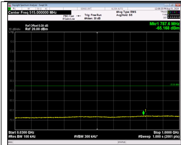
7-7-20MHz-10MHz-64QAM-64QAM-21051-21195-1RB#0 -1RB#49-30~1000MHz-PASS
