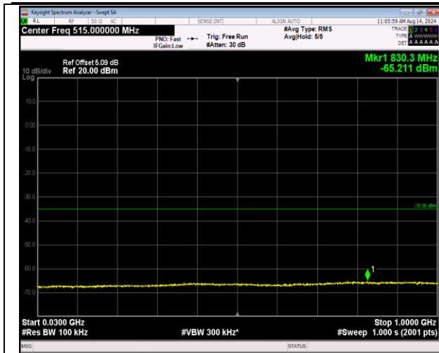
7-7-20MHz-20MHz-QPSK-QPSK-21001-21199-1RB#0-0 RB#0-30~1000MHz-PASS
