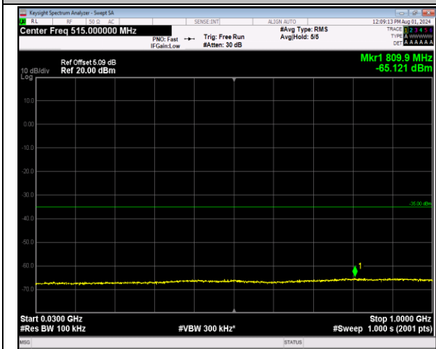
7-7-20MHz-10MHz-64QAM-64QAM-21051-21195-100RB #0-50RB#0-30~1000MHz-PASS
