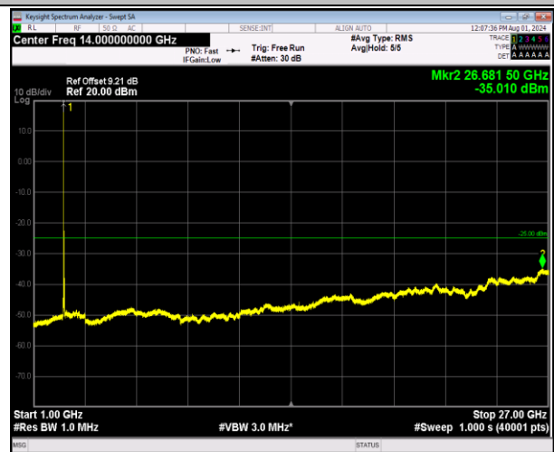
7-7-20MHz-10MHz-64QAM-64QAM-21051-21195-1RB#0-0 RB#0-1000~27000MHz-PASS
