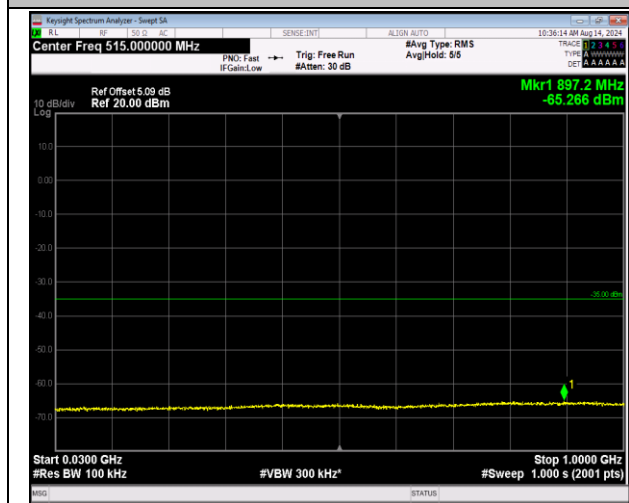
7-7-20MHz-10MHz-QPSK-QPSK-21251-21395-1RB#0-1 RB#49-30~1000MHz-PASS
