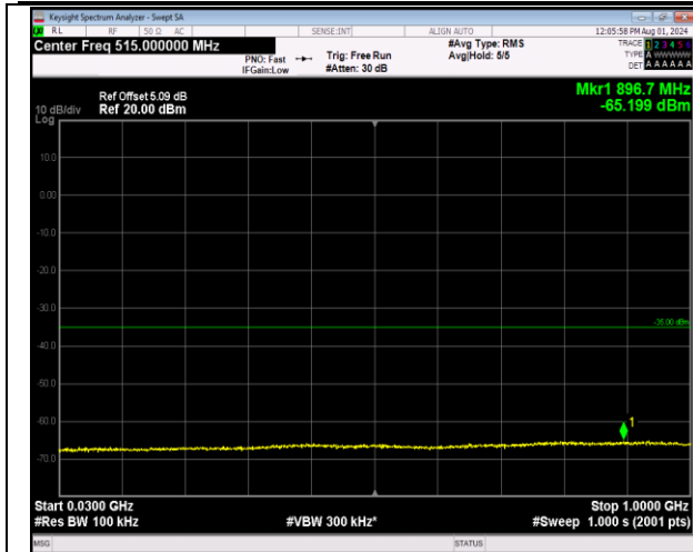
7-7-20MHz-10MHz-64QAM-64QAM-20850-20994-1RB#0 -1RB#49-30~1000MHz-PASS
