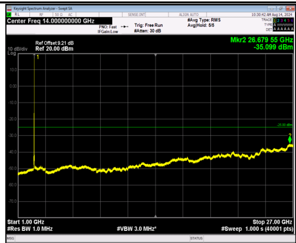
7-7-20MHz-10MHz-16QAM-16QAM-21051-21195-1RB#99- ORB#0-1000~27000MHz-PASS
