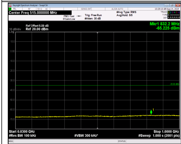
7-7-20MHz-10MHz-16QAM-16QAM-21051-21195-1RB#0 -0RB#0-30~1000MHz-PASS
