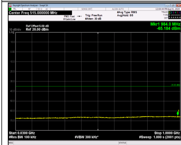
7-7-20MHz-10MHz-64QAM-64QAM-20850-20994-1RB#0 -0RB#0-30~1000MHz-PASS
