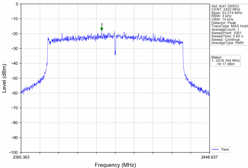
802.11ax(HEW40)_LCH_2422MHz_RU484_Left_Ant1 (SISO)_NTNV
