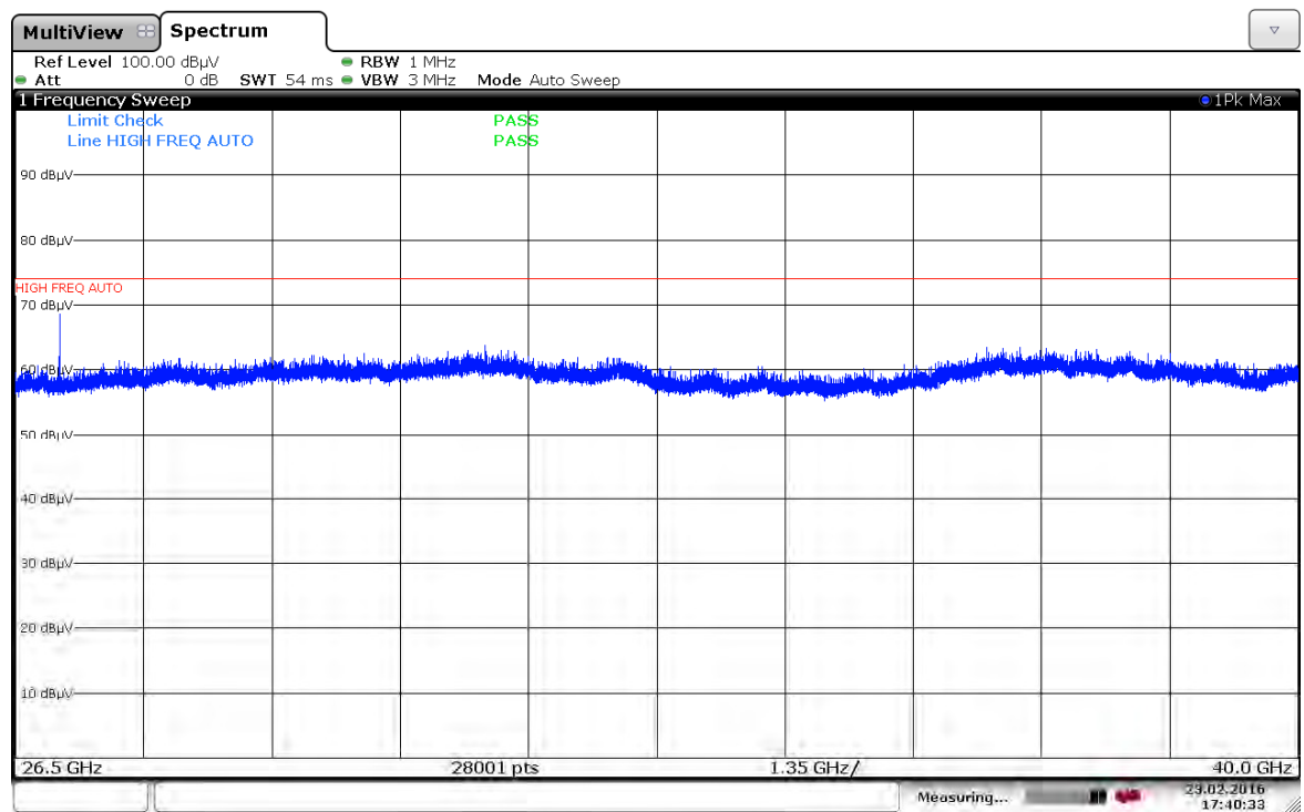
Plot 7-180. Radiated Spurious Plot > 26.5GHz (LAA (UNII Band 3, 20MHz BW), Ch. 53140)
