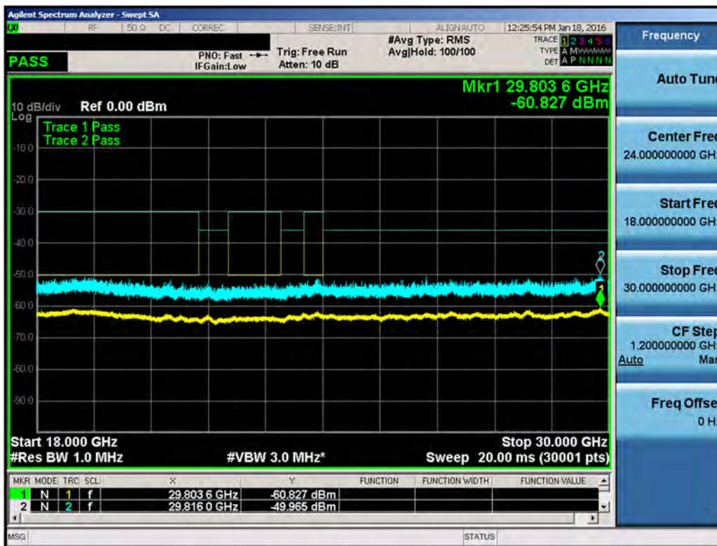
Plot 7-146. Conducted Spurious Plot (LAA (UNII Band 3, 20MHz BW) – Ch. 52740)
