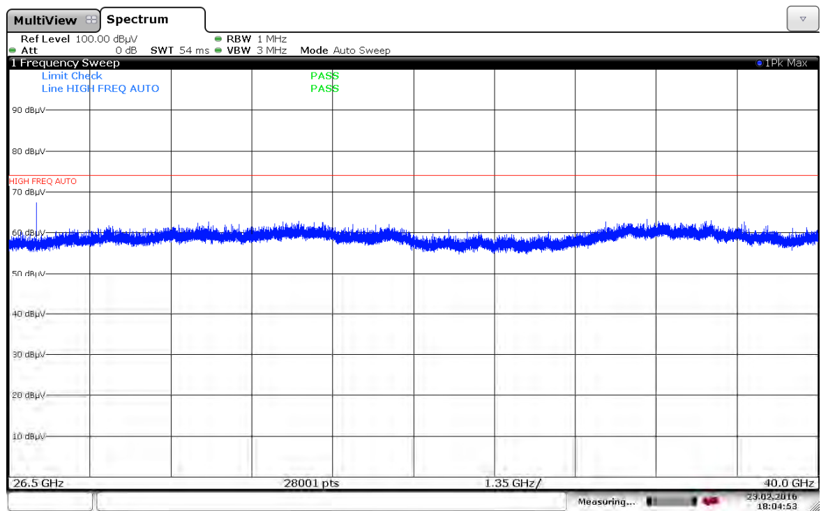
Plot 7-196. Radiated Spurious Plot > 26.5GHz (LAA (UNII Band 3, 40MHz BW), Ch. 53140, 53340)
