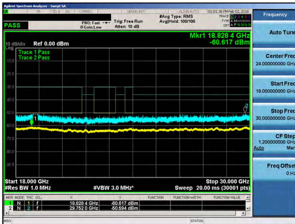
Plot 7-136. Conducted Spurious Plot (LAA (UNII Band 1, 40MHz BW) – Ch. 47290, 47490)
