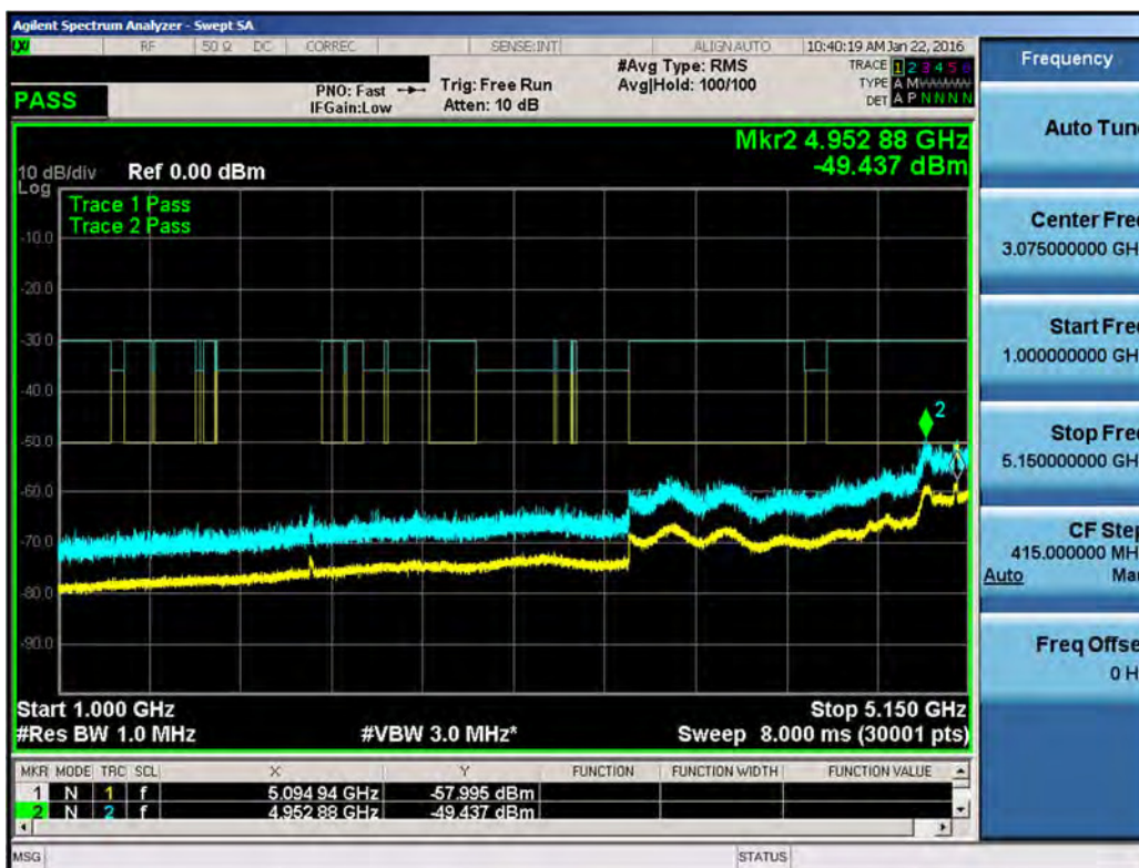
Plot 7-124. Conducted Spurious Plot (LAA (UNII Band 1, 20MHz BW) – Ch. 47690)
