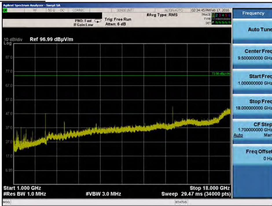
Plot 7-185. Radiated Spurious Plot > 1GHz (LAA (UNII Band 1, 20MHz BW), Ch. 47290)
