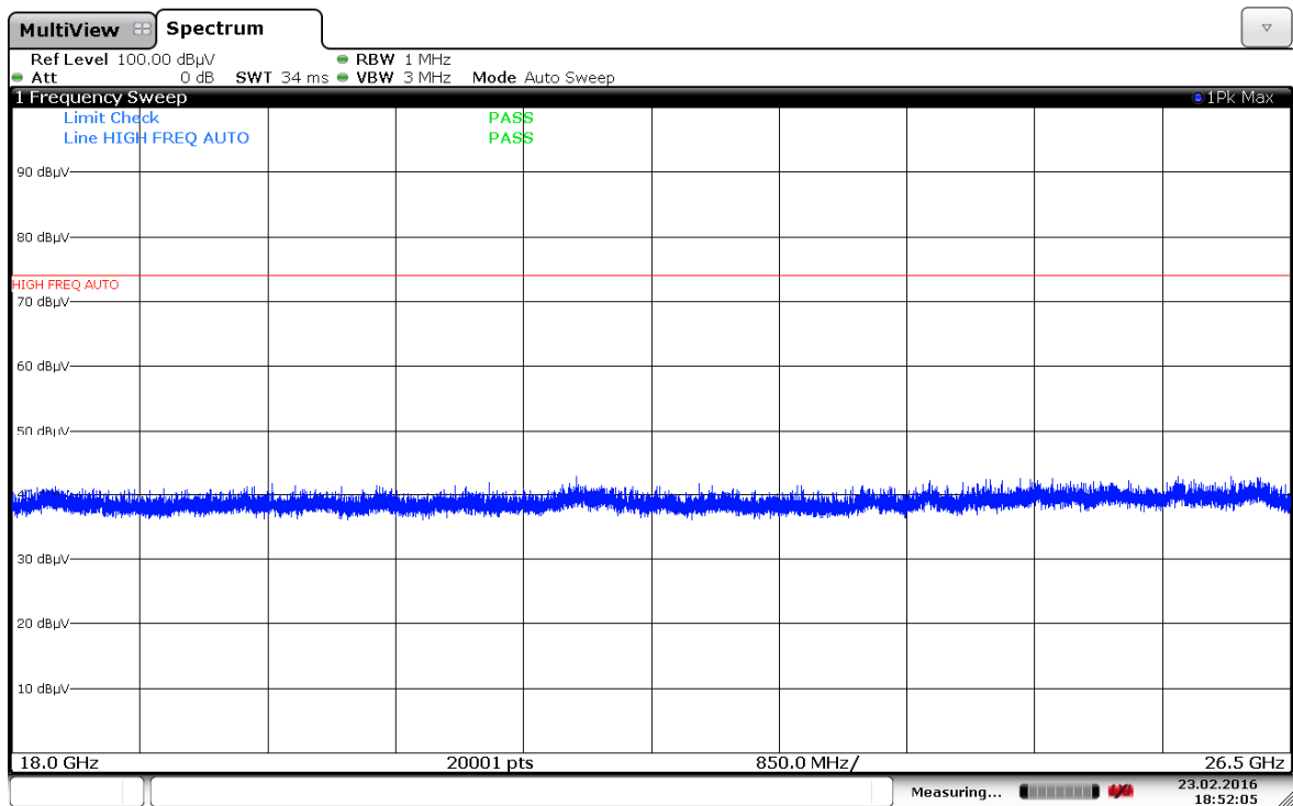
Plot 7-195. Radiated Spurious Plot > 18GHz (LAA (UNII Band 3, 40MHz BW), Ch. 53140, 53340)
