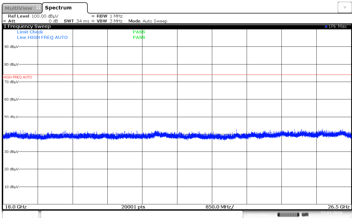
Plot 7-179. Radiated Spurious Plot > 18GHz (LAA (UNII Band 3, 20MHz BW), Ch. 53140)
