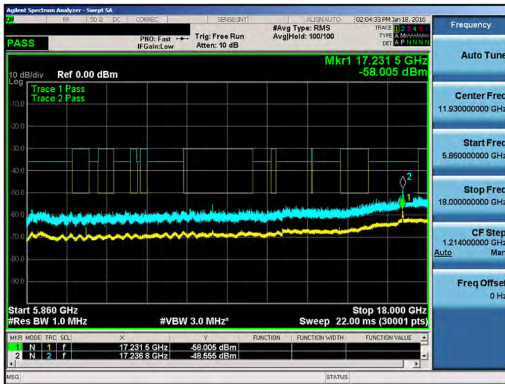
Plot 7-145. Conducted Spurious Plot (LAA (UNII Band 3, 20MHz BW) – Ch. 52740)
