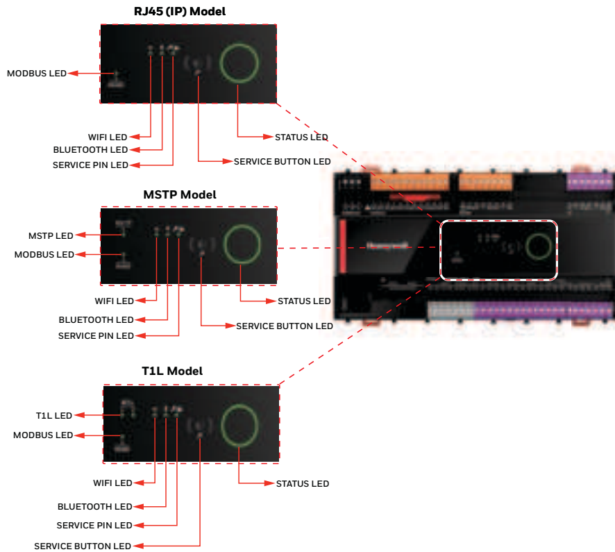
Figure 19. LED interface
