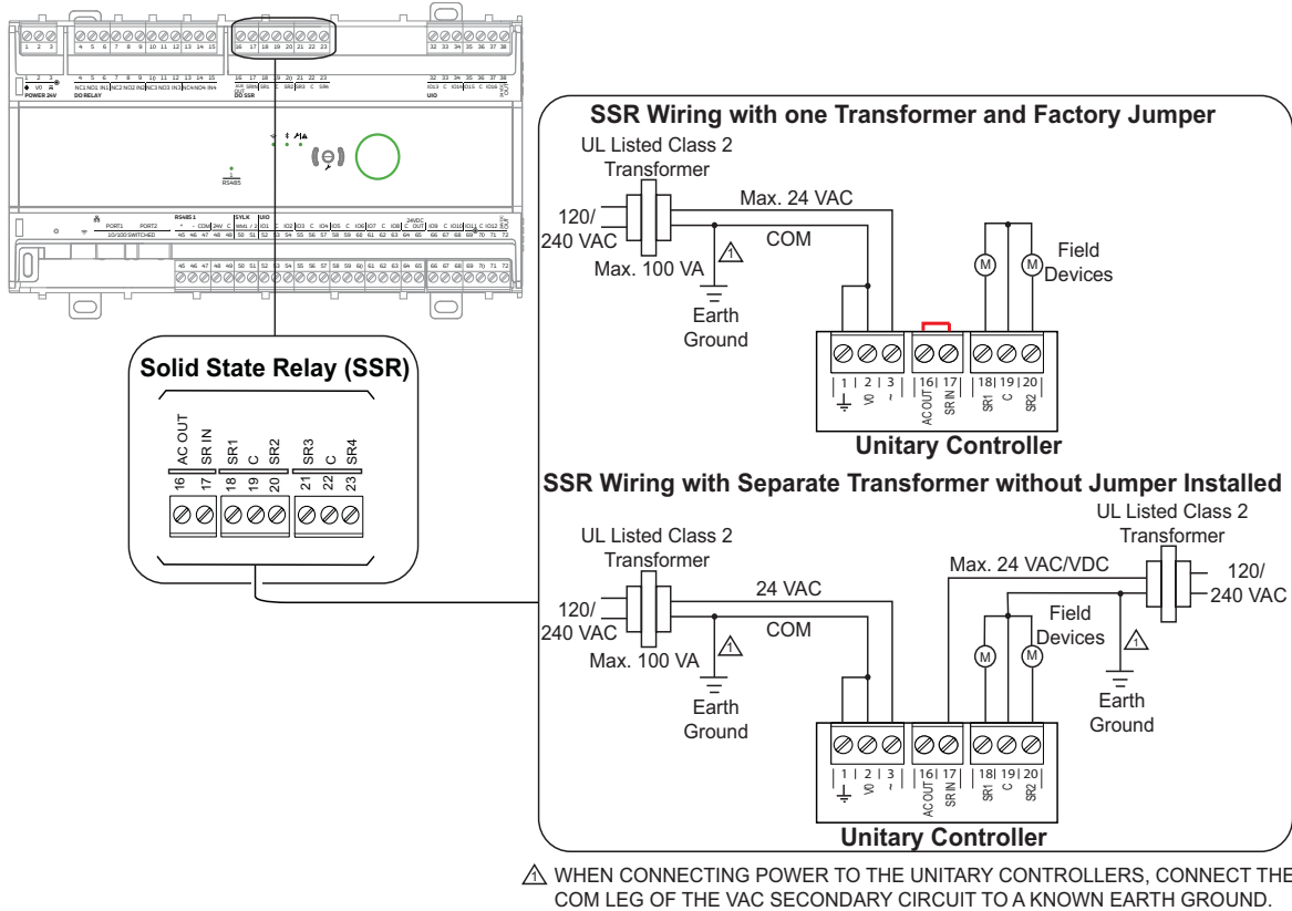
Figure 5. SSR Wiring
