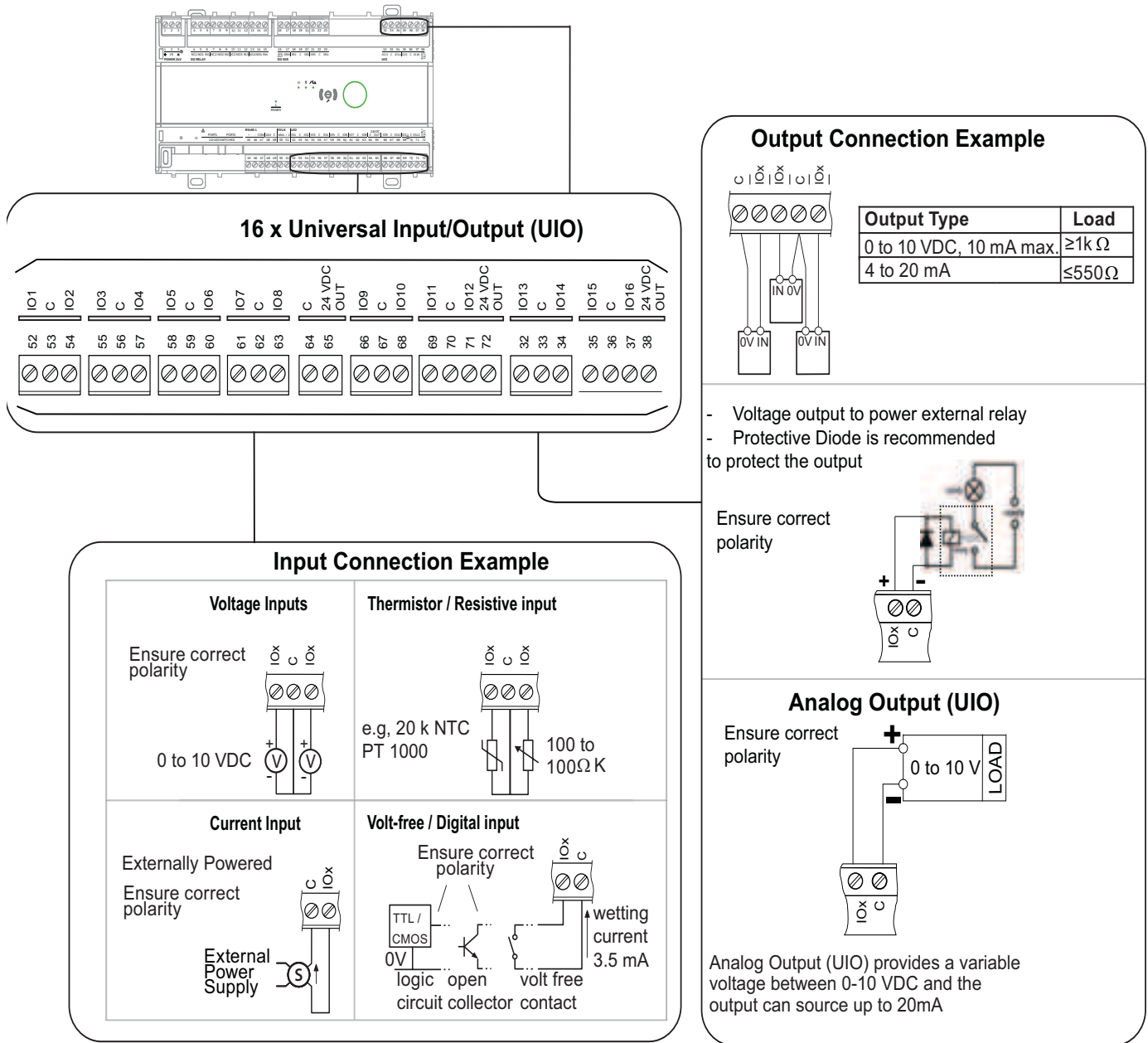
Figure 3. Universal IO Wring
