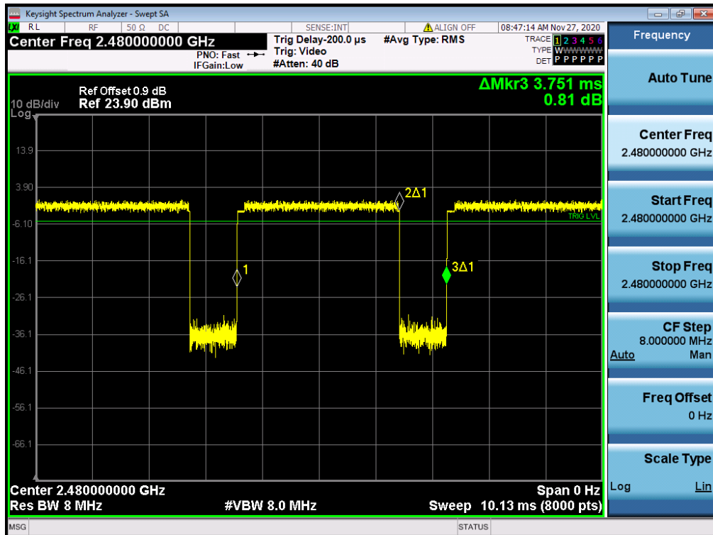
3DH5_Ant1_2480
