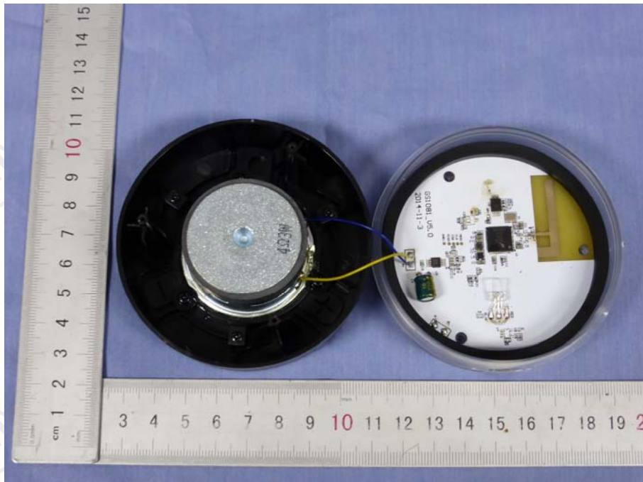
Fig.2- Inner View
