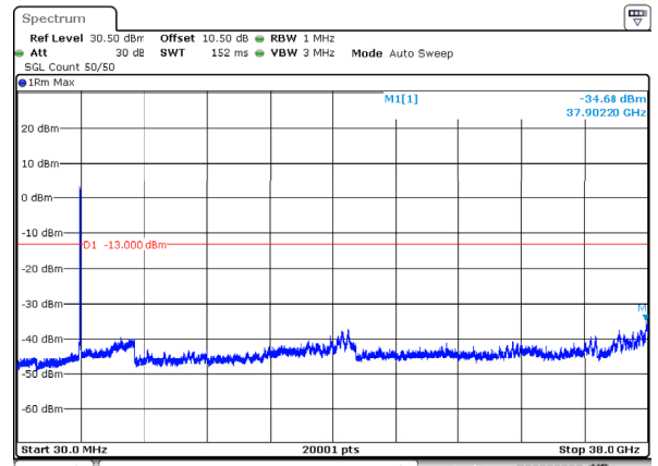
n78_3_40MHz_30kHz_3750MHz_DFT-s-OFDM QPSK_RB100@0 -34.68dBm
