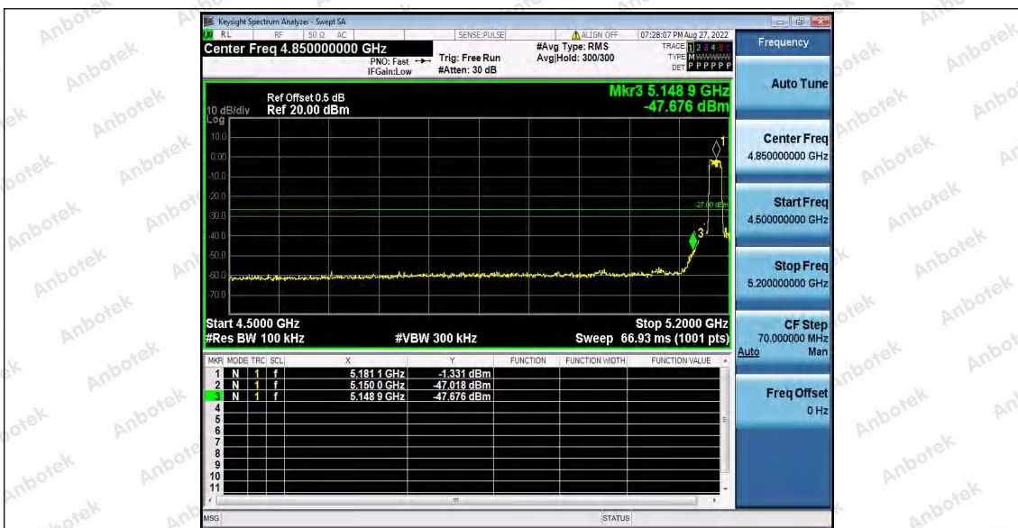
11AC20SISO_Ant2_Low_5180
