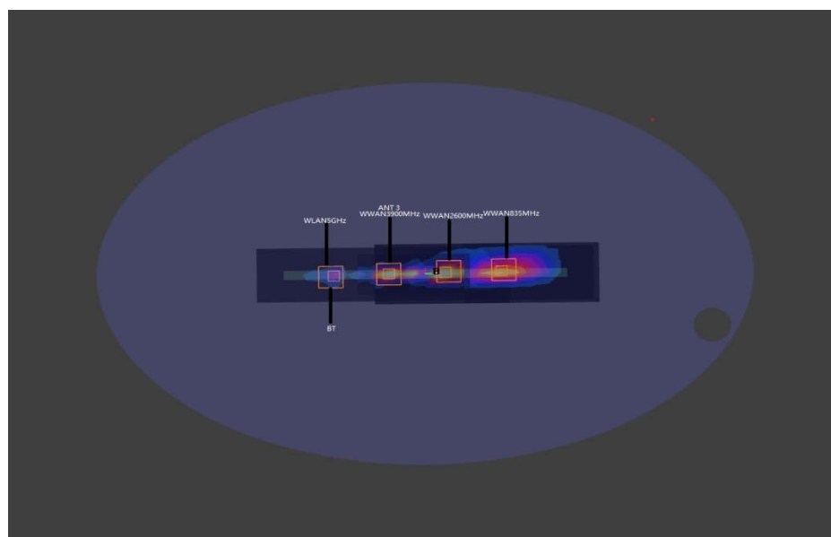
WWAN(ENDC)+WLAN5GHz+Bluetooth_Edge1 0mm
