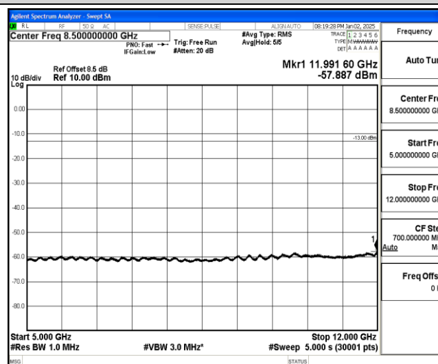
Band25-5MHz-QPSK-26365-1-0-Low-5000-12000--57.89-PASS
