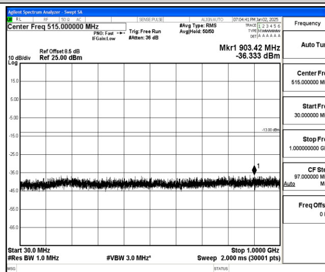
Band25-1.4MHz-16QAM-26047-1-0-Low-30-1000--36.33-PASS
