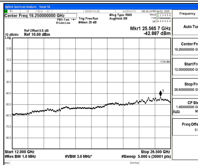
Band25-5MHz-QPSK-26065-1-0-Low-12000-26500--42.89-PASS
