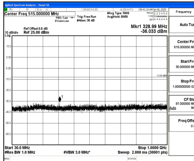
Band25-1.4MHz-16QAM-26365-1-0-Low-30-1000--36.03-PASS
