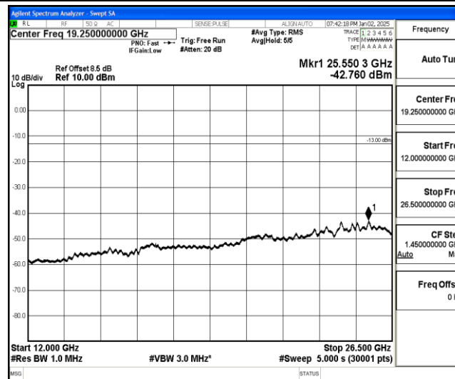
Band25-3MHz-QPSK-26365-1-0-Low-12000-26500--42.76-PASS
