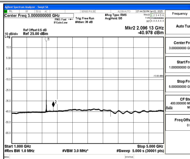
Band25-3MHz-QPSK-26675-1-0-High-1000-5000--40.98-PASS
