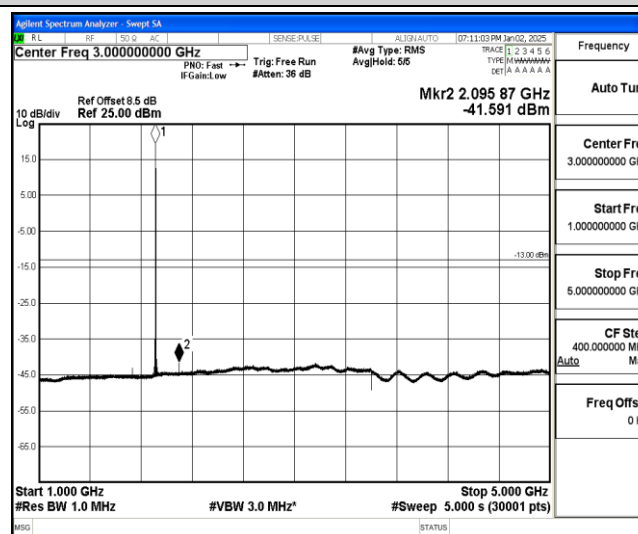
Band25-1.4MHz-QPSK-26683-1-0-High-1000-5000--41.59-PASS
