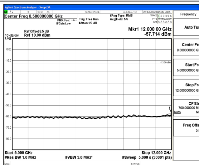
Band25-1.4MHz-16QAM-26365-1-0-Low-5000-12000--57.71-PASS
