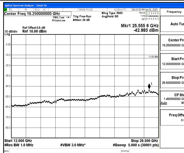
Band25-5MHz-QPSK-26665-1-0-High-12000-26500--42.88-PASS
